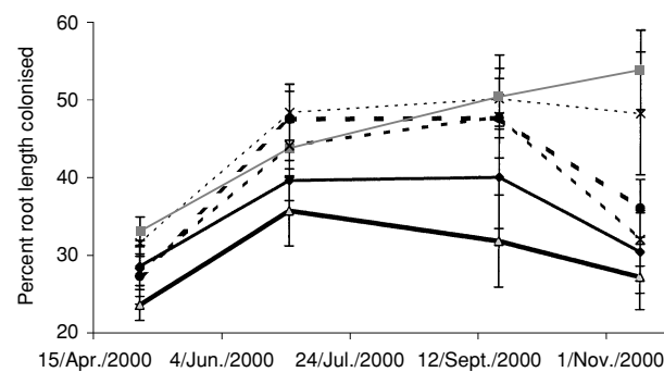
Fig. 3 Root length colonised (RLC) (percent) by arbuscular mycorrhizal fungi as affected by climatic manipulations. Treatments are: control (—●—), summer drought (—■—), summer water addition (—▲—), winter warming (—■—), warming and drought (—●—), warming and water addition (—■—); error bars represent standard errors.
