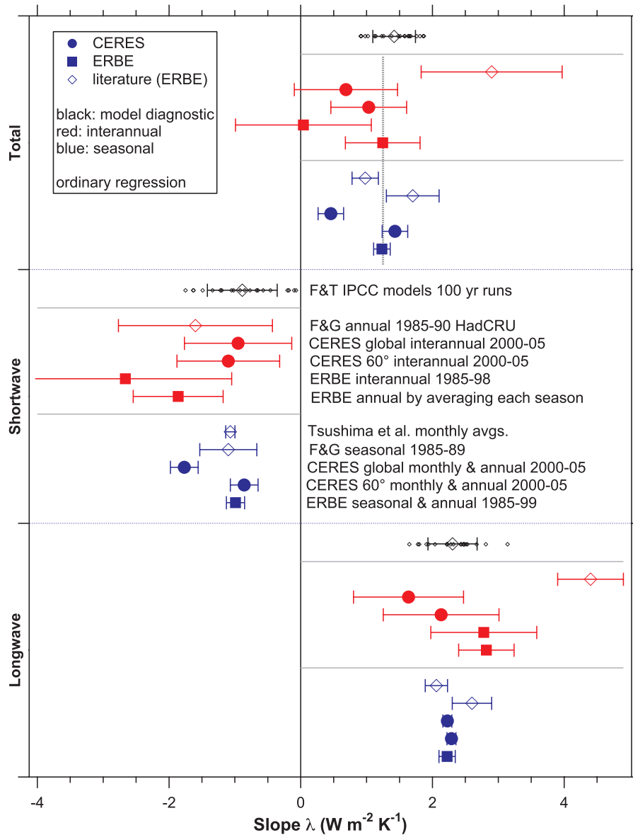
Figure 3. Summary of various calculations of \lambda for longwave, shortwave, and total radiation. The bottom two solid points in each category are the slopes from Figure 2. The next point up is a similar analysis for global CERES data rather than 60^{\circ}\text{S} – 60^{\circ}\text{N} . It shows a nearly identical longwave response but a much stronger shortwave response from snow in the polar regions. The open blue points are literature values including seasonal variation [Tsushima et al., 2005; Forster and Gregory, 2006]. The solid red points are slopes of interannual data for ERBE and CERES data (Appendix A). The open red point is a literature value for a subset of the ERBE data [Forster and Gregory, 2006]. The open black points are regressions of outgoing radiation minus forcing against temperature for 20 models in the IPCC archive [Forster and Taylor, 2006]. Values plotted here are ordinary regression; see Table 1 for the slopes of orthogonal distance regressions. The dotted vertical line in the total section is the value used in this paper.
