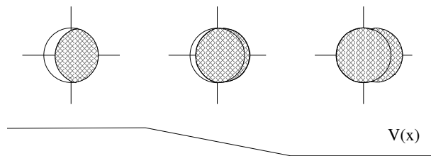
FIG. 1: Semi-classical interpretation of a finite-field potential V(x) applied to a wire. The local Fermi spheres are depicted as for 2D gas for clarity. The filled area on top of the equilibrium spheres indicates accelerated electrons, while the empty area inside the equilibrium spheres represents states emptied by the decelerating effect of the uphill field.
