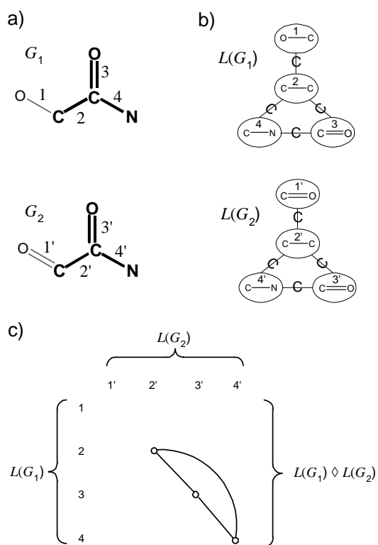
Figure 6. Modular Product of Line Graphs
