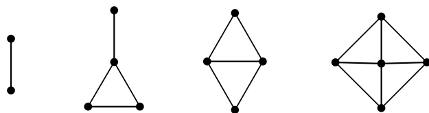
Figure 12. Forbidden Subgraphs for Line Graph Automorphism
