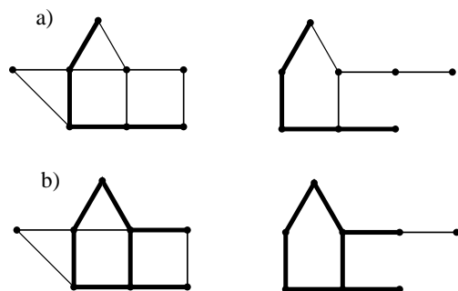
Figure 1. a) Maximum Common Subgraph b) Maximum Common Edge Subgraph
