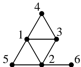
Figure 8. Undirected Graph G
