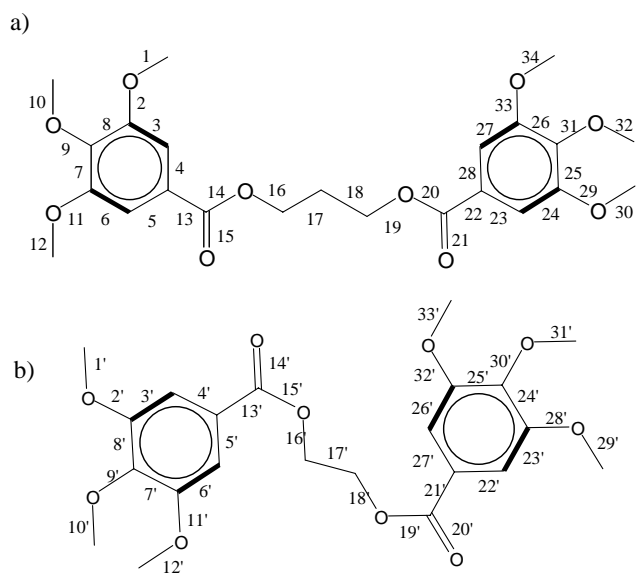
Figure 11. Symmetrical Molecular Graphs
