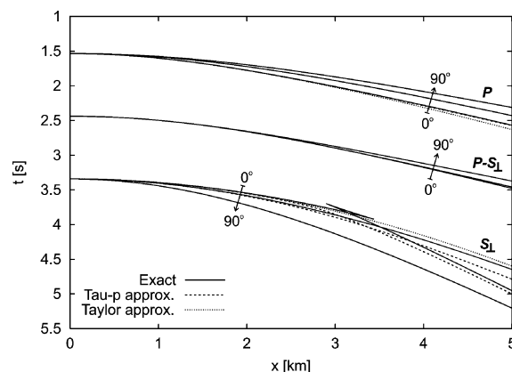
FIG. 7. Traveltimes for reflections from the bottom of the second HTI layer for P, S_{\perp} , and P-S_{\perp} converted waves. Traveltimes are computed for constant azimuthal phase angles of 0^{\circ} , 45^{\circ} , and 90^{\circ} . Solid line: exact curves; long dashes: \tau - p approximations; short dashes: Taylor-series approximations (along symmetry axis only).
