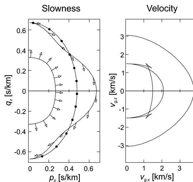
FIG. 4. Phase-slowness (left) and group-velocity (right) surfaces of the anisotropic shale described in Table 2. The velocity sheets are axisymmetric around the vertical axis.
