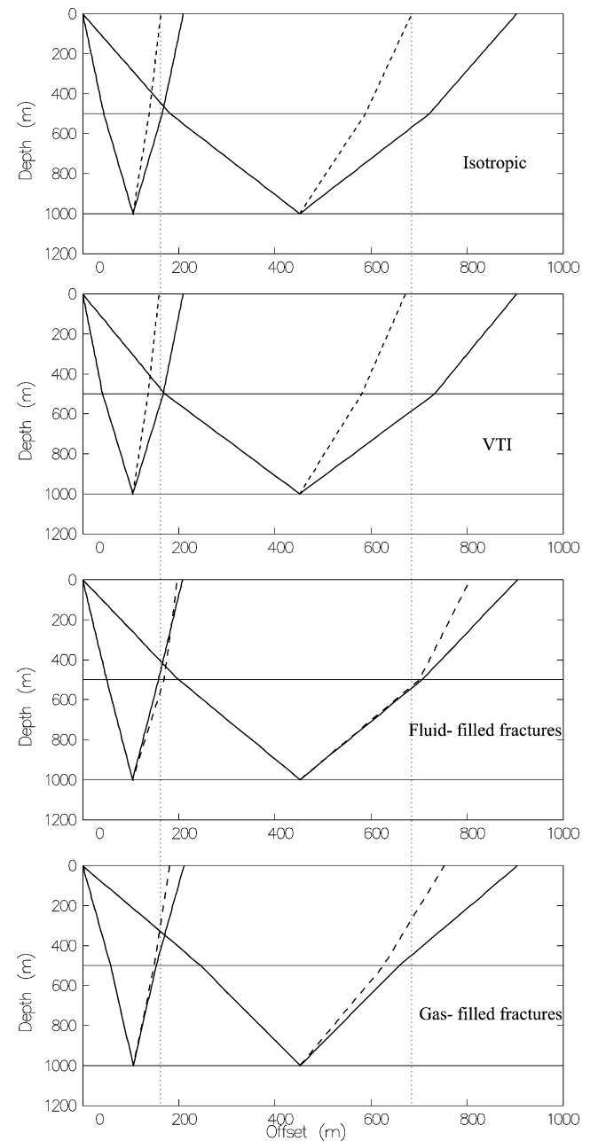
FIG. 3. Raypaths for P-waves (solid lines) and SV-waves (dashed lines) in the four models. From top to bottom, the properties of the second layer are: isotropic, elliptical VTI symmetry, fluid-filled fractures, gas-filled fractures.
