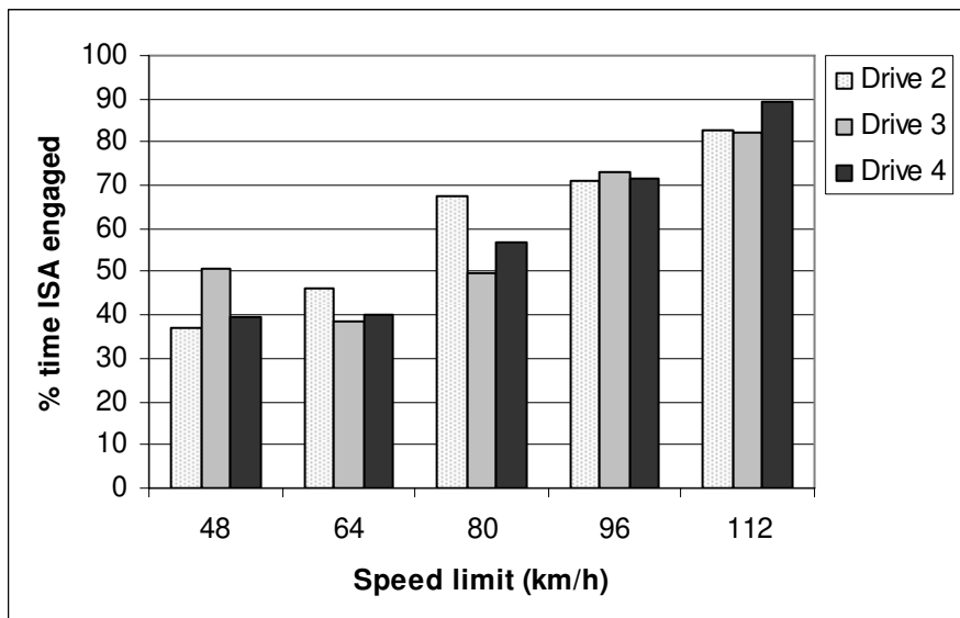
Fig 2. Use of the voluntary ISA system (simulator study)
