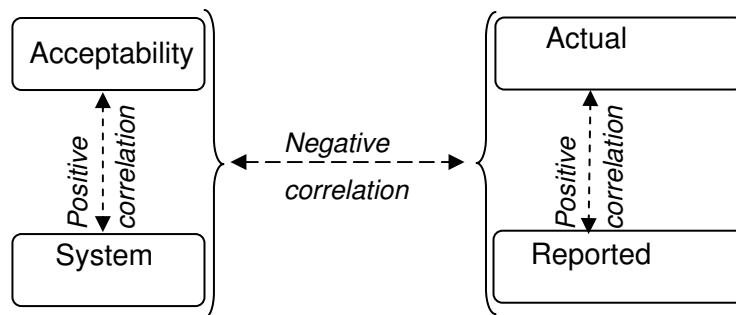
Fig 1. Hypothetical relationship between measured variables
