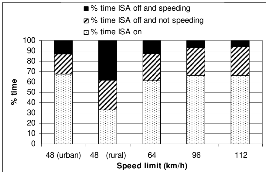
Fig 6. Use of the voluntary ISA system and speed choice (on-road study)
