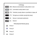
F5. Lithologic and petrophysical group key, p. 13.
