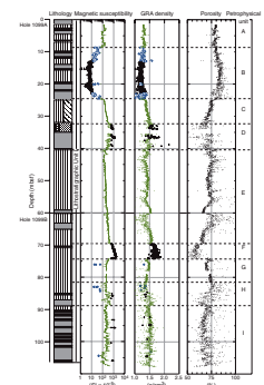
F4. Lithology, magnetic susceptibility, and GRA density, Holes 1099A and 1099B, p. 12.
