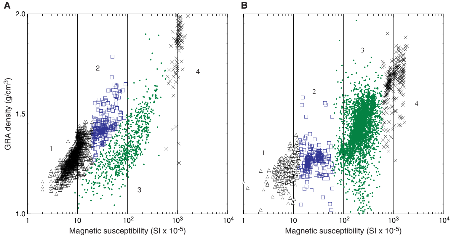
Figure F7. Gamma ray attenuation (GRA) density vs. magnetic susceptibility for (A) Hole 1098C and (B) Holes 1099A and 1099B. Data with a density <1 g/cm 3 have been removed from the plots.
