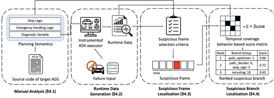
Fig. 3. Overview of our approach.
