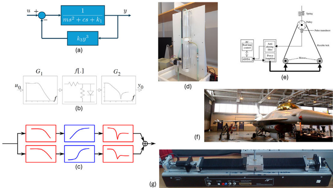
Figure 2. Overview of the considered benchmark systems: (a) Silverbox, (b) Wiener–Hammerstein, (c) Parallel Wiener–Hammerstein, (d) Cascaded Tanks, (e) Coupled Electric Drives, (f) F-16 Ground Vibration Test, and (g) Electro-Mechanical Positioning System.
