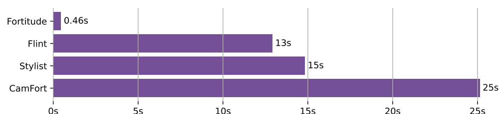
Figure 1: Time taken for Fortran linters to lint 72 files in the GS2 project.
