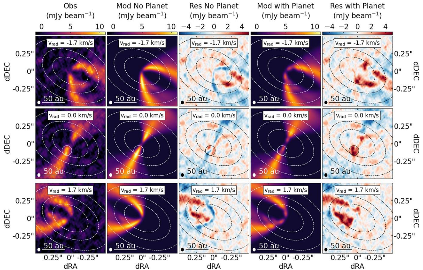
Figure 7. Select channels from the ^{12}\text{CO} ( J = 3-2 ) data cube of the observations (first column), the models shown in Figure 6 (second and fourth columns), and the residuals of the observations minus the models (third and fifth columns). The dashed ellipses in every panel show the location of the three continuum rings derived from our continuum observation analysis. Some key features of the observations are reproduced well in the models, namely, the backside of the disk being visible. Additionally, both sides of the disk dim in roughly the same place as in the observations due to continuum subtraction from the bright continuum rings (see, e.g., the dark lanes in CO coincident with the location of B69). In the model shown with planets, red residuals tend to follow the B43 ring since this model overpredicts its brightness and thus subtracts too much continuum. The residuals in both models show that the observations are brighter in the inner disk, while the models are brighter in the outer disk. The zero velocity channel shows a small S-shaped kink that is marked by a circle in the middle row and shows up as dark red spots in the residual maps. CO photodissociation is included in both of the models shown.
