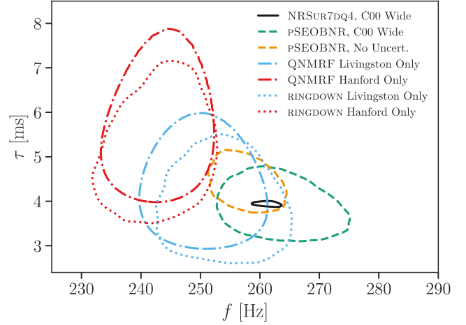
FIG. 4. Inferred (2,2,0) QNM frequency and damping time from analyses of GW250207. The full IMR GR result, incorporating a wide prior for Hanford calibration, is indicated by the solid line. The pSEOBNR analysis (dashed) compares results obtained by either neglecting calibration uncertainties (yellow) or incorporating a wide prior for Hanford to marginalize over them (green). The QNMRF (dot-dashed) and ringdown (dotted) analyses analyze Hanford (red) and Livingston (light blue) data separately without calibration uncertainty to assess potential systematic errors. QNMRF and RINGDOWN analyze the signal starting at 8t_{M_f} after the peak of the strain, where time is in units of the remnant mass in the detector frame (the maximum-likelihood estimate from the IMR analysis using the NRSUR7DQ4 waveform [193] and the wide calibration prior).
