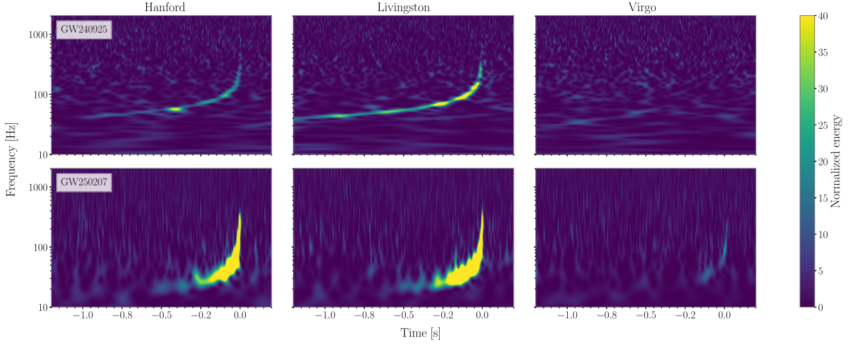
FIG. 1. Time–frequency spectrograms [98] showing data from LIGO Hanford (left), LIGO Livingston (middle), and Virgo (right) for GW240925 (top) and GW250207 (bottom). Times are relative to the times reported from the search algorithms for the two detections. We use C00 LIGO data. The data are whitened [13], and the scale bar shows the normalized energy.
