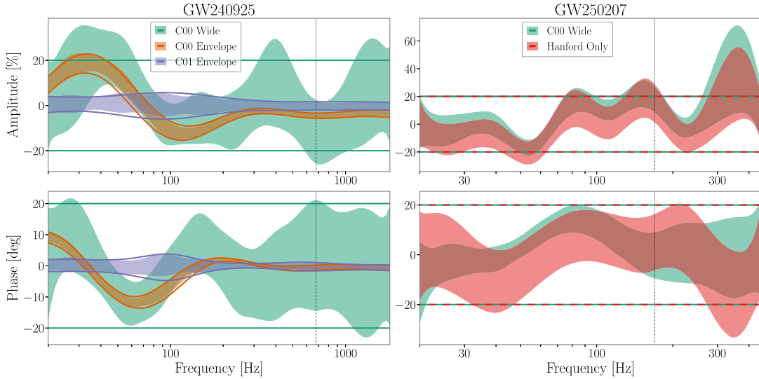
FIG. 2. LIGO Hanford calibration as a function of frequency over the analysis band for each signal. The top and bottom panels show the frequency-dependent amplitude error \delta A and phase error \delta \phi , respectively. Shaded regions indicate the 68% credible intervals of the posteriors, and the lines denote the 68% probability envelopes from which the priors are derived (see Supplemental Material [36]). GW240925 results (left) are from three analyses: one using a wide, uninformative prior on the miscalibrated C00 data (green), one using a narrow prior envelope based upon in situ measurements on the same data (orange), and one using a narrow in situ measured prior envelope for the recalibrated C01 data (purple). GW250207 results (right) are from two analyses, both using the same wide priors on the miscalibrated Hanford C00 data: one using data from all three detectors (green), with the in situ priors applied to Livingston and Virgo data, and one using only Hanford data (red). Results are more informative for frequencies where there is more signal power (Fig. 1), and the dotted vertical lines indicate the approximate peak frequencies f_{22}^{\text{peak}} for the \ell = |m| = 2 multipole of the signals.
