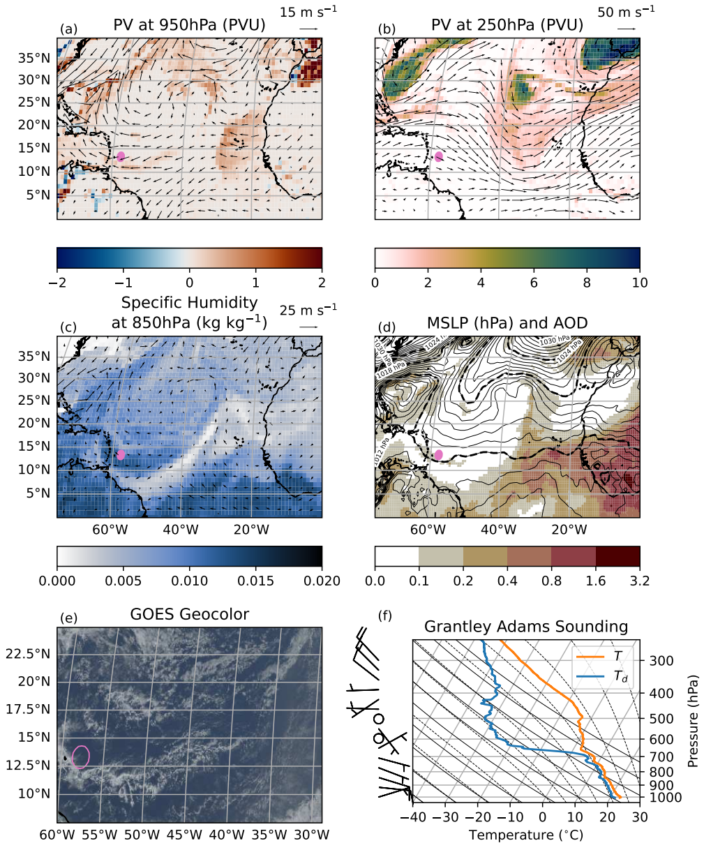
FIGURE 3 Reanalysis and observational data for 22nd January at 18 UTC. (a) ERA5 PV and wind vectors at 950 hPa. (b) ERA5 PV and wind vectors at 250 hPa. (c) ERA5 Specific humidity and wind vectors at 850 hPa. (d) ERA5 Mean-sea-level pressure (contours every 1 hPa and dashed every 6 hPa) and MERRA-2 aerosol optical depth (colours, logarithmic scale). (e) GOES Geocolor composite of visible channels following Miller et al. (2020). (f) Skew-T log-P chart of the sounding from Grantley Adams airport at 12 UTC. The wind barbs are in increments of 10 m s -1 (5 m s -1 for half barbs). The pink circle to the west of Barbados in panels a-e shows main measurement area during the EUREC 4 A field campaign.
