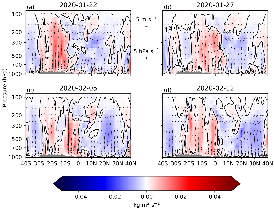
FIGURE 9 Vertical cross sections of the daily mean meridional mass flux (shaded, \text{kg m}^{-2} \text{s}^{-1} ) and the the wind in the plane of the cross section (arrows, \text{m s}^{-1} ) averaged over 60^\circ\text{W} to 40^\circ\text{W} at four times during the EUREC 4 A field campaign period.
