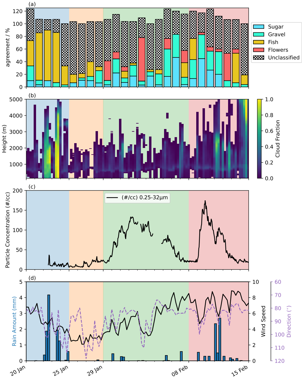
FIGURE 2 Timeseries of observations from Barbados during EUREC 4 A. (a) Daily average cloud pattern at the Barbados cloud observatory reproduced from figure 5a in (Schulz, 2022a). (b) 6-hourly averaged cloud fraction from the cloud radar at BCO. (c) Particle concentration in number per cubic centimetre of aerosol particles in the size range 0.25–32 \mu\text{m} measured by the GRIMM OPC. (d) 6-hourly accumulated rain, and 6-hourly averaged wind speed and direction observed at BCO. The wind direction is degrees from North (i.e. 90° is an easterly wind). The background colours show the four subjectively identified time periods.
