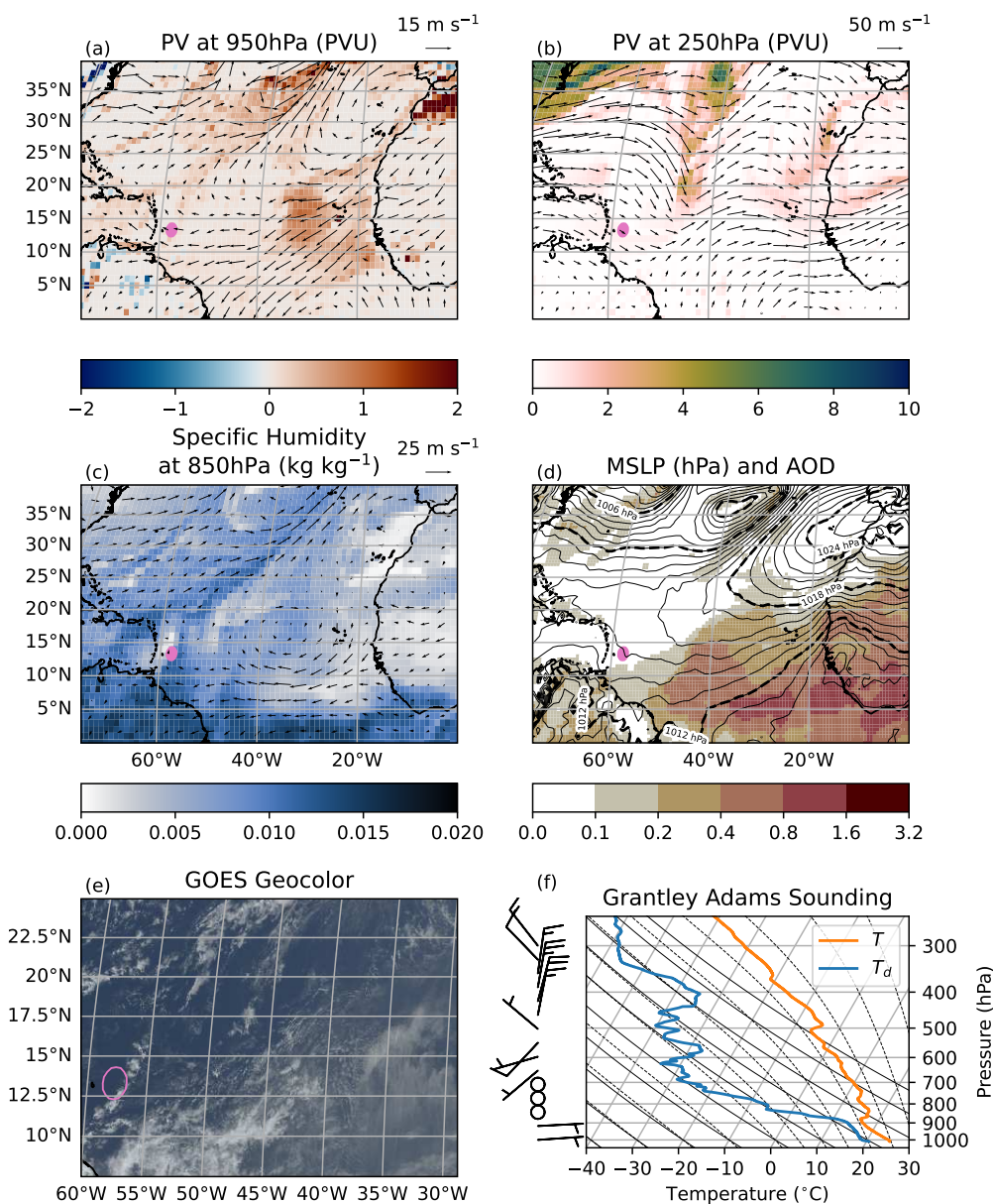
FIGURE 4 Same as Fig. 3 but for 27th January.
