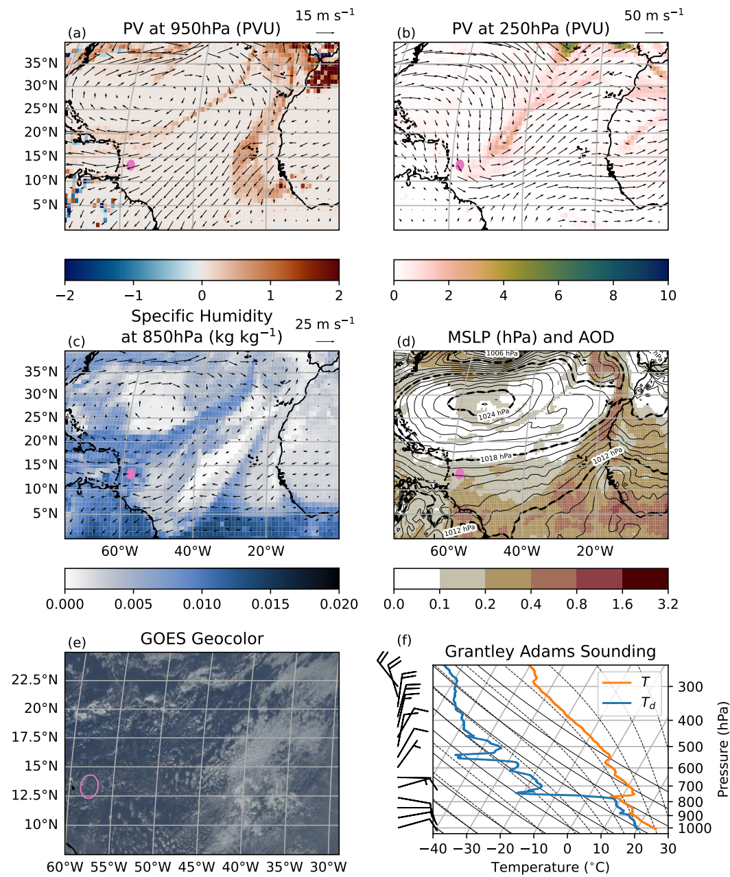
FIGURE 5 Same as Fig. 3 but for 5th February.
