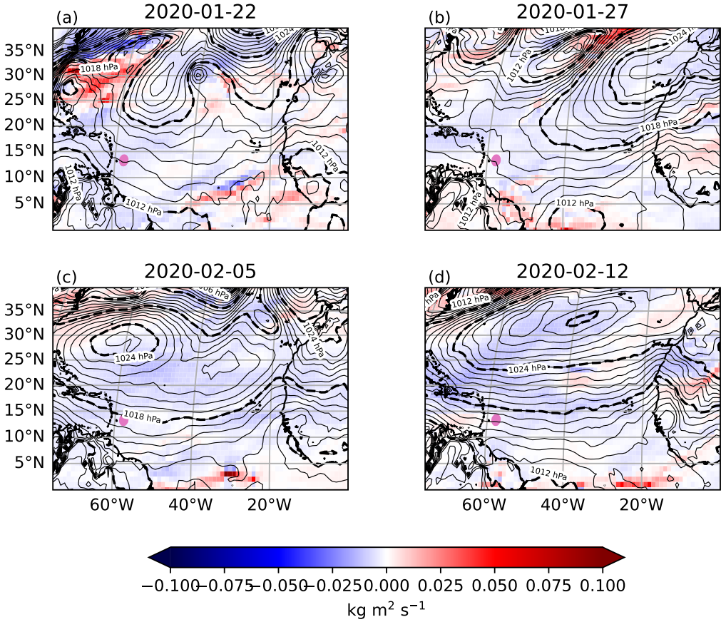
FIGURE 8 The daily mean meridional mass flux at 500 hPa (shaded, \text{kg m}^{-2} \text{s}^{-1} ) and MSLP (contours, hPa) at four times during the EUREC 4 A field campaign period.
