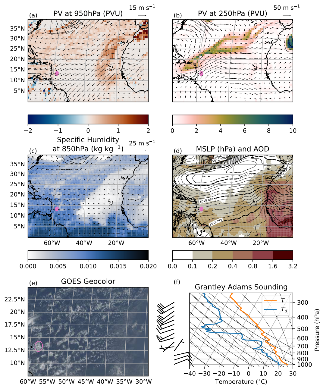
FIGURE 6 Same as Fig. 3 but for 12th February.
