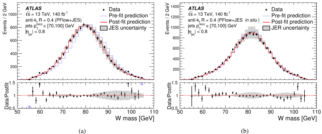
Fig. 9 The pre-fit (dotted line) and post-fit (solid line) predictions for the W -boson mass distribution in the diagonal region with reconstructed jet p_T between 70 and 100 GeV in the a JES and b JER fit to the Run 2 data. The hatched uncertainty band is estimated by propagating the total uncertainty in the a JES or b JER to the bin yield predictions. The predictions are normalised to the same total yield as data. The bottom
