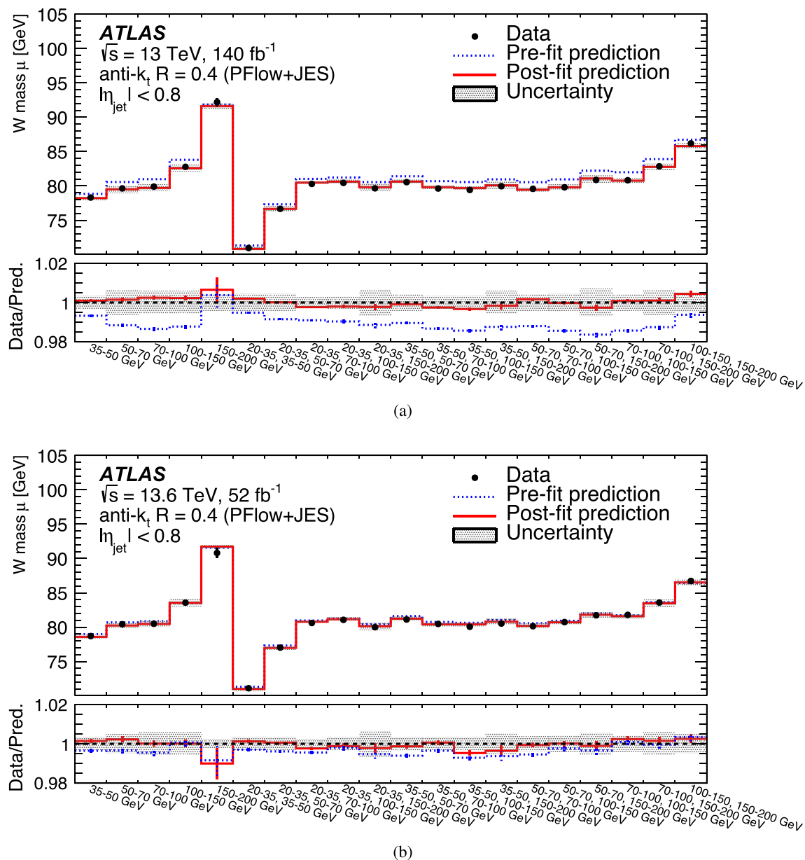
Fig. 6 Mean of the W mass distributions shown for the analysis regions defined in Sect. 5 in the JES fit in the a Run 2 and b Run 3 measurement. The values obtained in data are compared with those in simulations before and after the forward-folding correction. The uncertainties are obtained from pseudo-experiments taking into account the statistical and systematic uncertainties. The non-forward-folded (pre-
