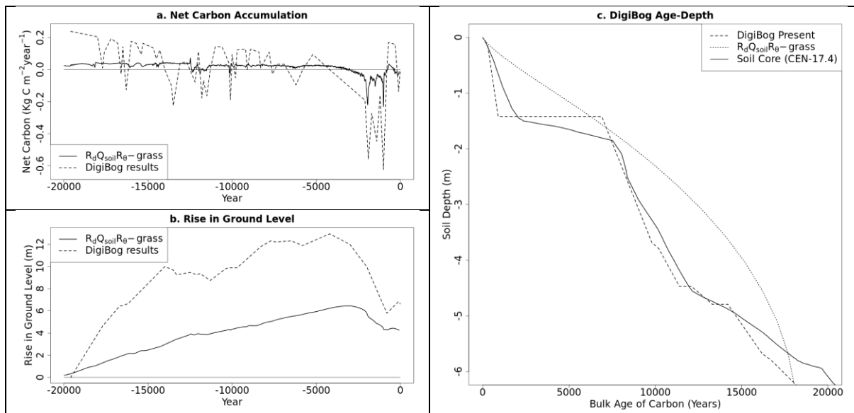
Figure 6: comparing the results from the final JULES-Peat simulation to DigiBog: (a) net carbon accumulation, (b) rise in ground level, and (c) age-depth profiles compared to the CEN-17.4 core.
