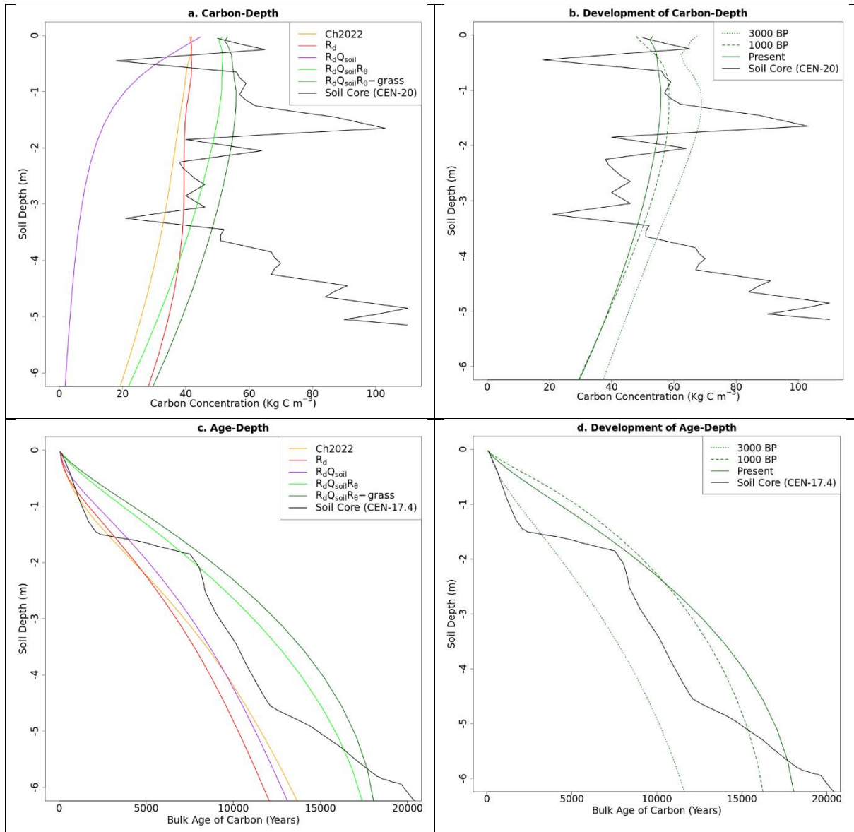
Figure 6: (a) carbon concentration profiles from JULES-Peat at the end of all five simulations compared to the measurements obtained from the CEN-20 core; (b) carbon concentration profiles at 3,000 BP (greatest depth of peat), 1,000 BP (following large loss of peat) and the end of the final simulation (times marked by diamonds on Figures 2i-j) compared to CEN-20; (c) carbon bulk age profiles from JULES-Peat at the end of all five simulations, with radiocarbon dates obtained from the CEN-17.4 core; (d) development of the carbon bulk age profile in the final simulation with CEN-17.4
