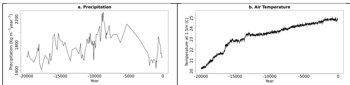
Figure 2: Palaeoclimate history in the Central Congo Basin. (a) precipitation reconstructed from isotopes in the CEN-17.4 peat core; (b) air temperature at 1.5m above the surface, simulated by the HadCM3 climate model.
