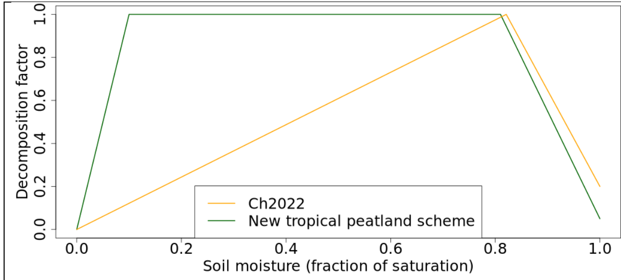
Figure 3: Old and new decomposition functions relating soil respiration to soil saturation in JULES-Peat.
