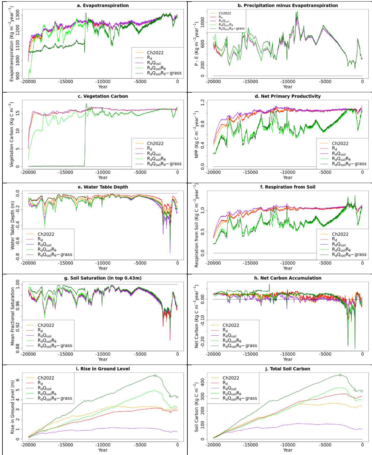
Figure 5: Evolution of the Central Congo Basin peatlands in the five simulations, the variants of the JULES-Peat model (Table 1): (a) evapotranspiration; (b) precipitation – evapotranspiration ( P-E ); (c) carbon in vegetation; (d) net primary productivity ; (e) water table depth, (f) respiration from soil, (g) fractional soil saturation (top 0.43m), (h) net annual increase in soil carbon, (i) rise in the ground level and (j) total carbon in the soil. The diamonds mark 3,000 BP (when there was the greatest depth of peat), 1,000 BP (following the large loss of peat) and the end of the simulation, and the profiles from these times are shown in Figure 6.
