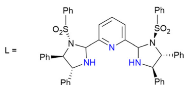
Scheme 1 Structures of calculated transition states and intermediates. Ligand field calculations were performed on the coordinating atoms and the atoms highlighted in blue.
