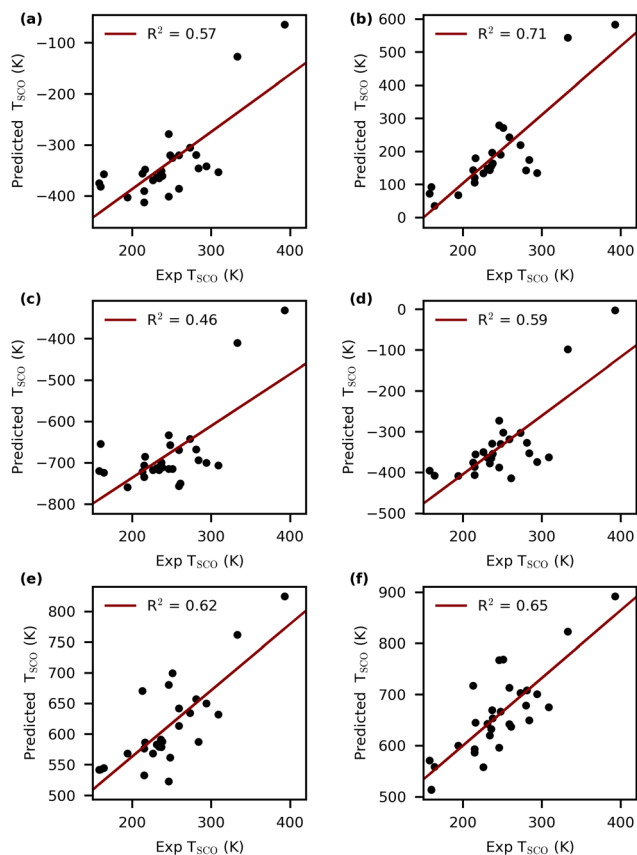
Fig. 6 Plots of predicted vs. experimental T_{\text{SCO}} values for T_{\text{SCO\_dataset}} without the three outliers: (a) B3LYP/def2-TZVP; (b) M06-L/def2-TZVP; (c) PBE0/def2-TZVP; (d) PBE0-D4/def2-TZVP; (e) TPSSH/def2-TZVP; and (f) r^2\text{SCAN} /def2-TZVP.
