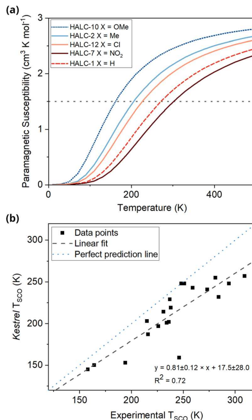
Fig. 3 (a) Susceptibility vs. temperature plots for selected [bis-{bis-(X-pyrazolyl)-Y-pyridine}Fe(II)] PBE0/def2-TZVP optimised structures using the fixed ligand field parameters; the midpoint, T_{1/2} , used to extract T_{\text{SCO}} , is shown by the dashed line; (b) plot of Kestrel calculated vs. experimental T_{\text{SCO}} ( n = 20 , R^2 = 0.72 , \sigma^2 = 0.18 ).
