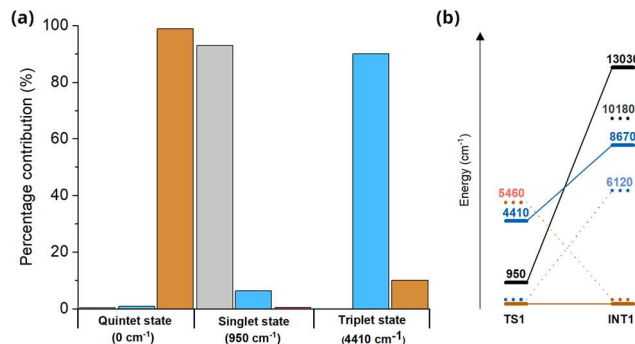
Fig. 9 (a) Configurational mixing of lowest energy quintet (left), singlet (middle) and triplet state (right). Singlet (grey), triplet (blue) and quintet (orange) configuration contributions to each state are shown. (b) Energy profile of literature DFT calculated spin-state energies (dashed lines) and Kestrel calculated spin state energies (solid lines) for the singlet (black), triplet (blue) and quintet (orange) states for TS1 and INT1 .
