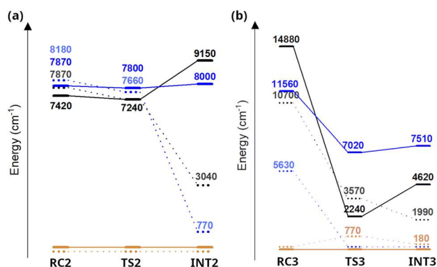
Fig. 10 (a) Energy profile of DFT calculated spin-state energies (dashed lines) and Kestrel calculated spin state energies (solid lines) for path I; (b) energy profile of DFT calculated spin-state energies (dashed lines) and Kestrel calculated spin state energies (solid lines) for path II. Energies are shown for doublet (black), quartet (blue) and sextet (orange) states.
