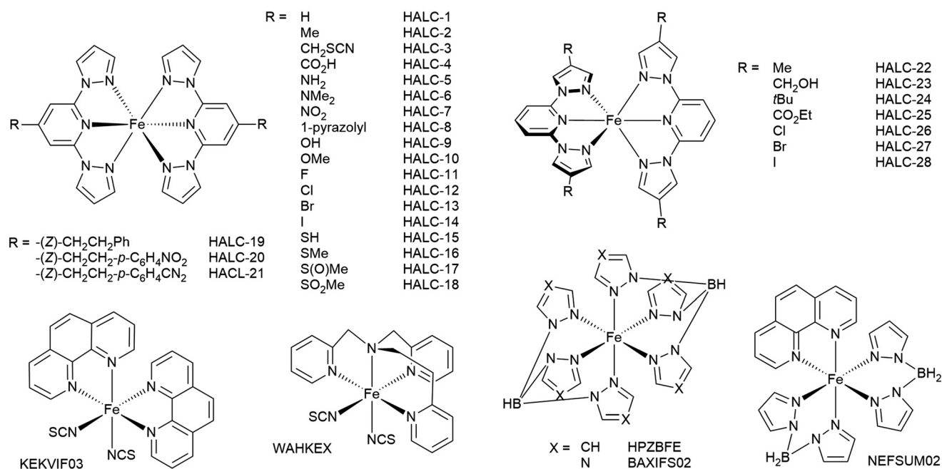
Fig. 2 Chemical structures of complexes in T_SCO_dataset .
