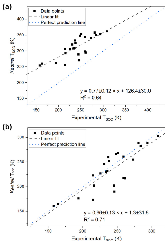
Fig. 8 (a) Experimental vs. Kestrel-calculated T_{\text{SCO}} using PBE0-D4 optimised geometries ( n = 24 , R^2 = 0.64 ); (b) experimental Kestrel-calculated T_{\text{SCO}} using PBE0-D4 optimised geometries where e_\sigma values are linked to the Hammett parameters of the substituents ( n = 24 , R^2 = 0.71 ).
