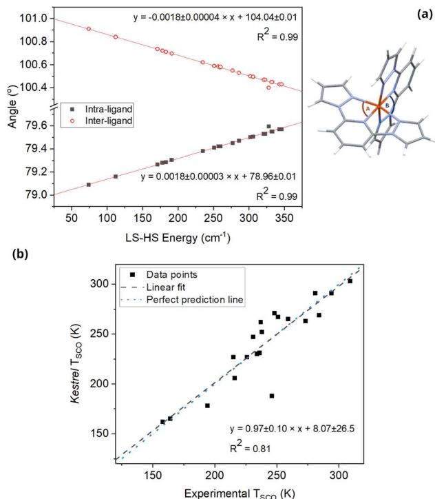
Fig. 7 (a) Variation of angle A (black) and angle B (red, empty) with LS-HS energy using the fixed ligand field parameters (Table 3); (b) experimental vs. ligand field-calculated T_{SCO} , where the ligand field strengths are linked to Hammett parameters of the substituents.
