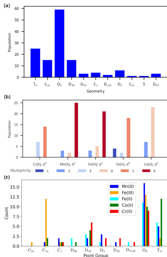
Fig. 1 Analysis of base_spin_dataset , showing the included (a) geometries, (b) metals, their oxidation states and multiplicities (1–6, in different colours); and (c) geometries for different metal centres.
