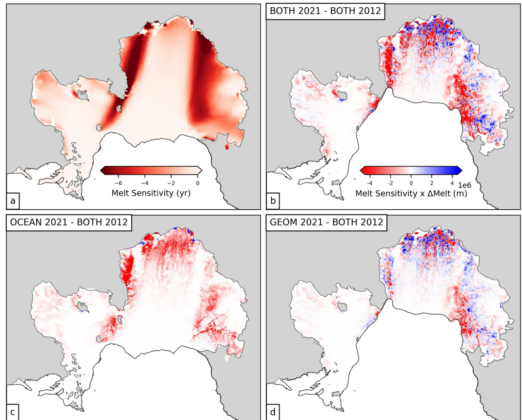
Figure 4. (a) Volume above flotation (VAF) sensitivity to melt from Gourmelen et al. (2025). The units are VAF change ( \text{m}^3 ) per melt rate ( \text{m/yr} ) per area ( \text{m}^2 ). (b–d) are the melt sensitivity multiplied by the difference in melt between the BOTH 2021, OCEAN 2021, and GEOM 2021 with the BOTH 2012 run, respectively.
