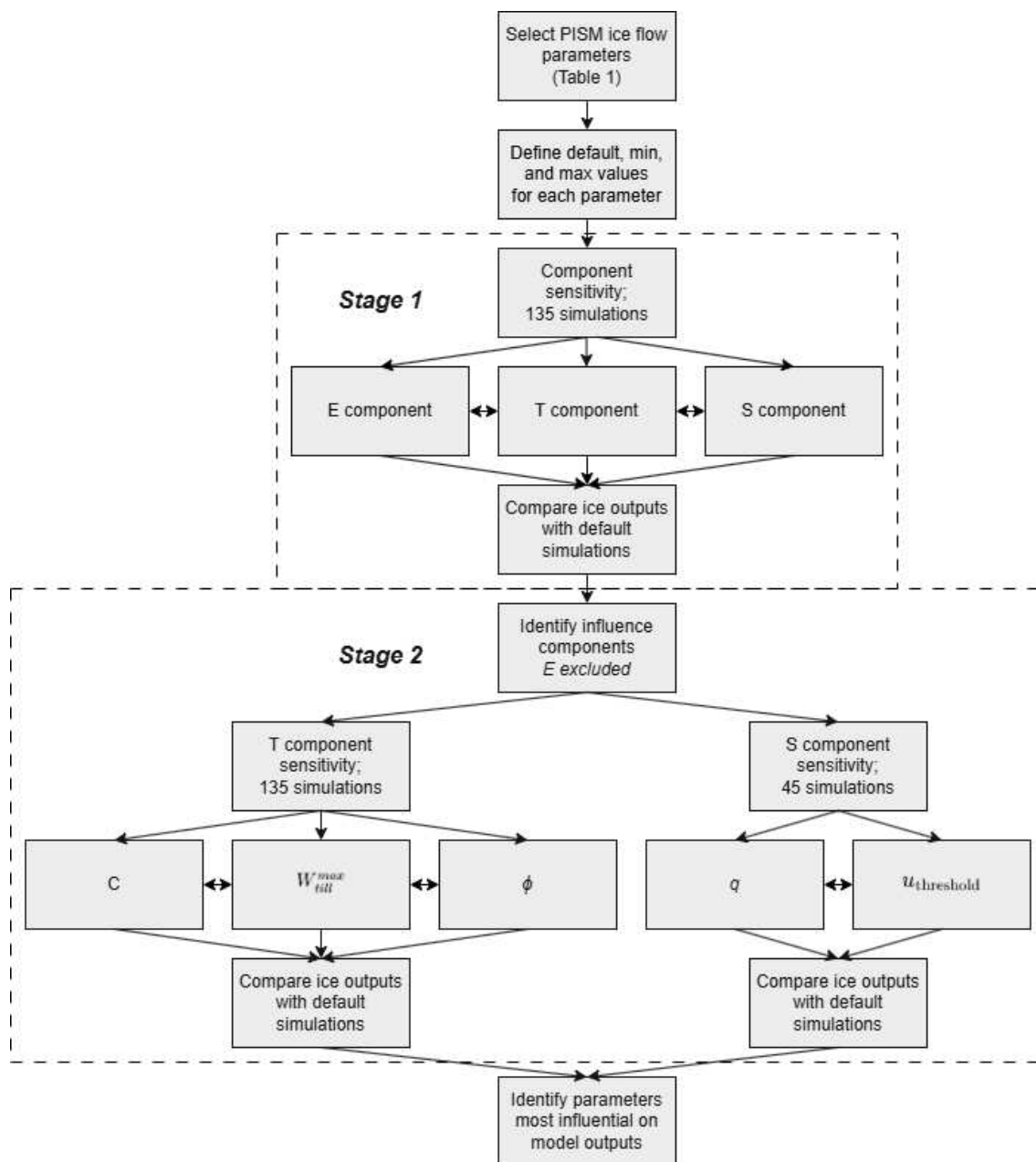
Figure 2. Workflow of the two-stage sensitivity experiment design used here. Stage 1 tests the influence of the chosen model components; the enhancement factors ( E ), till-related parameters ( T ), and sliding parameters ( S ). These use the default, minimum, and maximum parameter values from Table 1. Components with limited influence are excluded from Stage 2. Stage 2 then tests individual parameters within the retained T and S components to identify which parameters exert the most influence on modelled ice volume, thickness, and basal velocity. Simulation numbers are shown for the full five-domain ensemble. These were varied both individually and all together.
