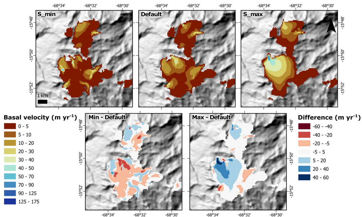
Figure 6. Example of the influence of sliding component parameters on basal ice velocity in the Kaka & Boopi (#3) domain (Ancohuma Ice Caps). Additional examples are provided in the Supplement. Increased parameter values enhance basal velocities, while decreased values reduce them. Variations amplify or suppress sliding patterns already present in the default simulation. “Max” and “min” parameter values are listed in Table 1.
