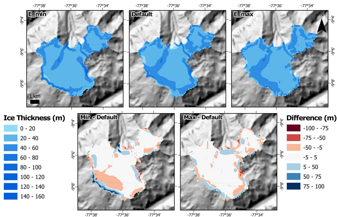
Figure 4. Example of the influence of the enhancement factors on simulated ice thickness in the Santa (#1) domain (Huascarán Ice Cap). Additional examples are provided in the Supplement. Ice peripheral differences in ice thickness are likely to arise from internal variability in the PDD model as mentioned previously in Sect. 3.3. Parameter values for “max” and “min” are listed in Table 1.
