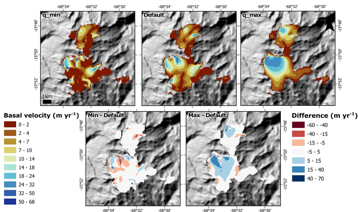
Figure 12. An example of the influence of the sliding exponent ( q ) parameter on the output of ice basal velocity in the Kaka & Boopi (#3) domain (Ancocuma ice caps). Remaining examples are shown in the Supplement. An increase or decrease in the q parameter sees a reorganisation of the velocities fields with more confined velocities when decreased, and more diffuse fields when increased. Values that correspond to “max” and “min” parameter values are found in Table 1.
