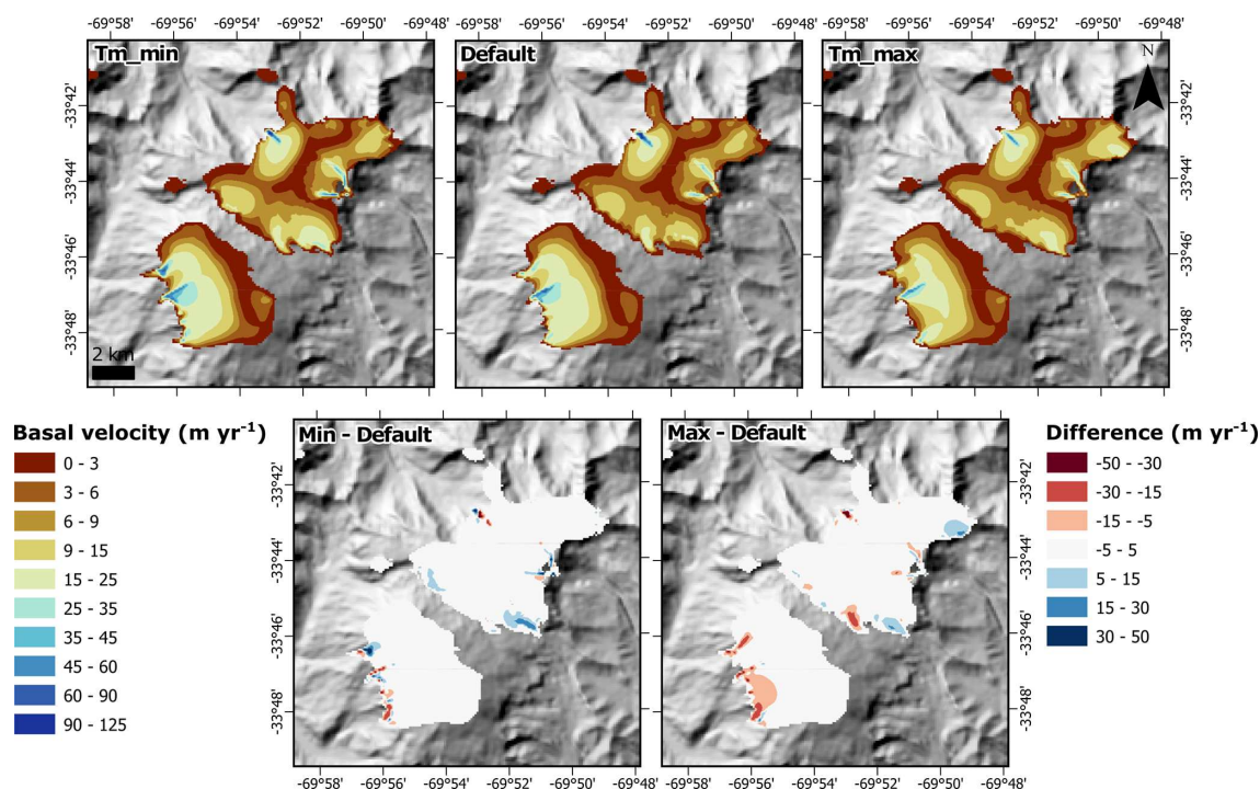
Figure 8. An example of the influence of the W_{\text{till}}^{\text{max}} ( T_m in figure panels) parameter on the output of ice basal velocity in the Mendoza, Maipo, and Rapel (#5) domain (Volcán Marmolejo). Remaining examples are shown in the Supplement. Increased values the T_m parameter generally sees no, or very little changes in basal ice velocities. Values that correspond to “max” and “min” parameter values are found in Table 1.
