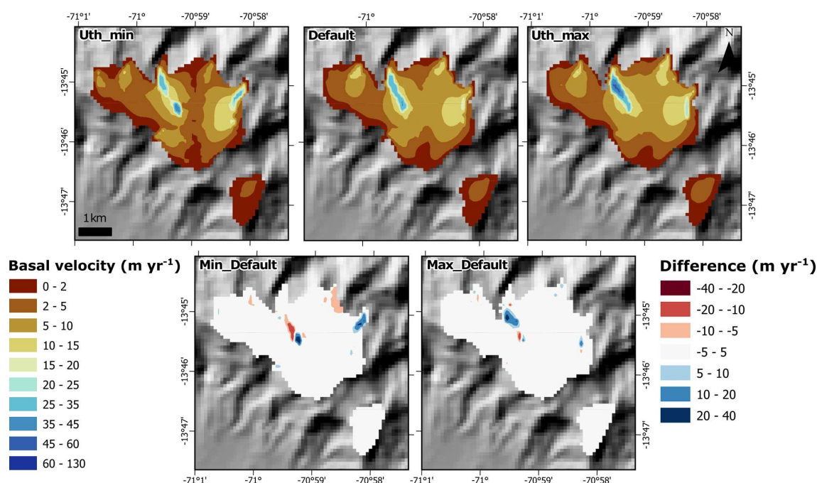
Figure 11. An example of the influence of the u_{\text{threshold}} ( U_{\text{th}} in figure panel) parameter on the output of ice basal velocity in the Vilcanota (#2) domain (Quelccaya Ice Cap). Remaining examples are shown in the Supplement. An increase in the u_{\text{threshold}} parameter sees increased basal velocities, while the opposite is seen when values are decreased. Values that correspond to “max” and “min” parameter values are found in Table 1.
