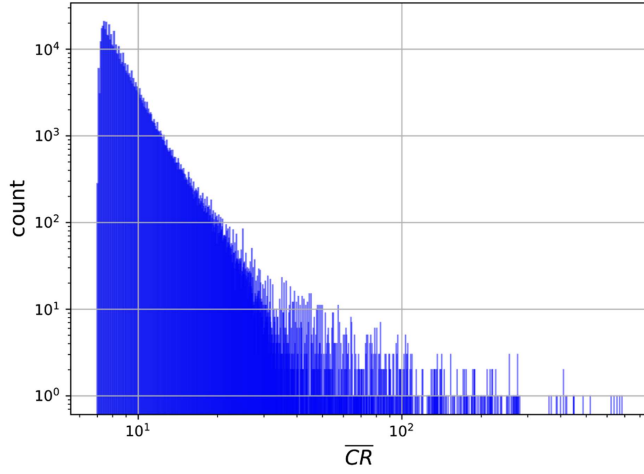
FIG. 5. The critical ratios of coincident candidates returned in our search whose \overline{CR} > CR_{\text{thr}} = 7 . Candidates with CR < CR_{\text{thr}} are not shown. \overline{CR} is averaged from candidates returned in both H1 and L1, and corresponds to the candidates that we followed up, all of which were vetoed. In order to compute upper limits on distance reach, we use these CR s in Eq. (B1) and apply the Feldman-Cousins procedure [66] that effectively increases CR to ensure 95% confidence-level coverage. In other words, real GW signals would have had to generate CR s above the ones in this figure at a given chirp mass, time, and frequency to have been detected by our search 95% of the time.
