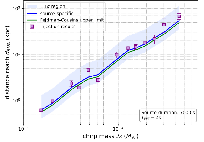
FIG. 6. Comparison of upper limits on distance reach calculated through injections and with the formula given in Eq. (B1). The blue line indicates the theoretical expectation for the distance reach at 95% confidence, adjusted by the source-specific factor \mathcal{C} (see text for details). The shaded region denotes the \pm 1\sigma uncertainty on the distance reach based on the range of source-specific \mathcal{C}_s values. The magenta points indicate the derived distance reach at which 95% of injections are recovered in our simulations. The green line indicates the upper limit that we would actually quote based on the Feldman-Cousins procedure. Our results show that the injection studies agree well with the theoretical blue and green curves and fall well within the shaded region. For each set of 50 injections, at each chirp mass, performed at different distance reaches to derive these results, we analyze different frequency bands and different times across the O4a dataset.
