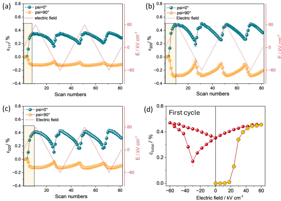
Fig. 3. \{111\}_p ; (b) \{200\}_p ; (c) \{220\}_p and (d) total estimated strain ( \psi = 0^\circ ) calculated from SXR peaks during first cycle of applied field.
