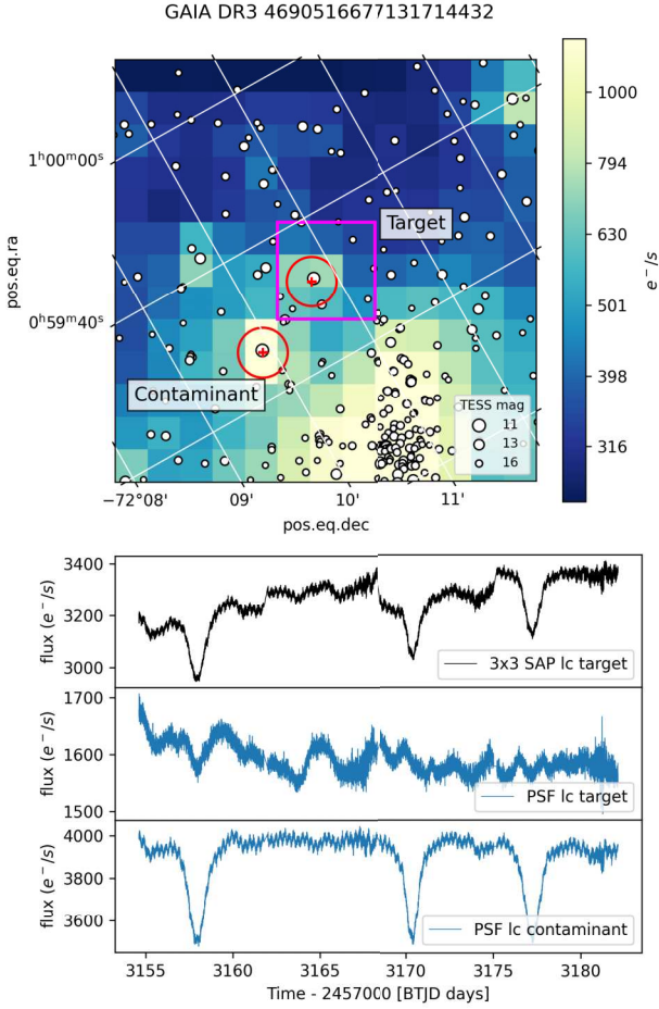
Figure 5. Demonstration of successfully disentangling contamination to reveal a false positive eclipsing binary with TESS data, sector 68. Upper panel: TESS pixel image around BLOeM 4-058 ( Gaia DR3 4690516677131714432). The red circles indicate the FWHM of the Gaussian PSF fit and the magenta rectangle illustrates a standard 3 \times 3 SAP mask. Lower panels: SAP (black) and PSF (blue) extracted light curves as well as the PSF light curve of contaminating stars. The SAP light curve is a combination of multiple sources of variability whereas the PSF light curves effectively disentangle them.
