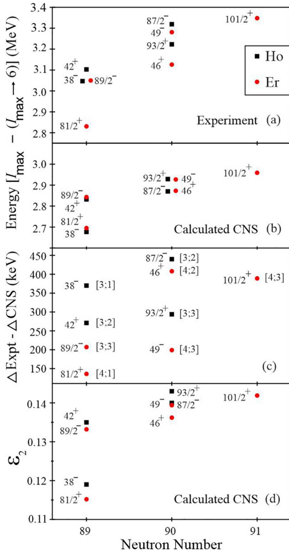
FIG. 23. (a) Experimental energy differences between I_{\max} and (I_{\max} - 6) states observed in ^{156,157}\text{Ho} and ^{157-159}\text{Er} , and (b) the calculated (CNS) energy difference. The particle exchange is a neutron moving from the h_{9/2} ( m_j = 5/2 ) to the f_{7/2} ( m_j = -7/2 ) state. The data are summarized in Table V, and details of the I_{\max} configurations are given in Tables I and II. The experimental energies are taken from [4] ( ^{156}\text{Er} ), [9] ( ^{157}\text{Er} ), [2] ( ^{158}\text{Er} ), [6] ( ^{159}\text{Er} ) and this work ( ^{156,157}\text{Ho} ). (c) Difference between the experimental and calculated (CNS) energies from the I_{\max} to (I_{\max} - 6) levels. The configuration of the I_{\max} level is displayed. (d) Deformation \varepsilon_2 of the I_{\max} states from the CNS calculations; each state is labeled by I^\pi .
