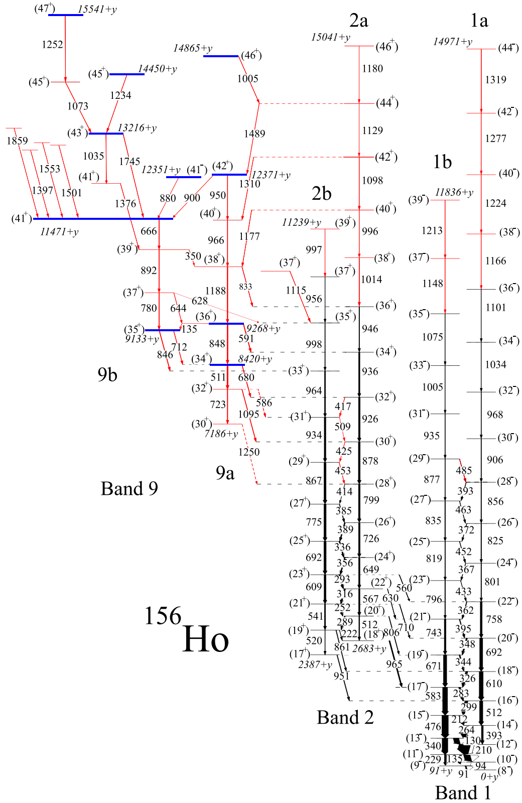
FIG. 1. Partial level scheme for ^{156}\text{Ho} with bands 1, 2, and 9. These bands in ^{156}\text{Ho} have not been connected to the 4^- ground state, so an additional energy y is indicated. New states and \gamma -ray transitions, extending the work of Ref. [22], are in red. Blue states indicate candidate oblate \gamma = 60^\circ states, see Sec. IV and Table I. Arrow widths are proportional to intensity for transitions of intensity >5\% . The white portion in an arrow represents the internal-conversion fraction.
