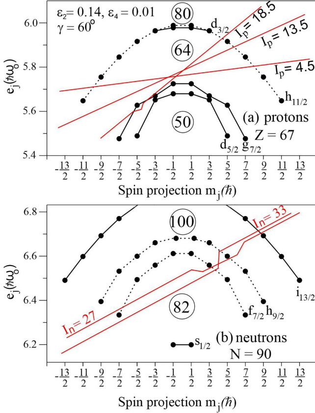
FIG. 16. Calculated single-particle energies at an oblate shape ( \gamma = 60^\circ ), with the x axis labeling the m_j projections of the single-particle angular momentum j onto the nuclear symmetry axis. The tilted Fermi-surfaces (red) indicate potential terminating proton and neutron configurations in ^{157}\text{Ho} . It is convenient to refer to the different states as belonging to one specific j shell but, in practice, the subshells that can be referred to as pseudospin partners are strongly mixed and should rather be referred to as “ dg ” ( d_{5/2}/g_{7/2} ), “ sd ” ( s_{1/2}/d_{3/2} ), and “ fh ” ( f_{7/2}/h_{9/2} ), respectively.
