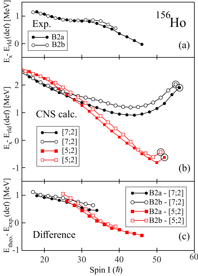
FIG. 19. (a) Energies, relative to a rotating liquid-drop reference, for band 2 in ^{156}\text{Ho} (the signature partners are labeled B2a and B2b). (b) CNS calculations for [7;2] and [5;2] configurations. (c) Energy differences between experiment and theory. Encircled states correspond to I_{\text{max}} oblate states.
