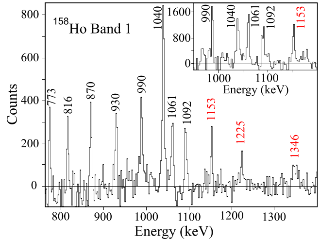
FIG. 11. High-energy part of a triple-gated \gamma^4 coincidence spectrum for the even-spin ( \alpha = 0 ) component of band 1 in ^{158}\text{Ho} . The spectrum was generated with the requirement l-l-1040 -keV; list l includes in-band transitions from 738 ( 24^- \rightarrow 22^- ) to 1225 keV ( 48^- \rightarrow 46^- ), excluding the 1040-keV triplet. The inset is a double-gated \gamma^3 coincidence spectrum with the requirement 1040-1040-keV. Newly identified transitions are in red.
