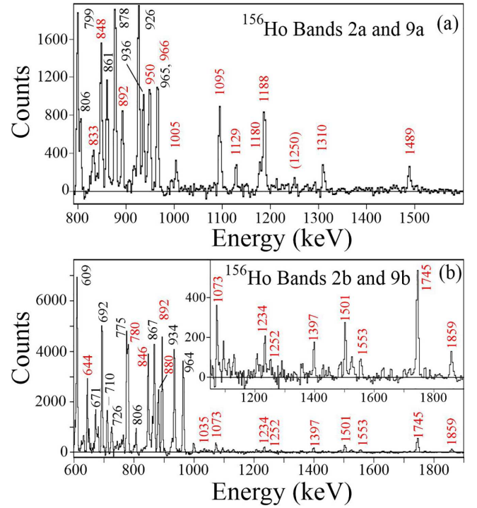
FIG. 4. High-energy part of triple-gated \gamma\gamma coincidence spectra for (a) bands 2a and 9a, and (b) bands 2b and 9b in ^{156}\text{Ho} , respectively. The spectrum in panel (a) was generated with the requirement I1-I1-I1 ; list I1 includes in-band transitions from 649 ( 24^+ \rightarrow 22^+ ) to 878 keV ( 30^+ \rightarrow 28^+ ) in band 2a, and those from 1095 ( 32^+ \rightarrow 30^+ ) to 966 keV ( 40^+ \rightarrow 38^+ ) in band 9a. The spectrum in panel (b) was generated with the requirement I2-I2-666 keV ( 41^+ \rightarrow 39^+ ); list I2 includes in-band transitions from 692 ( 25^+ \rightarrow 23^+ ) to 964 keV ( 33^+ \rightarrow 31^+ ) in band 2b, the 846 ( 35^+ \rightarrow 33^+ ) to 892 keV ( 39^+ \rightarrow 37^+ ) ones in band 9b, and the 965 keV ( 18^+ \rightarrow 17^- ) transition. Newly identified transitions are indicated in red.
