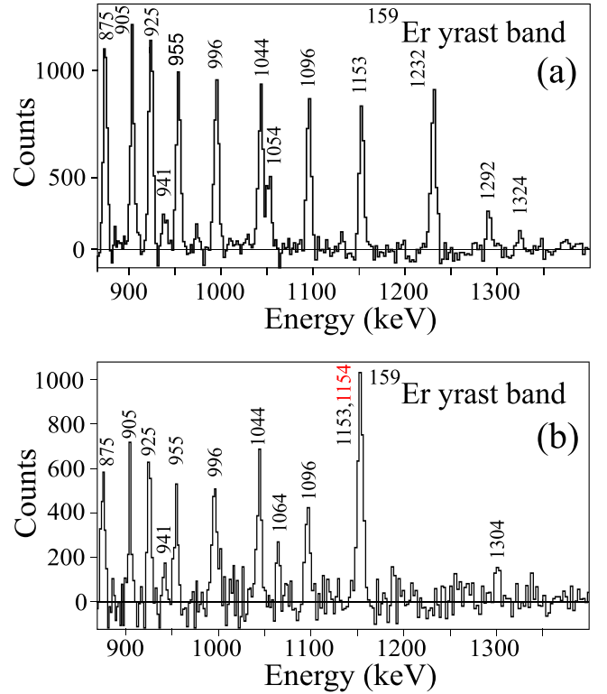
FIG. 13. High-energy part of triple-gated \gamma^4 coincidence spectra for the \alpha = +1/2 yrast band of ^{159}\text{Er} . The spectrum in panel (a) was generated with the requirement l - l -1276 keV, while the spectrum in panel (b) was generated with the requirement l - l -1342 keV. The list l for both spectra includes the in-band transitions from 626 ( 33/2^+ \rightarrow 29/2^+ ) to 1096 keV ( 81/2^+ \rightarrow 77/2^+ ).
