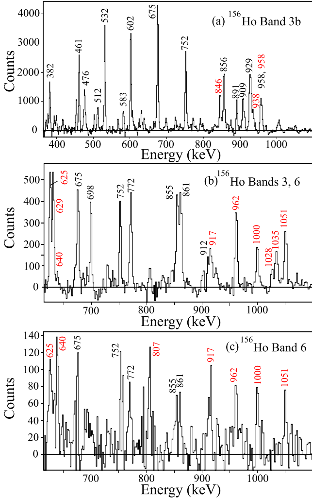
FIG. 5. Representative triple-gated \gamma^4 coincidence spectra for bands 3 and 6 in ^{156}\text{Ho} . The spectrum in panel (a) was generated with the requirement I1-I2-I2 ; the list I1 includes in-band transitions from 382 ( 13^- \rightarrow 11^- ) to 752 keV ( 23^- \rightarrow 21^- ) while list I2 includes in-band transitions from 856 ( 25^- \rightarrow 23^- ) to 891 keV ( 33^- \rightarrow 31^- ) in band 3b. The spectrum in panel (b) was generated with the requirement I3-I3-912 keV ( 28^- \rightarrow 26^- ) in band 3a; list I3 includes transitions in band 6 from 625 ( 32^- \rightarrow 30^- ) to 1000 keV ( 40^- \rightarrow 38^- ). The spectrum in panel (c) highlights the highest-spin transitions in band 6 up to the 640-keV one ( 44^- \rightarrow 42^- ); this spectrum has the gating requirement I4-I4-1028 keV ( 42^- \rightarrow 40^- ), where list I4 includes the 625-, 1051-, 962-, 917-, and 1000-keV transitions in band 6. Newly identified transitions are indicated in red.
