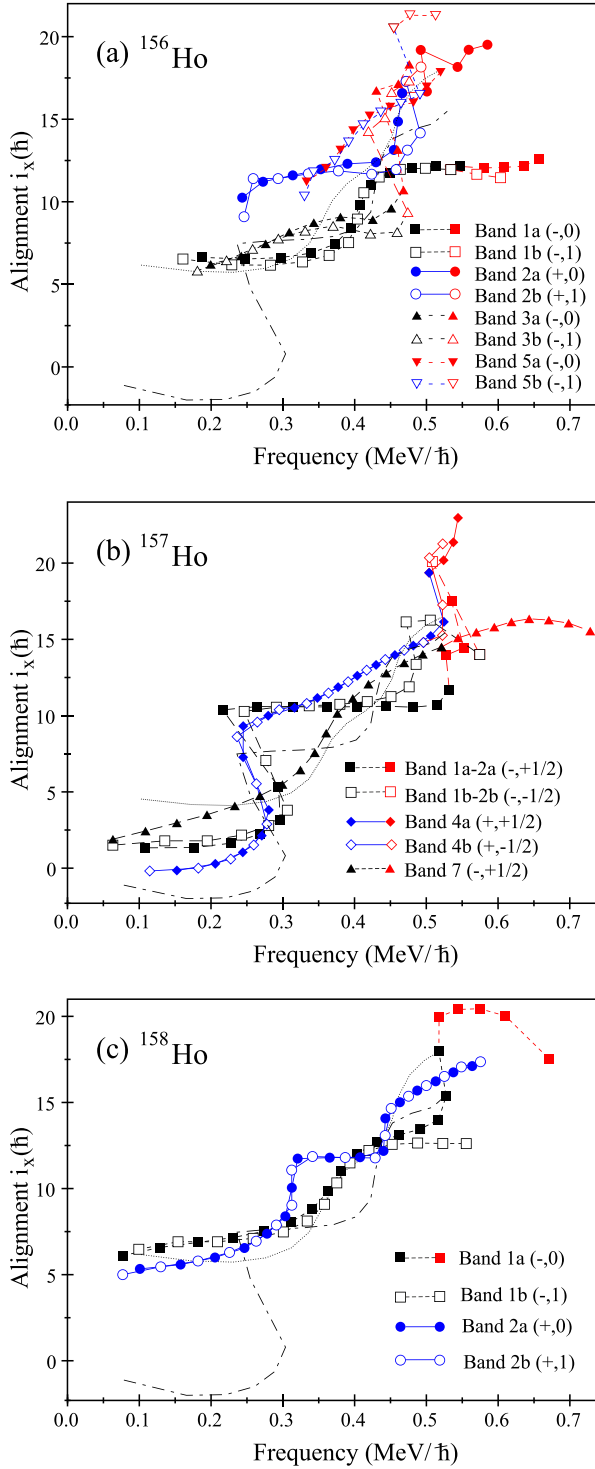
FIG. 17. Experimental alignments i_x as a function of the rotational frequency for bands in ^{156-158}\text{Ho} . Bands are labeled as in the level schemes and by (parity, signature). New states are denoted by red symbols and lines. (a) Bands 1, 2, 3, and 5 in ^{156}\text{Ho} . (b) Bands 2, 4, and 7 in ^{157}\text{Ho} . The noncollective states are not included. (c) Bands 1 and 2 in ^{158}\text{Ho} . The data for band 2 are taken from Refs. [28,29]. The dot-dashed and dotted black lines are the yrast bands in ^{158}\text{Er} and ^{159}\text{Er} , respectively. These are plotted to show the expected position of the first and second (\nu i_{13/2})^2 neutron and first (\pi h_{11/2})^2 proton band crossings.
