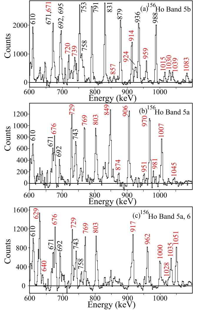
FIG. 6. Representative triple-gated \gamma^4 coincidence spectra for bands 5 and 6 in ^{156}\text{Ho} . The spectrum in panel (a) was generated with the requirement I1-I1-I2 ; the list I1 includes in-band transitions from 695 ( 25^- \rightarrow 23^- ) to 879 keV ( 33^- \rightarrow 31^- ) while list I2 includes in-band transitions from 936 ( 35^- \rightarrow 33^- ) to 959 keV ( 41^- \rightarrow 39^- ) in band 5b. The spectrum in panel (b) was generated with the requirement I1-I1-I2 ; list I1 includes in-band transitions from 676 keV ( 24^- \rightarrow 22^- ) to 803 keV ( 30^- \rightarrow 28^- ) while list I2 includes in-band transitions from 849 ( 32^- \rightarrow 30^- ) to 1007 keV ( 38^- \rightarrow 36^- ) in band 5a. The spectrum in panel (c) was generated with the requirement I1-I1-I1 ; list I1 includes in-band transitions from 729 ( 26^- \rightarrow 24^- ) to 803 keV ( 30^- \rightarrow 28^- ) in band 5a and from 629 ( 32^- \rightarrow 30^- ) to 962 keV ( 36^- \rightarrow 34^- ) in band 6. Newly identified transitions are in red.
