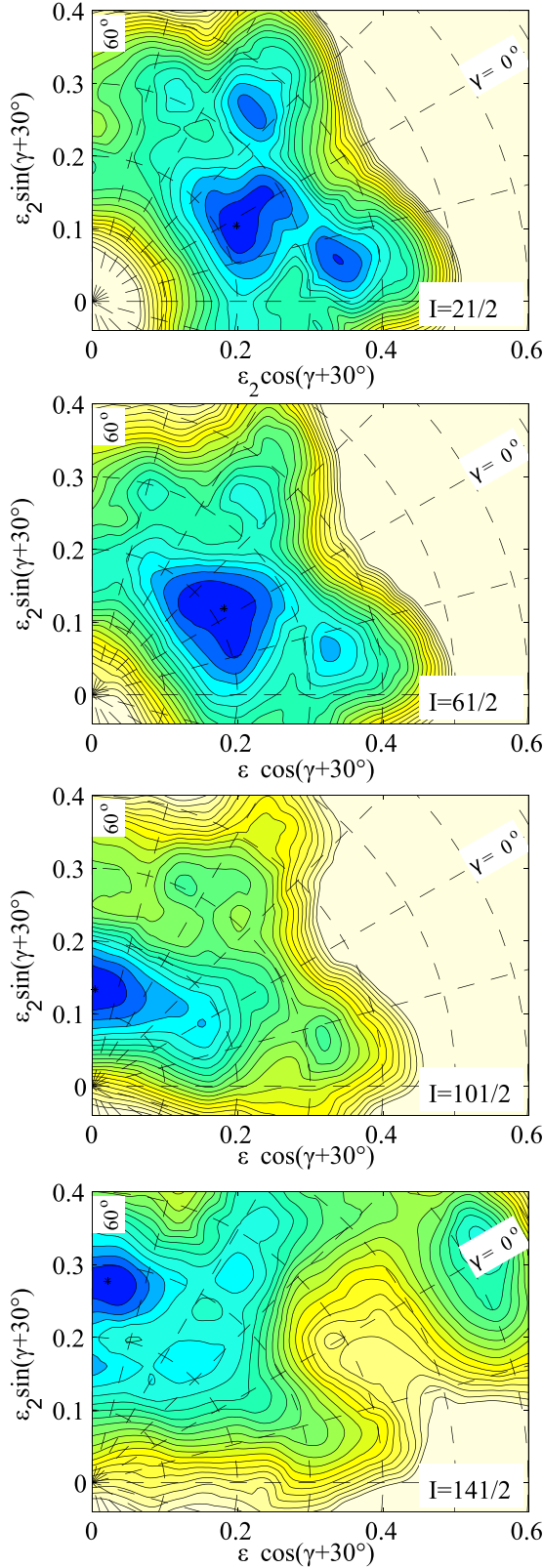
FIG. 14. PES surfaces for the (\pi, \alpha) = (-, +1/2) configuration in ^{157}\text{Ho} , calculated at various spins. The energy contours are separated by 0.25 MeV.
