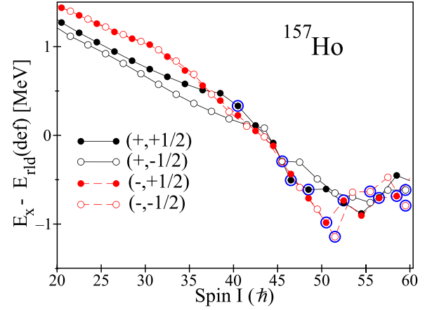
FIG. 15. Calculated CNS excitation energies relative to a deformed rotating-liquid-drop reference, plotted as a function of spin, for the yrast states in ^{157}\text{Ho} , for the four possible combinations of parity and signature. Terminating oblate configurations are encircled in blue. It can be seen that the collective yrast line for spins less than 45\hbar is replaced by a noncollective yrast line for higher spins.
