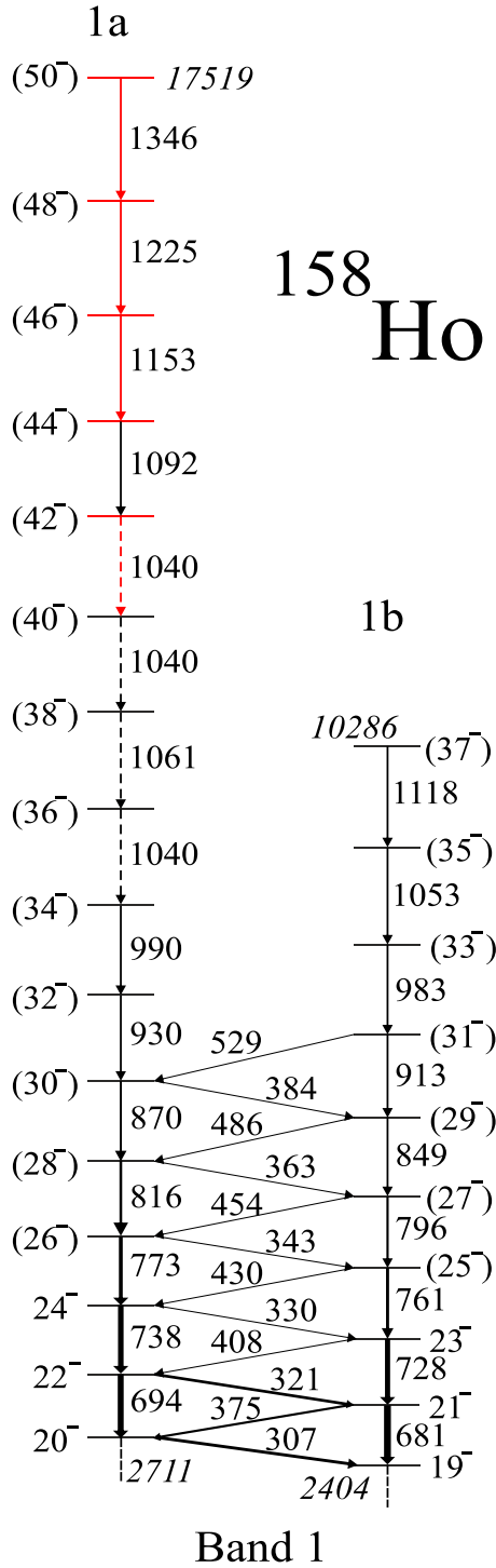
FIG. 10. Level scheme for band 1 in ^{158}\text{Ho} ; 1a even spin, 1b odd. The excitation energy is based on the accepted values in Ref. [28], which is based on Ref. [29]. All energies shown are from this work and in agreement with those in Ref. [28]. The spin-parity of states above 23^- and 24^- , established in Ref. [29], are tentative. New states and \gamma -ray transitions are in red.
