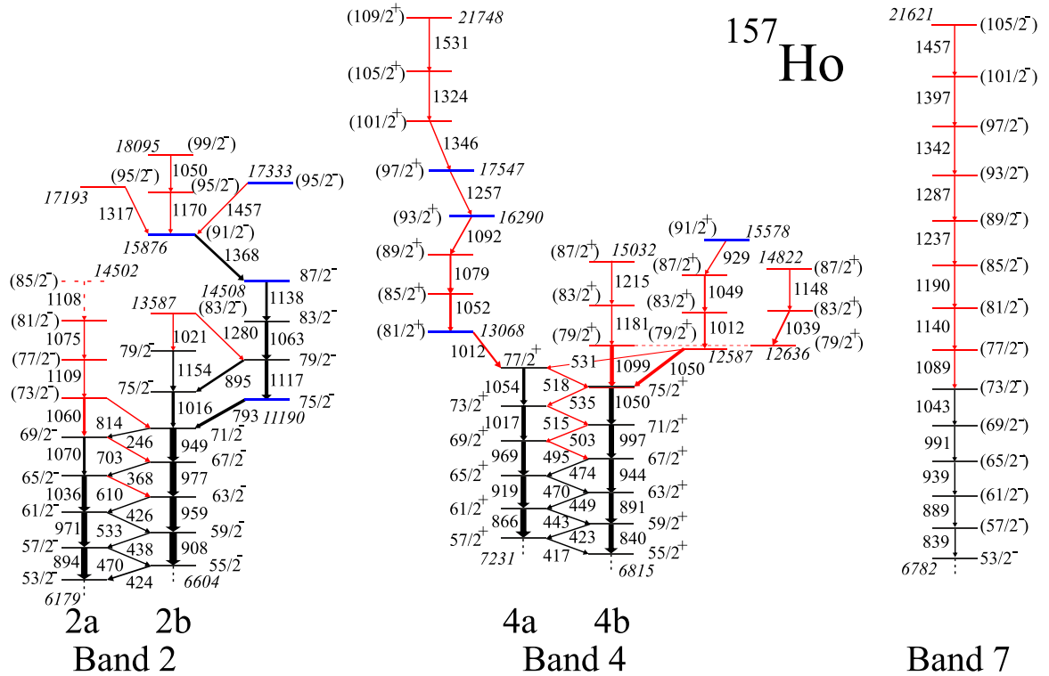
FIG. 7. High-spin region of the levels in bands 2, 4, and 7 in ^{157}\text{Ho} . The excitation and transition energies for known states, in black, are taken from Ref. [8]. New states and \gamma -ray transitions are in red. Blue states indicate candidate oblate \gamma = 60^\circ states, see Sec. IV and Table I.
