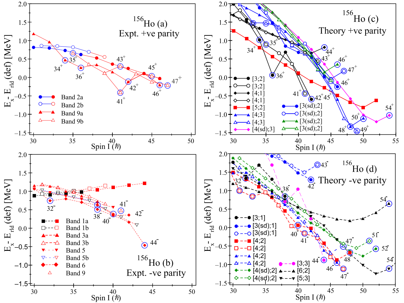
FIG. 20. Experimental and calculated excitation energies in ^{156}\text{Ho} , relative to a deformed rotating-liquid-drop reference, plotted as a function of spin. (a) Positive-parity experimental states, (b) negative-parity experimental ones, (c) low-lying positive parity calculated configurations, and (d) low-lying negative-parity ones. Blue circles indicate oblate ( \gamma = 60^\circ ) configurations. In the experimental plots such states are encircled where a possible corresponding oblate state is identified in theory. In the theory plots, states are labeled by their I^\pi values at high spin or where a candidate experimental state is suggested. The calculated configurations are defined in Table I.
