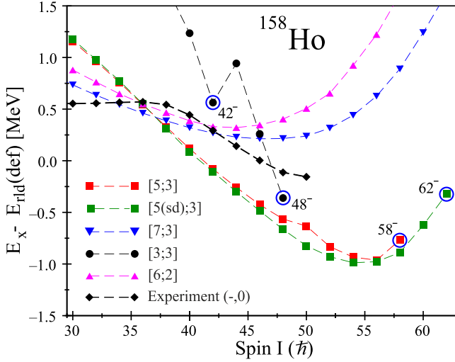
FIG. 22. Experimental excitation energies of the even-spin members of band 1 in ^{158}\text{Ho} plotted relative to a deformed rotating liquid-drop reference. Calculated CNS configurations are also provided.
