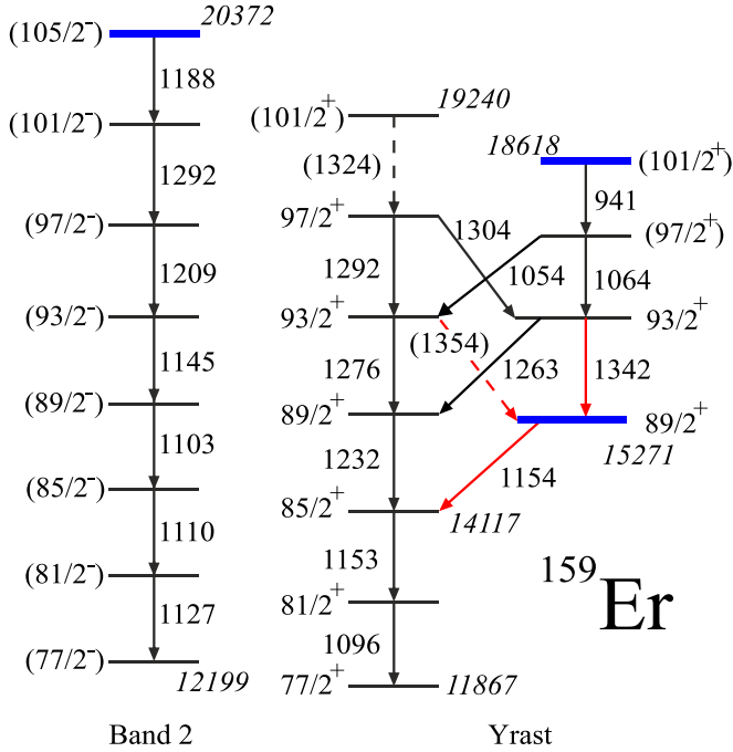
FIG. 12. The high-spin states in ^{159}\text{Er} [6] from 77/2^+ in the yrast positive-parity structure and (77/2^-) in the negative-parity, band 2. The order of the 1154- and 1342-keV transitions (red) is changed compared with Ref. [6]. The states in blue are predicted oblate \gamma = 60^\circ configurations, see Sec. IV and Table II.
