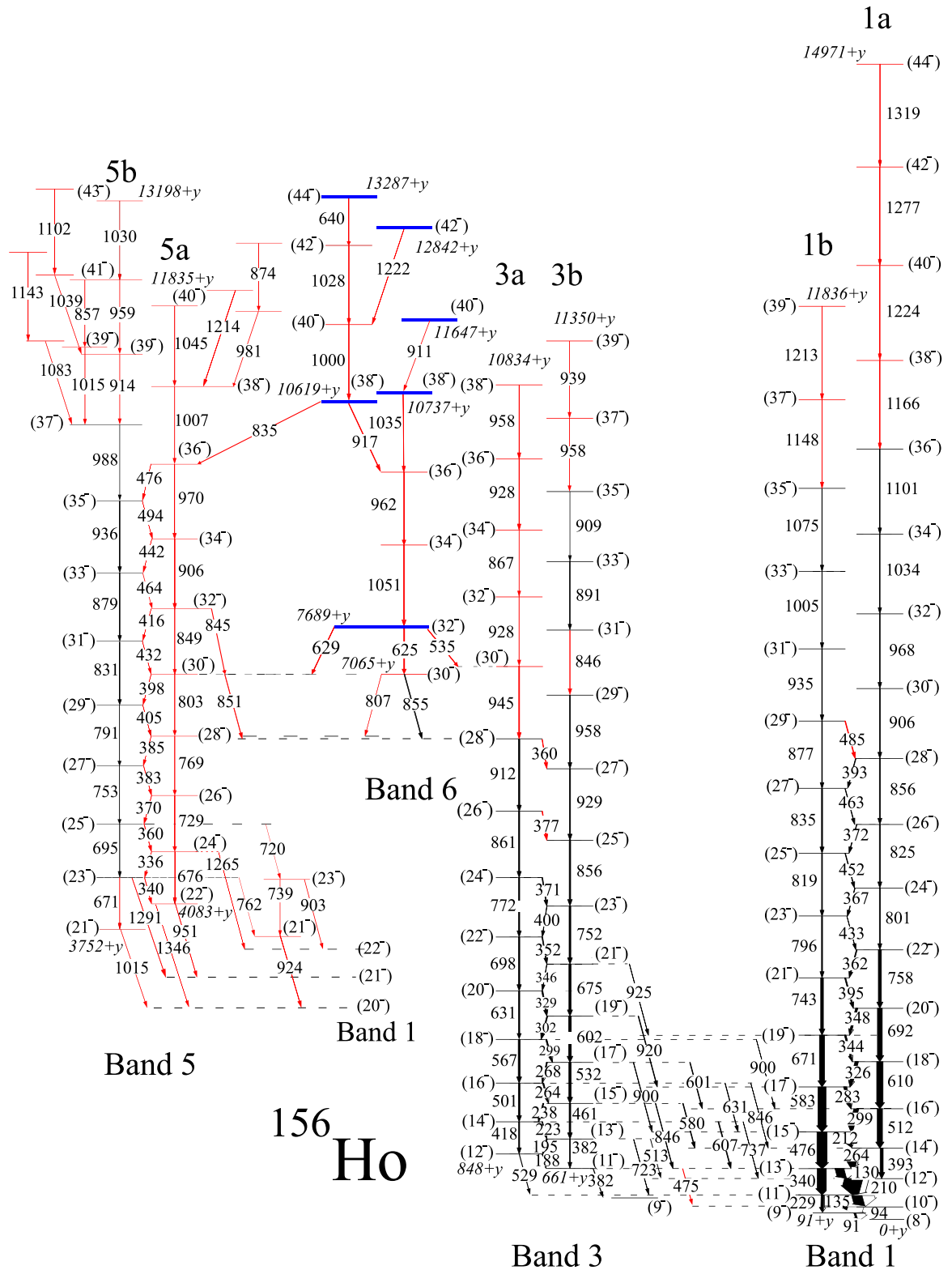
FIG. 2. Partial level scheme for ^{156}\text{Ho} with the negative-parity bands 1, 3, 5, and 6 in ^{156}\text{Ho} . These bands in ^{156}\text{Ho} have not been connected to the 4^- ground state, so an additional energy y is indicated. New states and \gamma -ray transitions, extending the work of Ref. [22], are in red. Blue states indicate candidate oblate \gamma = 60^\circ states, see Sec. IV and Table I. Arrow widths are proportional to intensity, for transitions of intensity >5\% . The white portion in an arrow represents the internal-conversion fraction.
