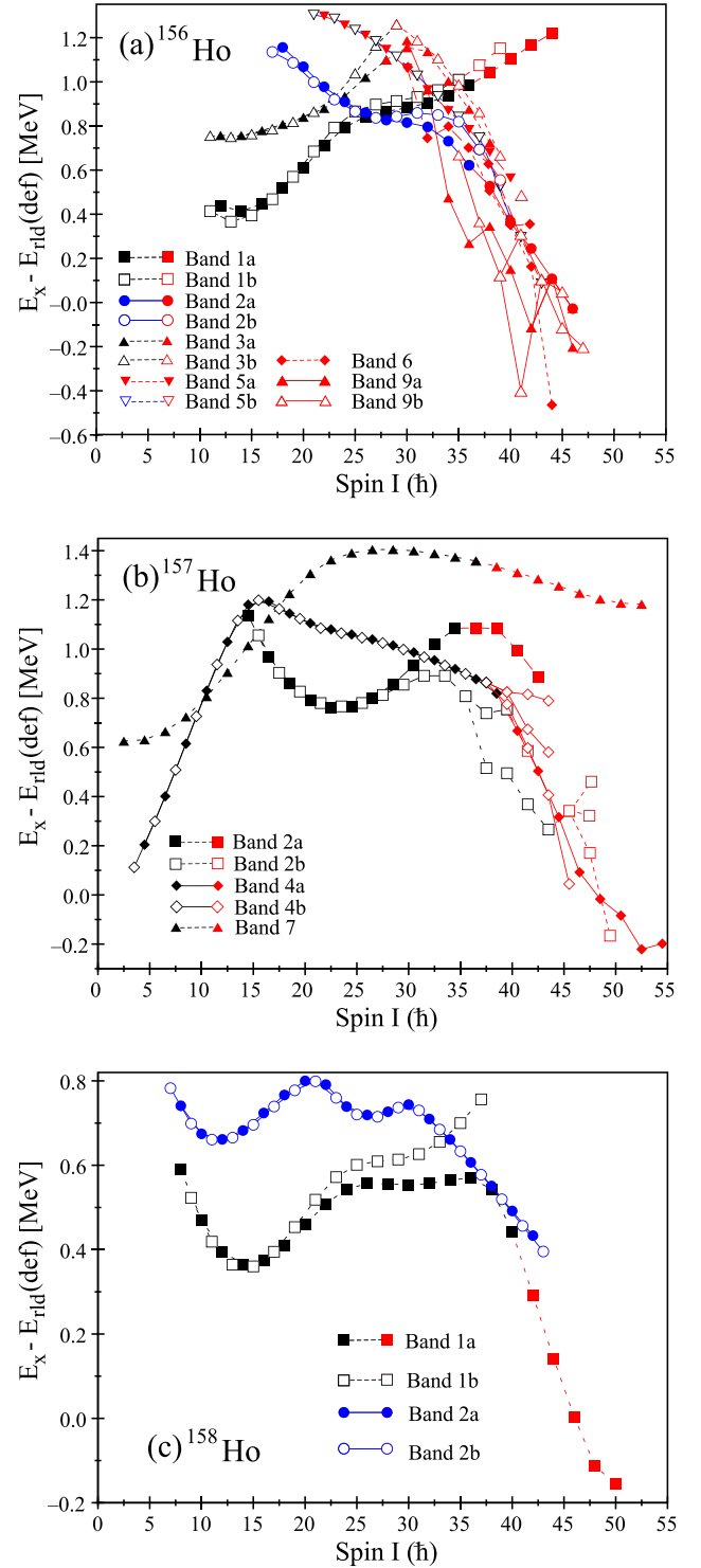
FIG. 18. Experimental excitation energy, relative to a deformed rotating-liquid-drop reference E - E_{\text{rld}} , plotted as a function of spin I for bands in ^{156,157,158}\text{Ho} . New states are denoted by red symbols and lines. (a) Bands 1, 2, 3, 5, 6, and 9, in ^{156}\text{Ho} . (b) Bands 2, 4, and 7 in ^{157}\text{Ho} . (c) Bands 1 and 2 in ^{158}\text{Ho} . The data for band 2 are taken from Refs. [28,29]. The convention for labeling in the alignment, i_x (Fig. 17), and E - E_{\text{rld}} , this figure, is as follows: Parity: solid lines denote positive parity, dashed ones for negative parity. Signature ( \alpha ): Filled symbols denote \alpha = 0 (and \alpha = +1/2 for odd-A nuclei); open symbols denote \alpha = 1 (and \alpha = -1/2 for odd-A nuclei).
