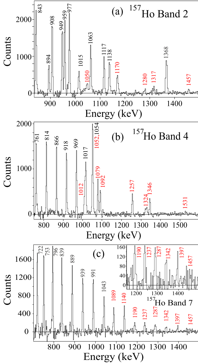
FIG. 8. High-energy part of triple-gated \gamma^4 coincidence spectra representative of (a) band 2, (b) band 4, and (c) band 7 in ^{157}\text{Ho} , respectively. The spectrum in panel (a) was generated with the requirement l1-l1-l2 ; list l1 includes in-band transitions from 591 ( 43/2^- \rightarrow 39/2^- ) to 949 keV ( 71/2^- \rightarrow 67/2^- ) in band 2b while l2 includes the 1117 ( 79/2^- \rightarrow 75/2^- ), 1063 ( 83/2^- \rightarrow 79/2^- ), 1138 ( 87/2^- \rightarrow 83/2^- ), and 1170 keV ( 95/2^- \rightarrow 91/2^- ) transitions. The spectrum in panel (b) was generated with the requirement on l1-l1-l2 ; list l1 includes in-band transitions in band 4a from 703 ( 49/2^+ \rightarrow 45/2^+ ) to 1054 keV ( 77/2^+ \rightarrow 73/2^+ ) while l2 includes the 1012 ( 81/2^+ \rightarrow 77/2^+ ), 1079 ( 89/2^+ \rightarrow 85/2^+ ), and 1092 keV ( 93/2^+ \rightarrow 89/2^+ ) transitions. The spectrum in panel (c) was generated with the requirement l3-l3-l3 ; list l includes in-band transitions from 650 ( 37/2^- \rightarrow 33/2^- ) to 1397 keV ( 101/2^- \rightarrow 97/2^- ). Newly identified transitions are labeled in red.
