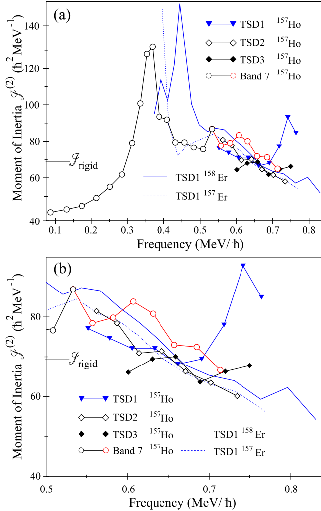
FIG. 24. (a) The dynamic moment of inertia \mathcal{J}^{(2)} as a function of rotational frequency for the three TSD bands tentatively assigned to ^{157}\text{Ho} , band 7 in ^{157}\text{Ho} , and the strongest sequences (labeled TSD1) in ^{158}\text{Er} and ^{157}\text{Er} [11]. New states in band 7 correspond to the red symbols. (b) Expanded plot for high frequency. The rigid-body moment of inertia for mass 157 and a deformation of \beta_2 = 0.3 is indicated.
