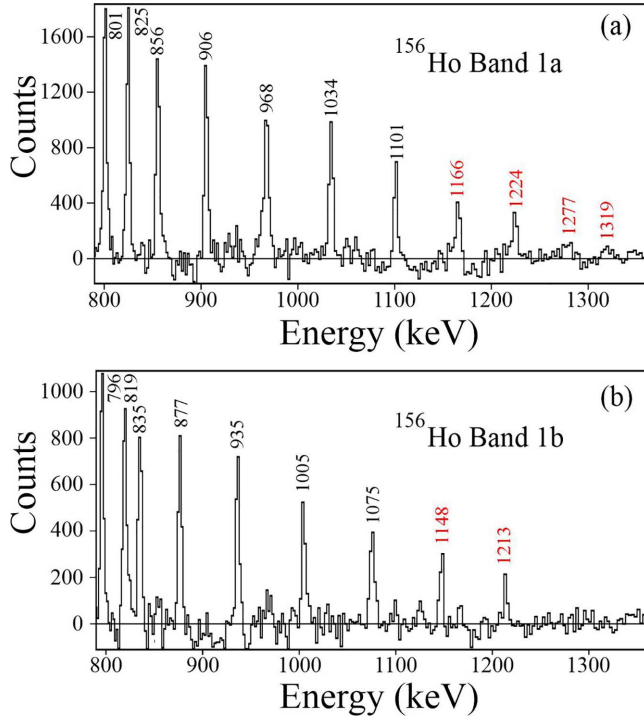
FIG. 3. Triple-gated \gamma\gamma coincidence spectra representative of (a) band 1a, and (b) band 1b in ^{156}\text{Ho} , respectively. The band 1(a) spectrum in panel (a) was generated using gate-lists with the requirement I1-I1-I2 ; list I1 contains in-band transitions from 512 ( 16^- ) \rightarrow 147 ( 14^- ) to 968 keV ( 32^- ) \rightarrow ( 30^- ), while list I2 contains those from 1034 ( 34^- ) \rightarrow ( 32^- ) to 1277 keV ( 42^- ) \rightarrow ( 40^- ). The band 1b spectrum in panel (b) was generated with the requirement I1-I1-I2 ; list I1 contains in-band transitions from the 671 ( 19^- ) \rightarrow ( 17^- ) to 935 keV ( 31^- ) \rightarrow ( 29^- ) and list I2 contains those from 1005 ( 33^- ) \rightarrow ( 31^- ) to 1213 keV ( 39^- ) \rightarrow ( 37^- ). Newly identified transitions are indicated in red.
