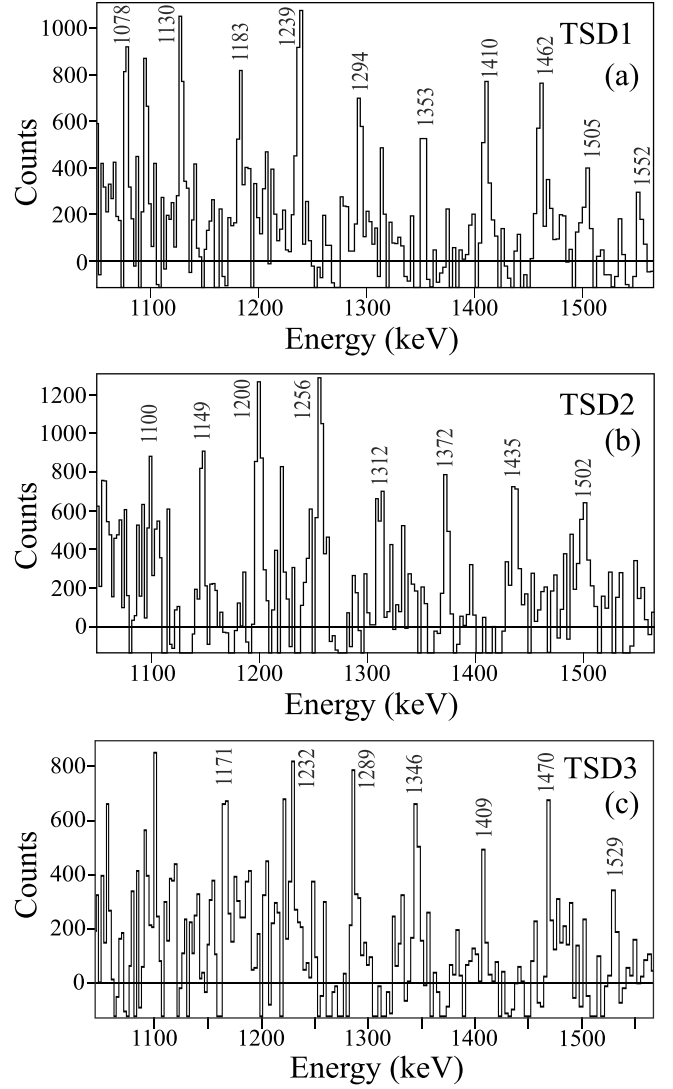
FIG. 9. Double-gated \gamma^3 spectra for the three TSD structures tentatively assigned to ^{157}\text{Ho} . The spectrum in panel (a) was generated with the requirement l-l ; the list l contains transitions from 1183 to 1462 keV. The spectrum in panel (b) was generated with the requirement l-l ; the list l contains transitions from 1149 to 1435 keV. The spectrum in panel (c) was generated with the requirement l-l ; the list l contains transitions from 1171 to 1409 keV.
