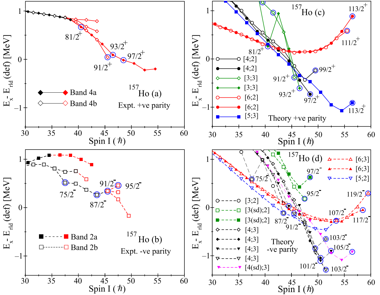
FIG. 21. Experimental and calculated excitation energies in ^{157}\text{Ho} , relative to a deformed rotating liquid-drop reference, as a function of spin. (a) Band 4, (b) band 2, (c) calculated low-lying positive-parity configurations, and (d) low-lying negative-parity ones. Blue circles indicate oblate ( \gamma = 60^\circ ) configurations. The calculated configurations are defined in Table I.
