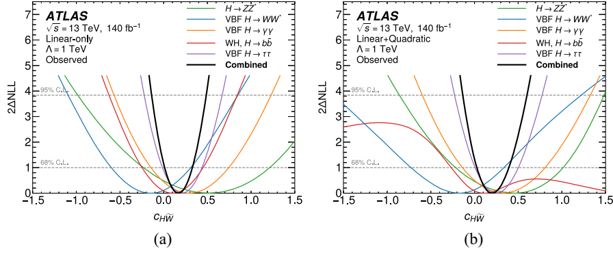
FIG. 5. Observed 2\Delta\text{NLL} scans as a function of c_{H\tilde{W}} considering the (a) linear-only and the (b) linear plus quadratic terms for the individual channels (in different colors) and their combination. The dashed horizontal lines show the values of \Delta\text{NLL} thresholds defining the 68% and 95% confidence levels, assuming the asymptotic approximation.
