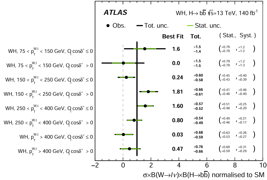
FIG. 1. Measured WH production cross sections times the W \rightarrow \ell \nu and the H \rightarrow b \bar{b} branching ratios normalized to their SM predictions. The best fit values and corresponding uncertainties (total as well as its statistical and systematic components) are shown for all regions. Theoretical uncertainties on the predictions are not shown as they are too small to be visible.
