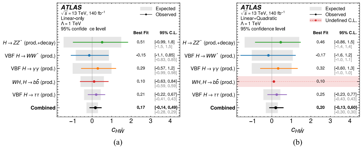
FIG. 6. Best-fit values and 95% C.L. intervals for c_{H\tilde{W}} obtained in single-parameter fits for each of the individual analyses and the combined result, for both (a) linear-only and (b) linear and quadratic interpretations. For the WH, H \rightarrow b\bar{b} linear and quadratic result, the best-fit value is valid in the c_{H\tilde{W}} range [-1.5, 1.5] and no 95% C.L. interval is defined, as explained in the text.
