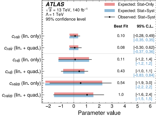
FIG. 4. Best-fit values and 95% C.L. intervals for all three Wilson coefficients obtained in a simultaneous fit to all coefficients. In both cases, linear and linear plus quadratic scenarios are shown. Expected limits using the full model and statistical only are also presented.
