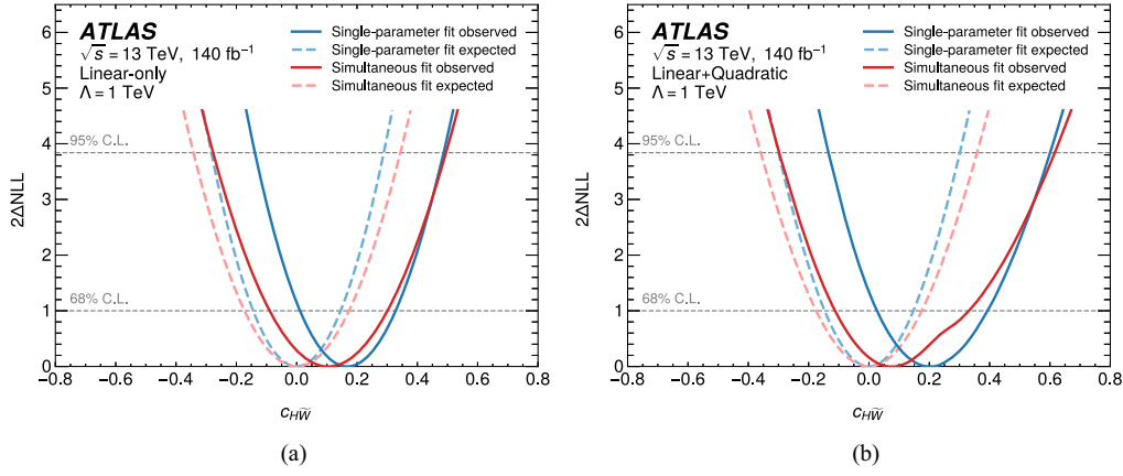
FIG. 2. Negative profile log-likelihood ratio scans are shown as a function of c_{H\bar{W}} , with single-parameter fits ( c_{H\bar{B}} = c_{H\bar{W}B} = 0 ) and simultaneous fits (all three coefficients floating), for (a) linear-only and (b) linear plus quadratic terms. Solid lines indicate the observed scans, while dashed lines show the expected results. The dashed horizontal lines show the thresholds defining the 68% and 95% confidence levels, assuming the asymptotic approximation.
