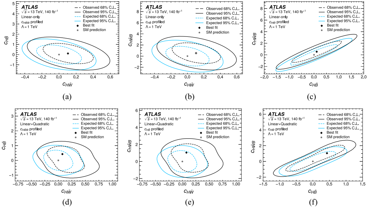
FIG. 3. Observed 68% (dashed line) and 95% (solid line) C.L. two-dimensional contours are shown for all three pairings of the Warsaw basis: (a),(d) c_{H\bar{W}} versus c_{H\bar{B}} , (b),(e) c_{H\bar{W}} versus c_{H\bar{W}B} , and (c),(f) c_{H\bar{B}} versus c_{H\bar{W}B} a simultaneous fit, for (a)–(c) linear-only and (d)–(f) linear plus quadratic terms interpretations. Expected contour lines are also shown. All couplings scale as 1/\Lambda^2 with \Lambda = 1 TeV.
