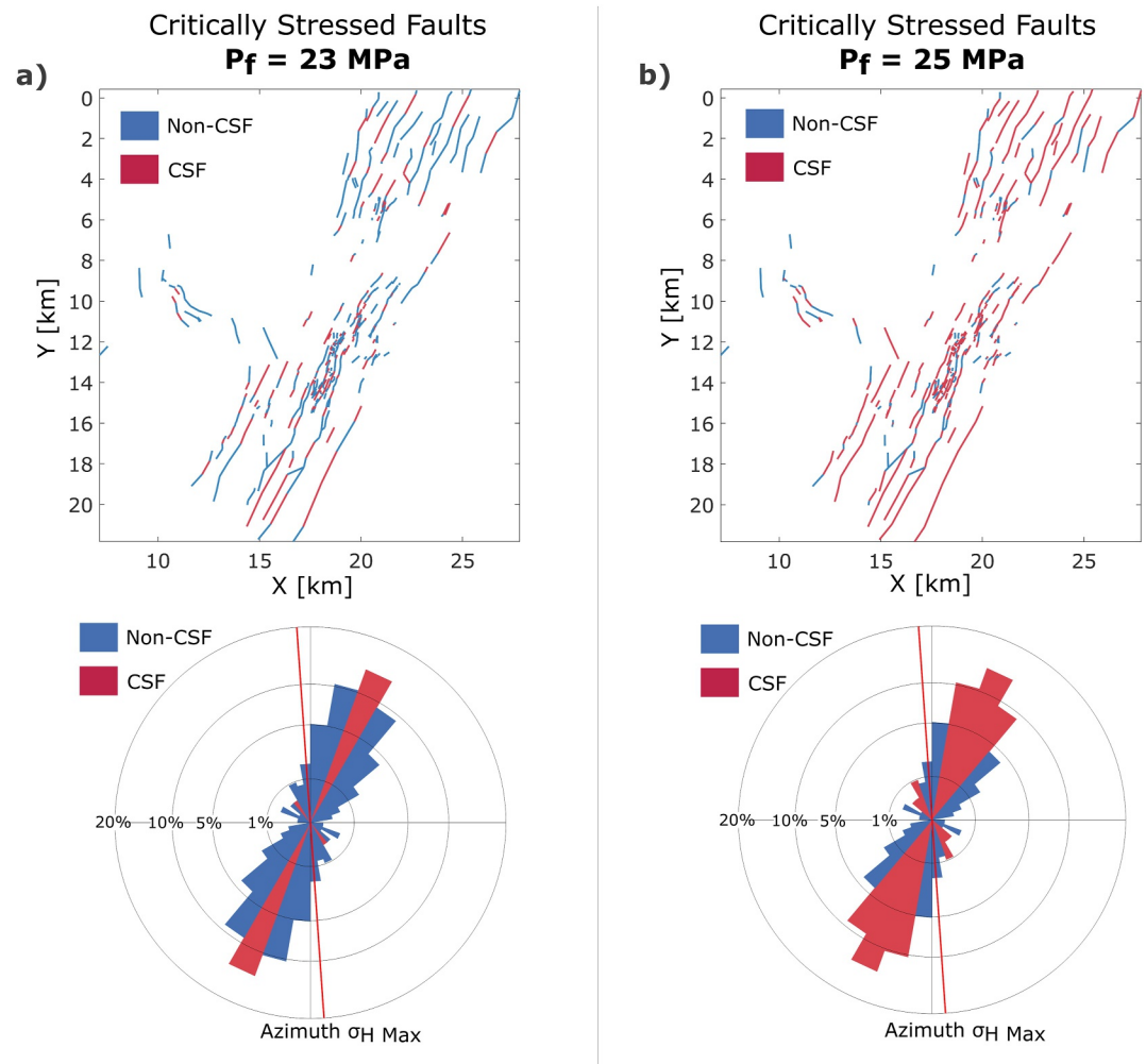
Figure 8. Modeled critically stressed faults (CSF) as deviation from the current hydrostatic condition. We modeled two possible scenarios of pore fluid increase: (a) a relatively small increase of pore fluid pressure, that is, 3 MPa from the current hydrostatic pressure condition ( P_f = 20 MPa at 2 km depth). (b) Marked increase in pore fluid pressure (5 MPa). The two top figures illustrate fault segment traces for the critically stressed faults (red lines), while the bottom figures show the relative rose diagrams (red petals indicate the strikes for the critically stressed faults).
