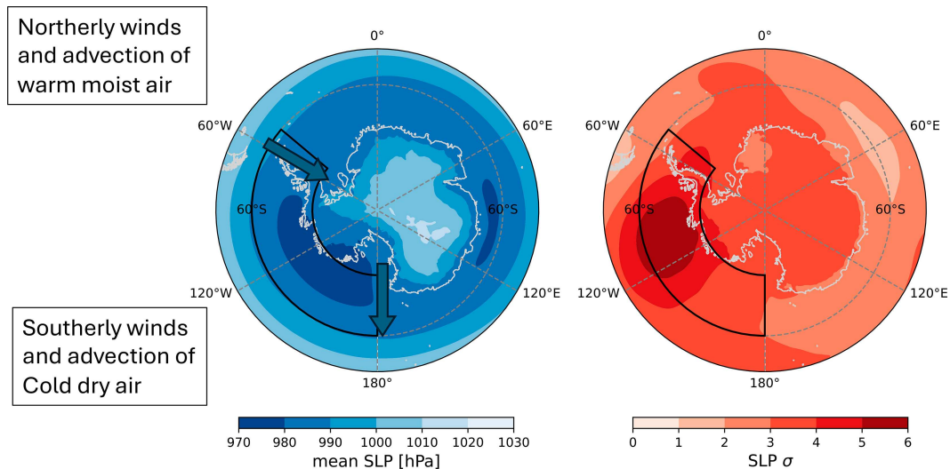
FIG. 1. (a) Mean and (b) SD of SON SLP over the Southern Hemisphere mid-high latitudes, 1979–2023, using ERA5 data. The box shows the region used to calculate the area-averaged ASL index ( 180^{\circ} – 310^{\circ} E, 60^{\circ} – 75^{\circ} S).
