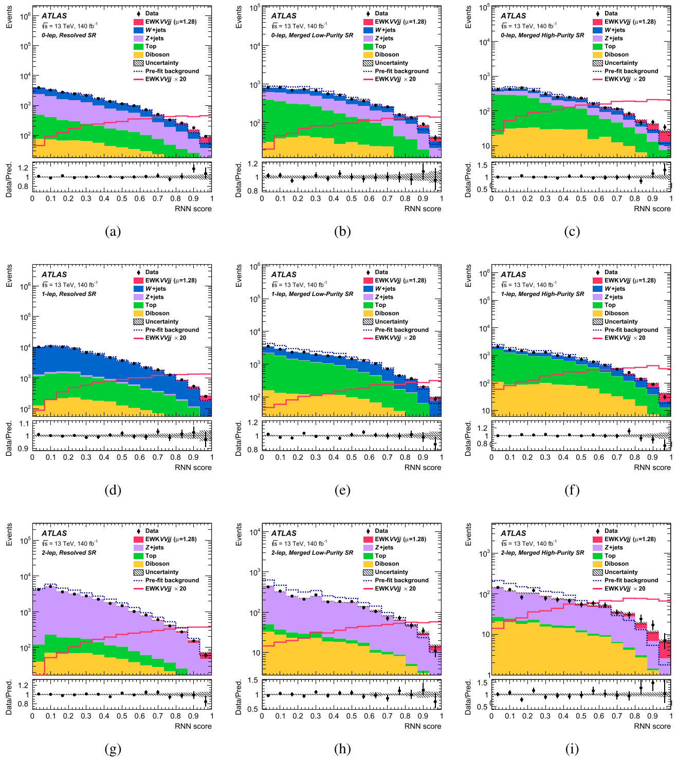
Fig. 8 Distribution of the RNN score for data (dots) and post-fit prediction separated by process (stacked histograms). The EWK VVjj signal is also shown separately scaled by visibility by a factor of 20. For comparison, the pre-fit background distribution is overlaid as a
