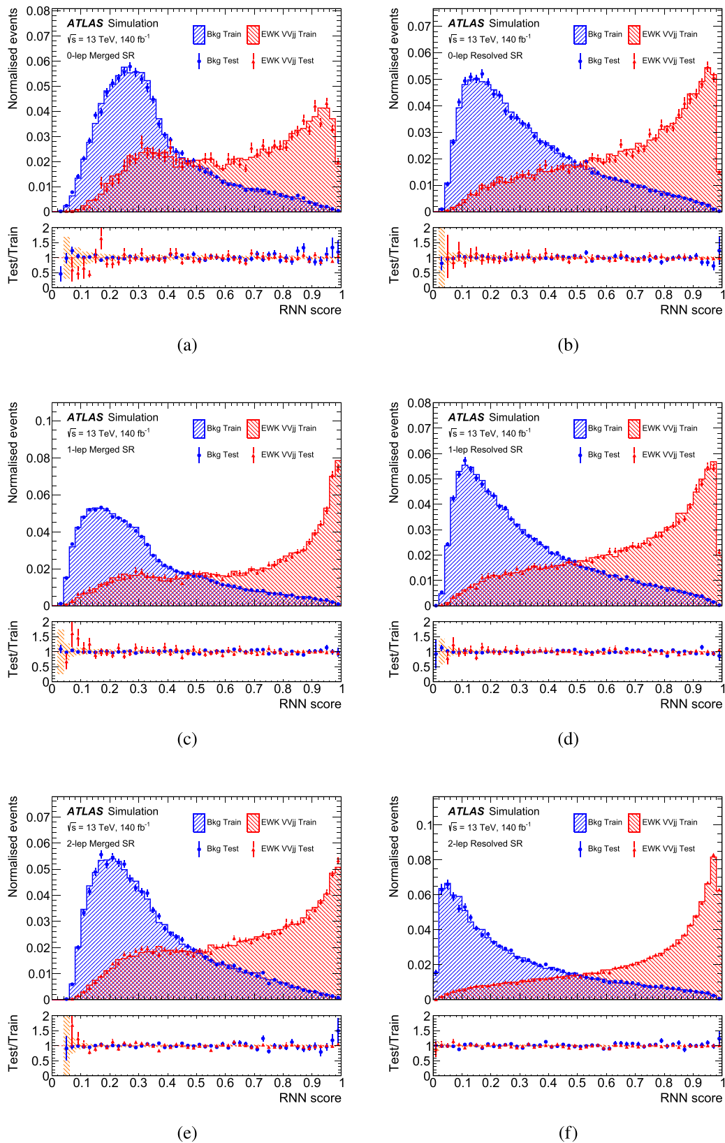
Fig. 6 RNN score distributions for signal and background samples showing the training (histograms) and test (markers) datasets for the a, b 0-, c, d 1- and e, f 2-lepton a, c, e merged and b, d, f resolved
