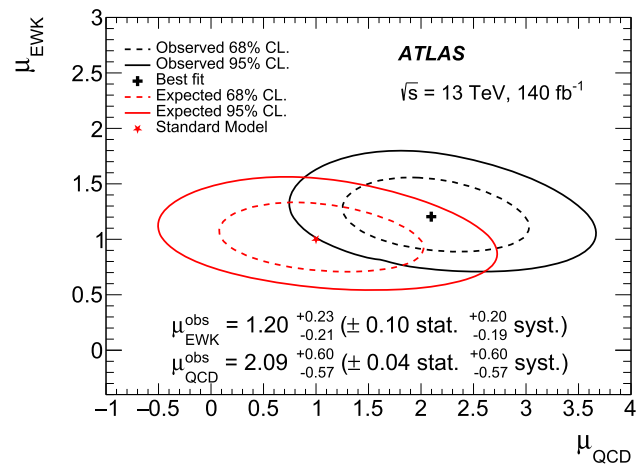
Fig. 10 The two dimensional 68% and 95% negative log-likelihood contours for the simultaneous fit to \mu_{EWK} and \mu_{QCD} . The SM prediction from the generator is highlighted as a star
