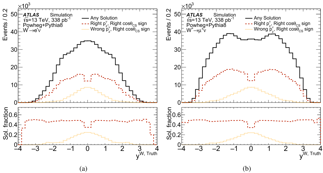
Fig. 1 W -boson rapidity distributions for events reconstructed with the correct or the wrong sign of \cos \theta_{CS} for the a W^- \rightarrow e^- \nu and the b W^+ \rightarrow \mu^+ \nu channels. Events with the chosen solution closest to the true p_z^\nu are labelled as right p_z^\nu . Events with an unambiguous determination of \cos \theta_{CS} are labelled as right \cos \theta_{CS} sign. The differences between the electron and muon distributions reflect both the different
