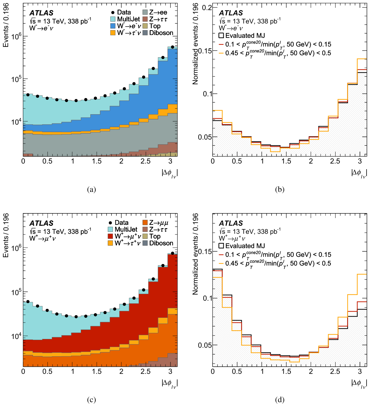
Fig. 2 |\Delta\phi_{\ell\nu}| distribution in the fit region for data, multijet background and for signal and background from simulation in the a W^- \rightarrow e^- \nu and c W^+ \rightarrow \mu^+ \nu channel. The multijet template shown in the plots is the one obtained from data in the first anti-isolation interval, as an exam-
