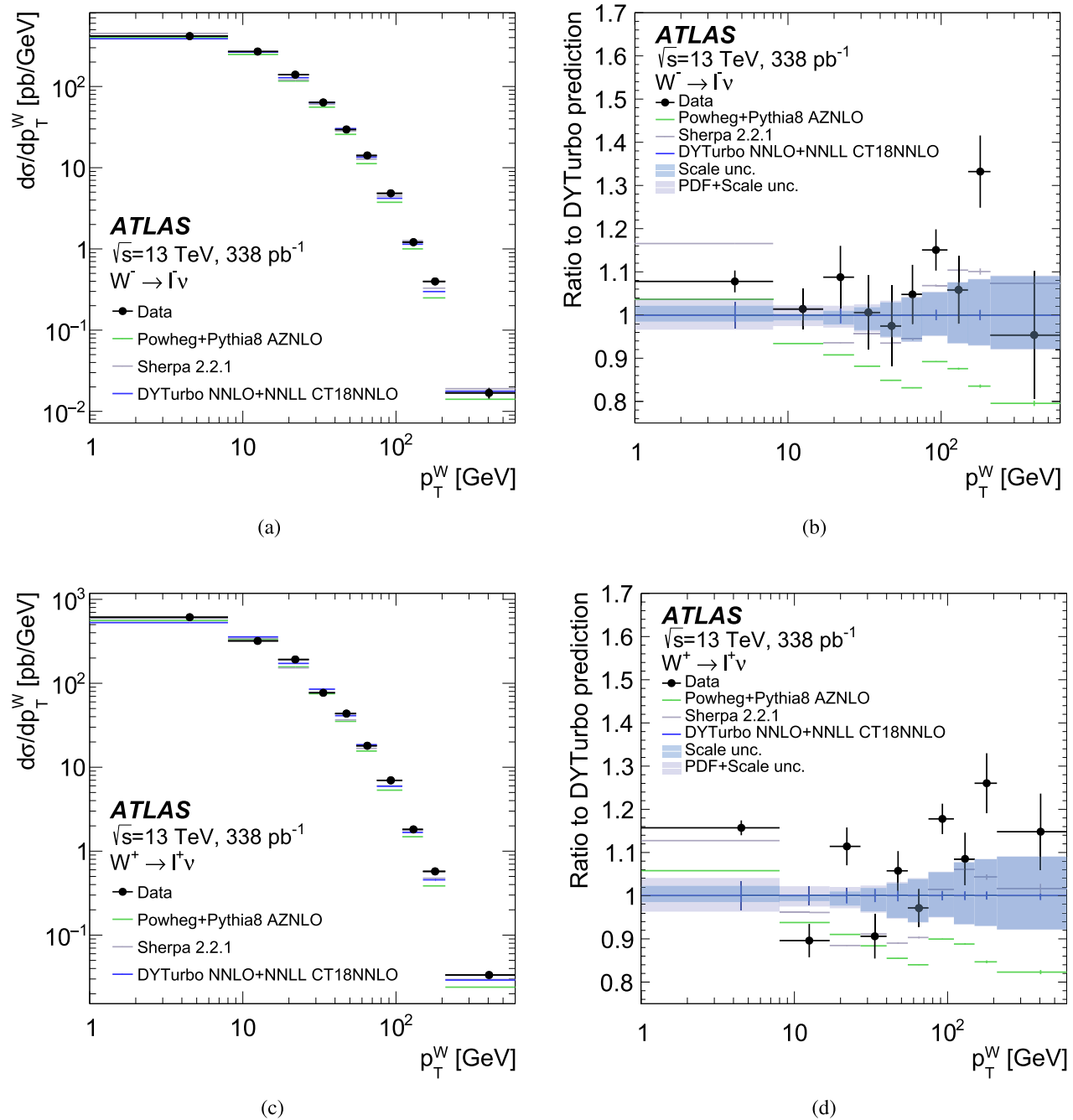
Fig. 17 Comparison of the measured absolute differential cross-sections \frac{d\sigma}{dp_T} for a W^- and c W^+ bosons with predictions from POWHEG and SHERPA event generators, as well as from DYTURBO. The quoted cross-sections include the branching ratio to a single lepton flavour. Ratio of the measured \frac{d\sigma}{dp_T} and the MC predictions to DYTURBO for
