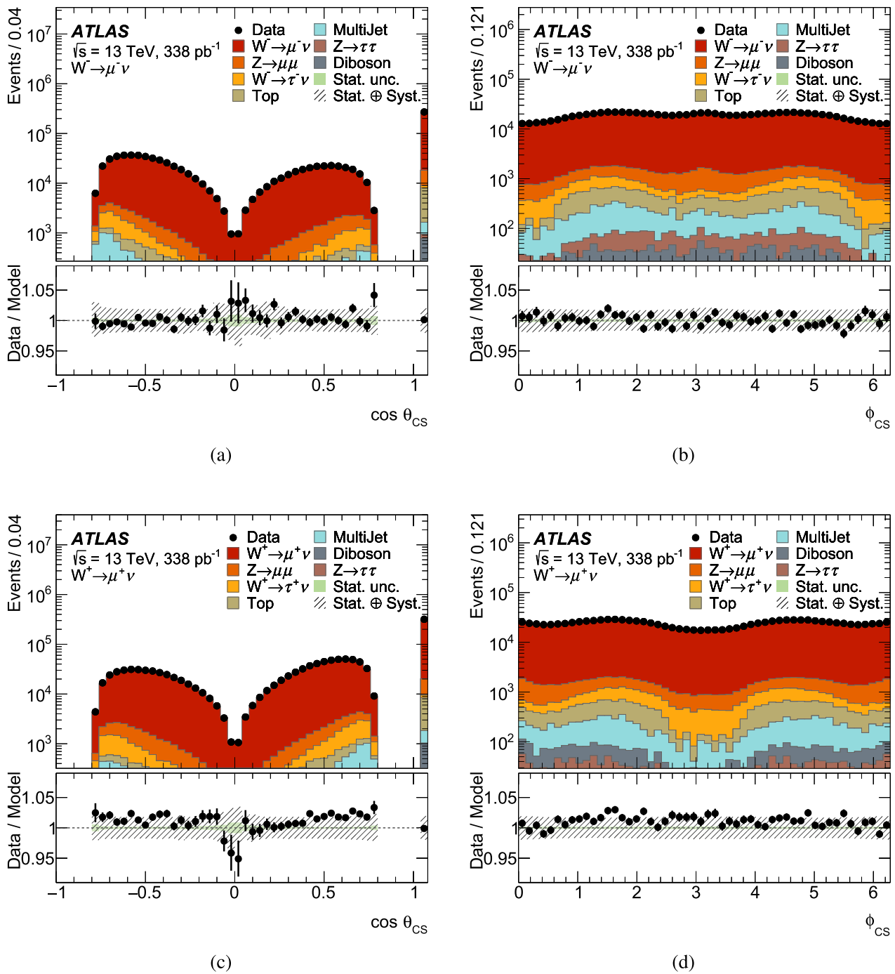
Fig. 6 The \cos \theta_{CS} and \phi_{CS} angular distributions, integrated over p_T^{\ell \nu} for the W \rightarrow \mu \nu channel for a, b negative and c, d positive leptons. The expected distributions are shown separately for the signal and the
