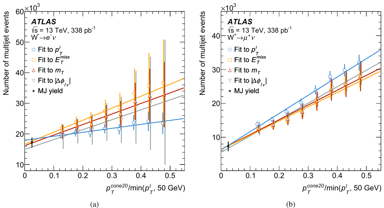
Fig. 3 Examples of multijet event yields extraction procedure from the template fit described in the text as a function of the different anti-isolation regions in p_T^{\text{cone20}}/\min(p_T^l, 50 \text{ GeV}) are shown for the a W^- \rightarrow e^- \nu and the b W^+ \rightarrow \mu^+ \nu channels. The legend indicates
