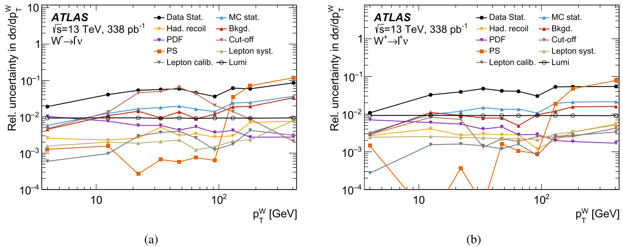
Fig. 11 The breakdown into statistical and systematic components of all the uncertainties for the measured \frac{d\sigma}{dp_T^W} in the a W^- \rightarrow \ell^- \nu and b W^+ \rightarrow \ell^+ \nu channel, as obtained from the full fit. The values are given as relative uncertainty. The uncertainty of 0.92% in the integrated luminosity is included
