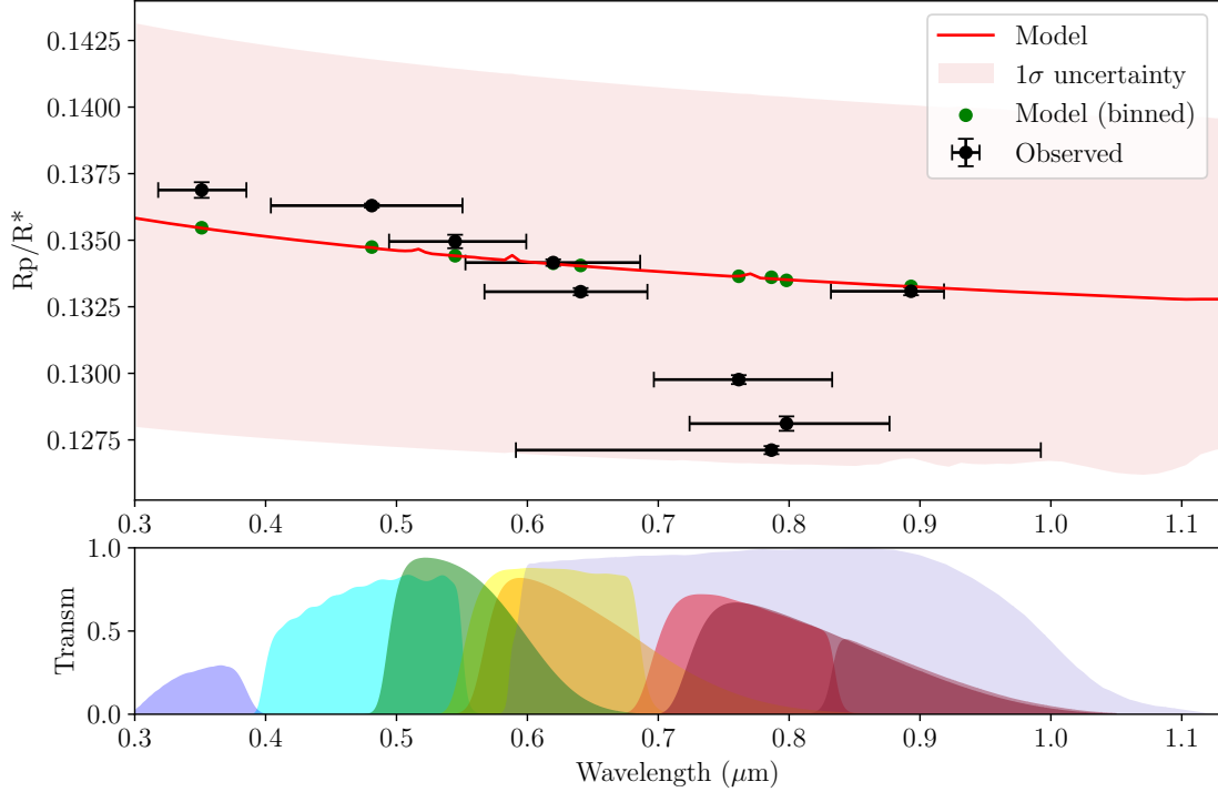
Figure 6. Top panel: retrieved transmission spectrum of WASP-11 b/HAT-P-10 b with forward models generated using PLATON. Bottom panel: Band-pass filter profiles for u' , g' , V , r' , R , i' , I , TESS , and z' (from left to right).
