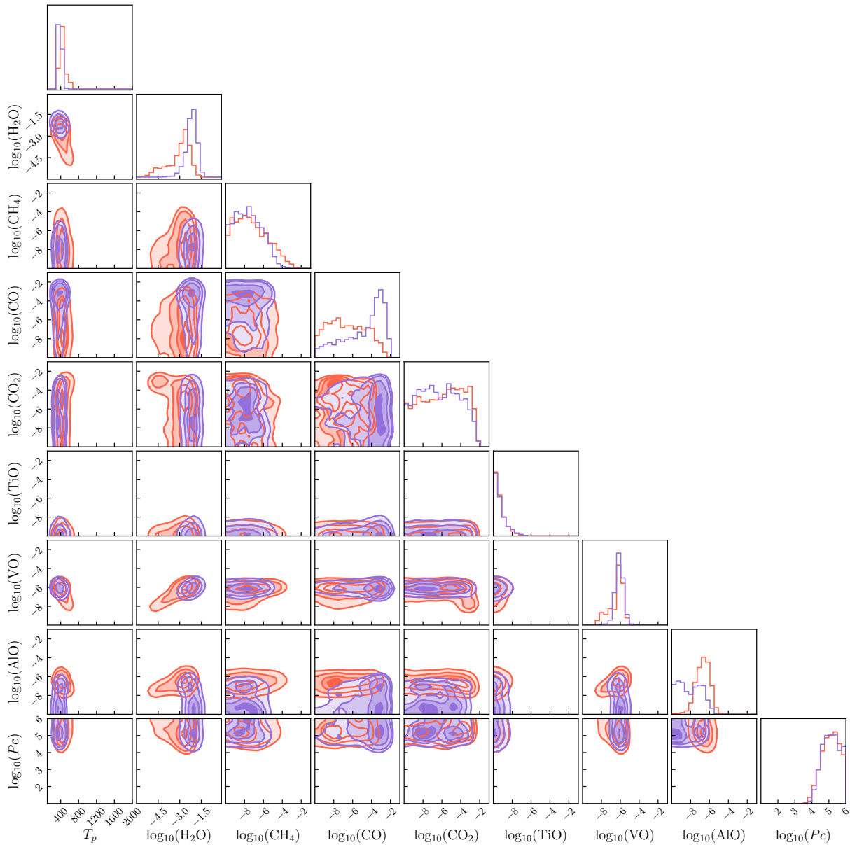
Figure E2. Posterior probability distributions for the transmission spectrum model of WASP-43 b across the full wavelength coverage: Case III, ground-based +TESS+HST/Iraclis+JWST (red); case IV, ground-based+TESS+HST/TransitFit+JWST (purple). The retrieved parameter values correspond to the 16th and 84th percentiles of the posterior distributions, representing the 1\sigma credible intervals.
