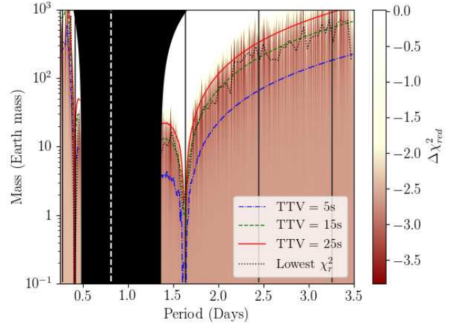
Figure 7. Upper mass limit of the perturbing planet in the WASP-43 system. The best \Delta\chi^2_{\text{red}} values, binned with a period ratio of 0.05, are shown as the black dotted line. The upper mass limits for TTV amplitudes of 5, 15, and 25 s are represented by the blue dashed-dotted, green dashed, and red solid lines, respectively. The white vertical line represents the orbital period of WASP-43 b. The black vertical lines, from left to right, indicate the orbital period resonances of 2:1, 1:2, 1:3, and 1:4. The contour illustrates the \Delta\chi^2_{\text{red}} values from comparing the best TTV model to the best linear model. The unstable orbit region is shown as the shaded black area.
