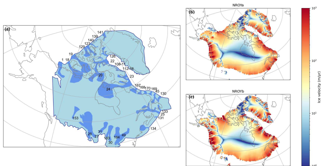
Figure 8. (a) Empirical reconstruction of the active LGM Laurentide ice sheet ice streams (adapted from Margold et al. (2018), and (b) NROYa and (c) NROYb ice velocities at the end of the 5000 year simulations.
