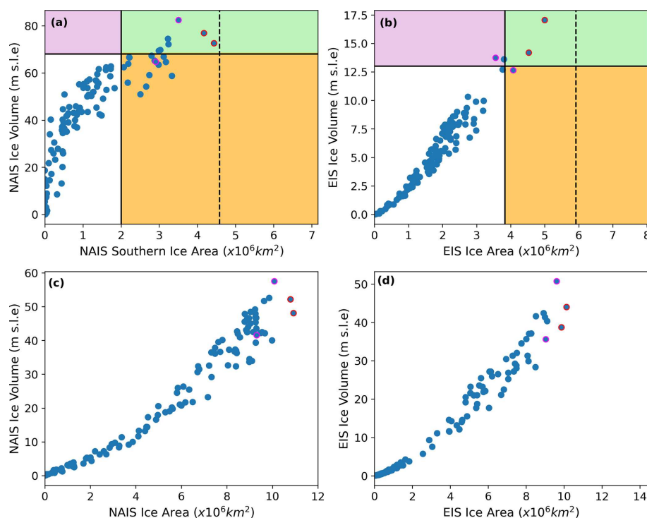
Figure 6. Results from the full ensembles of simulations showing (a) LGM North American ice sheet southern area versus volume and (b) LGM Eurasian ice sheet area versus volume. The solid lines show the minimum values used in the implausibility metric for area and extent and the dotted line shows the actual extent of the ice sheet reconstructions. Simulations that fall within the green box satisfy area and volume constraints for each individual ice sheet, the orange box indicates they satisfy the area constraints only and purple only the volume constraints. The points outlined in red are the 2 NROY simulations (i.e. fall into the green box for both ice sheets) and the points outlined in pink are the additional NROY extent and NROY volume simulations. Panels (c) and (d) show the equivalent results for the PGM ensembles without the constraints.
