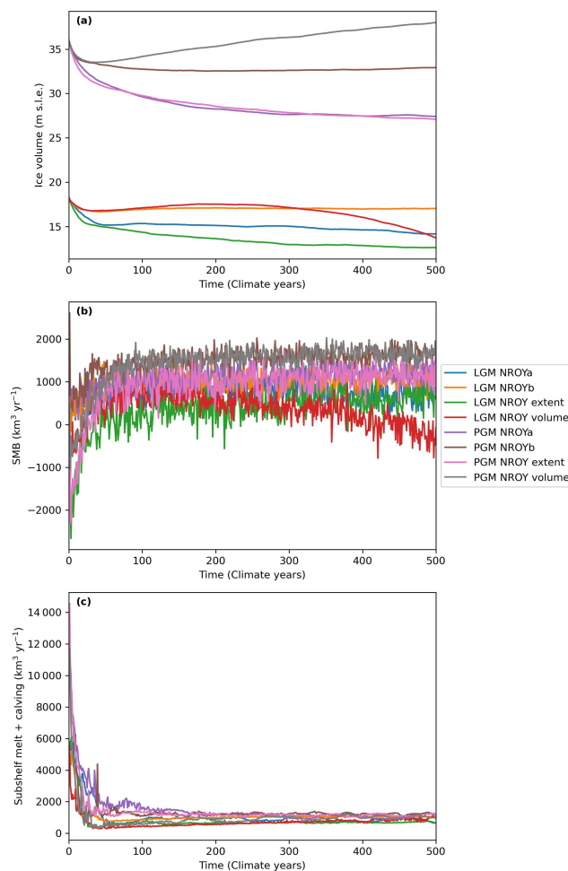
Figure E2. Time series of variables averaged over Eurasia for the NROY simulations; (a) ice volume; (b) surface mass balance; (c) total sub-shelf melt plus calving mass loss; and (d) surface air temperature.
