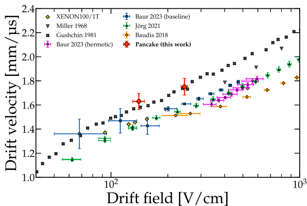
Fig. 19 Field-dependent drift velocities measured in PANCAKE (red). Considering the spread typically attributed to differing LXe temperatures, the results agree with previous measurements [26–32]
