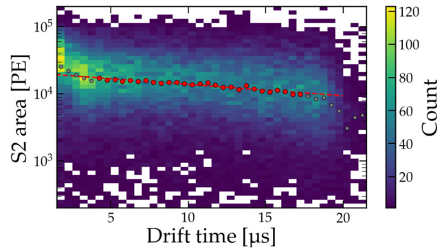
Fig. 18 S2 area vs. drift time for a dataset with good Xe purity. The red dots indicate the median S2 area of all signals per drift time bin which are described by an exponential decay function (red line). Low drift times are excluded from the fit (grey dots) since the region is affected by the higher extraction field above the gate electrode. The fit yields an electron lifetime of \tau_e = (25.6 \pm 1.5) \mu s
