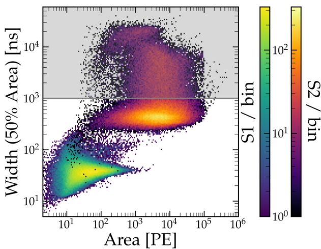
Fig. 14 Distribution of signal width vs. area from S1 and S2 peaks from paired events. Events with S2 widths above 1 \mu\text{s} are rejected from the final event selection (gray area)
