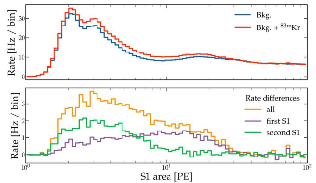
Fig. 12 Top: signal spectrum of all S1 events within time differences \Delta t < 800 ns. The increase from 83m Kr events is clearly visible. Bottom: the difference spectrum from 83m Kr (orange) is separated into the spectra of the time ordered first (purple) and second (green) S1 peak from the delayed coincidence decay of 32.1 keV and 9.4 keV signals, respectively. The 9.4 keV signal extends down to the S1 threshold of 2 PE
