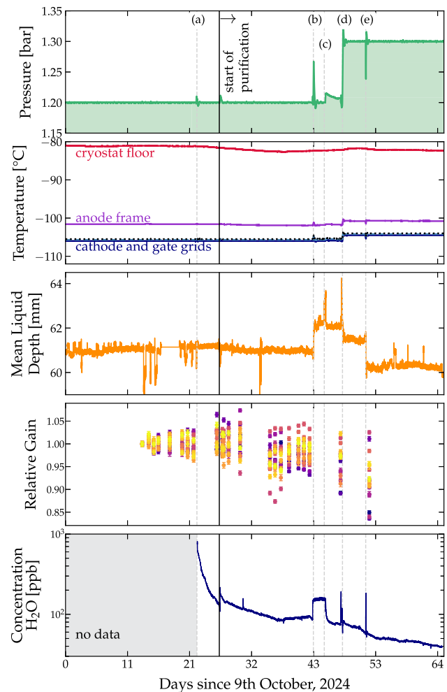
Fig. 8 Operation parameters during the TPC phase. Major operations are indicated by the vertical lines: a test of purification system and HALO+, b filling additional xenon, c power outage, d change operation pressure from 1.2 to 1.3 bar, e recuperation of xenon. The start of the xenon purification is indicated by the solid black line. No Xe purification between b , c . Panel 1 : Xenon gas pressure in the inner cryostat. Two different pressures were set to evaluate the impact. Panel 2 : temperatures measured at the TPC electrodes and the cryostat floor. The cryostat floor was warmer since it was not in direct contact with liquid xenon. Panel 3 : average value of all four levelmeters after detector leveling. Panel 4 : the relative PMT gains normalized to day 1 indicate that the gains were stable within \pm 10\% . The colors represent the different PMTs. Panel 5 : \text{H}_2\text{O} concentration measured with the HALO+ trace gas analyzer
