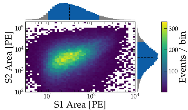
Fig. 15 Distributions of the S1 and S2 signal areas of the final dataset after selection cuts. The median S1 (S2) area is 31 PE (4051 PE) with the central 90 % located between [10, 165] PE for S1s, and [393, 24 137] PE for S2s). Interestingly, the background spectrum in combination with the very position-dependent detector response leads to peak-like distributions
