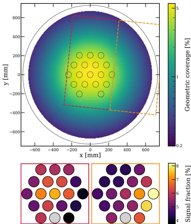
Fig. 10 Top: simulated geometric coverage of positions across the active TPC, averaged over the full LXe depth. The positions covered by the muon telescope are indicated by the colored boxes. The large circle indicates the open-topped vessel. Bottom: average PMT hit patterns generated by muon-induced interactions in the LXe at these positions. The central bottom PMT (omitted or gray) was not used in the analysis
