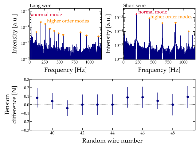
Fig. 7 Top: two frequency spectra for a long and a short wire, respectively, the normal and higher order modes are indicated. Bottom: tension differences for a representative set of wires comparing the tension before and after the operation in liquid xenon. No significant tension change was observed for any of the wires. The nominal tension of these wires was 5.5 N
