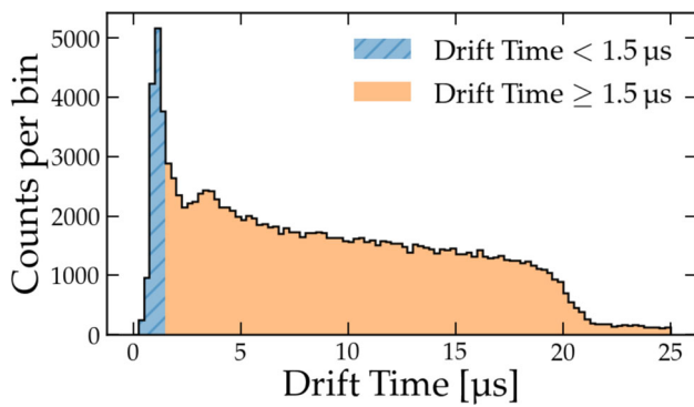
Fig. 13 Electron drift time of events with exactly one S1 and one S2 peak at a drift field of 140(10) V/cm. A cut is applied to remove events with drift times below 1.5 \mu\text{s} which are likely to be from gas events or random coincidences. The drop of events around 20 \mu\text{s} is due to the maximal drift time across the TPC
