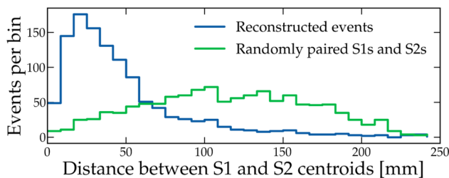
Fig. 17 The distance between the reconstructed S1 and S2 centroid positions for reconstructed events (blue) exhibits significantly smaller separations than that obtained from randomly paired S1 and S2 signals (green). Only events containing exactly one S1 and one S2 are considered. A minimum S1 size of 50 PE is required, and events with saturated channels are excluded to ensure a valid comparison
