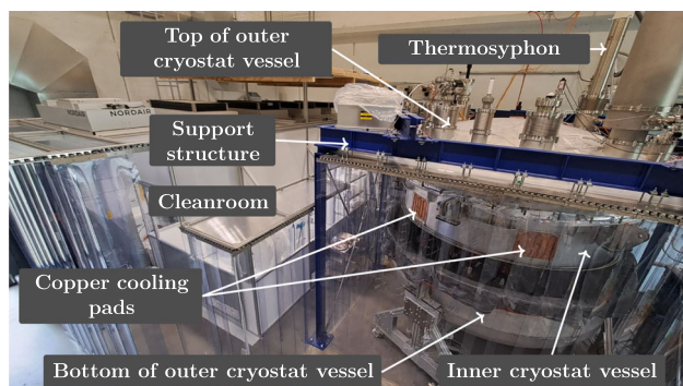
Fig. 1 The PANCAKE facility [13] on the right with its surrounding soft-wall clean area and adjacent cleanroom. The lower outer cryostat vessel was disconnected from its top flange and placed on the floor. The (closed) inner vessel is also visible. The cryostat is suspended from the blue support structure
