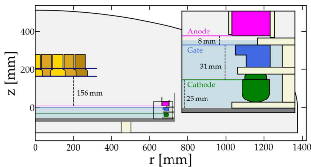
Fig. 2 Schematic side view of the inner cryostat with the installed PMT array (gold) and TPC. The inset depicts the electrode distances; the colored horizontal lines indicate the electrode planes. The uncertainty on the distance between the anode plane and the PMT array is around 10 mm
