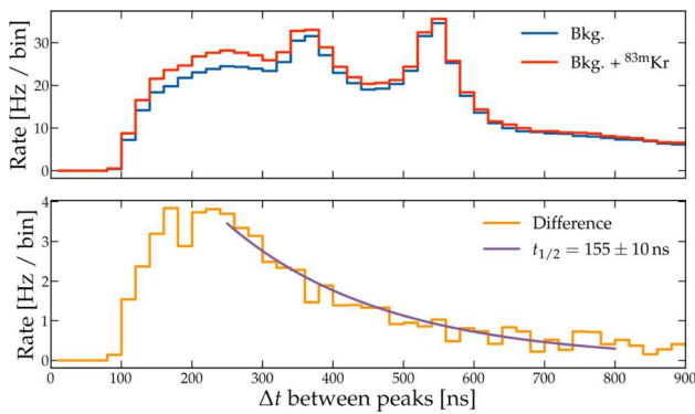
Fig. 11 Top: time differences between consecutive S1 peaks before (blue) and after 83m Kr-injection (red). Bottom: rate difference between both datasets. An exponential fit yields a half-life of 155(10) ns, compatible with the literature value for the decay of the intermediate 83m Kr state
