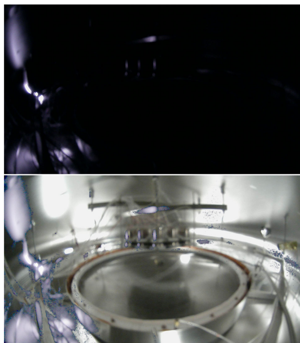
Fig. 9 Top: the camera image shows large light emission for very high cathode voltages. Bottom: overlaying the top (dark) image onto an illuminated reference image reveals that the light was emitted along the high voltage cable connected to the cathode and coiled up in the Xe gas phase (left). Reflections at the PMT array (top center) and the cryostat floor (bottom left) can also be seen. This indicates that the voltage range in this run was limited by the cable
