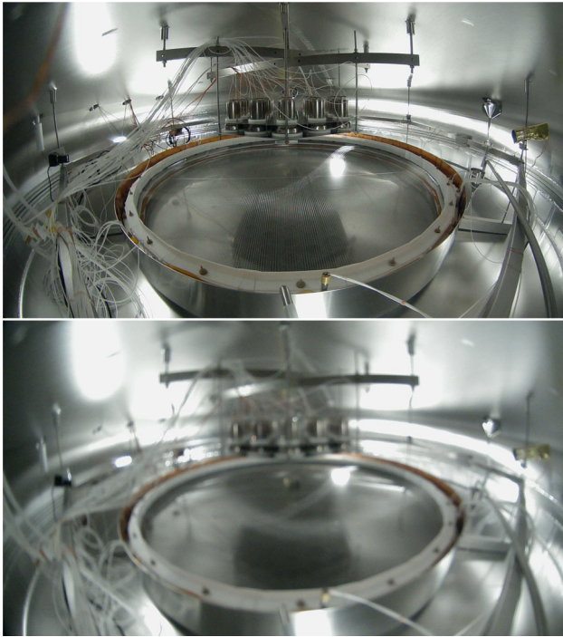
Fig. 5 Inner cryostat illuminated by the internal LEDs. The images were captured by the overview camera when the cryostat was at room temperature (top) and when it was cold and filled with liquid xenon (bottom). The images show that the camera loses focus when being cold. This is likely due to thermal shrinkage and is reverted once the camera is at room temperature again
