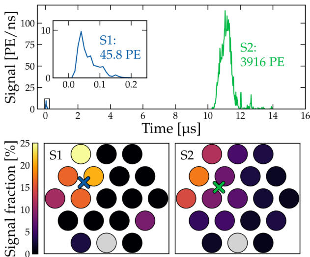
Fig. 16 Example of a typical waveform detected by the TPC. The bottom panel shows the distribution of the S1 and S2 signals across the PMTs. The almost identical location of the distribution's centroids (crosses) indicate a common position in the x - y -plane, as expected for a properly reconstructed event
