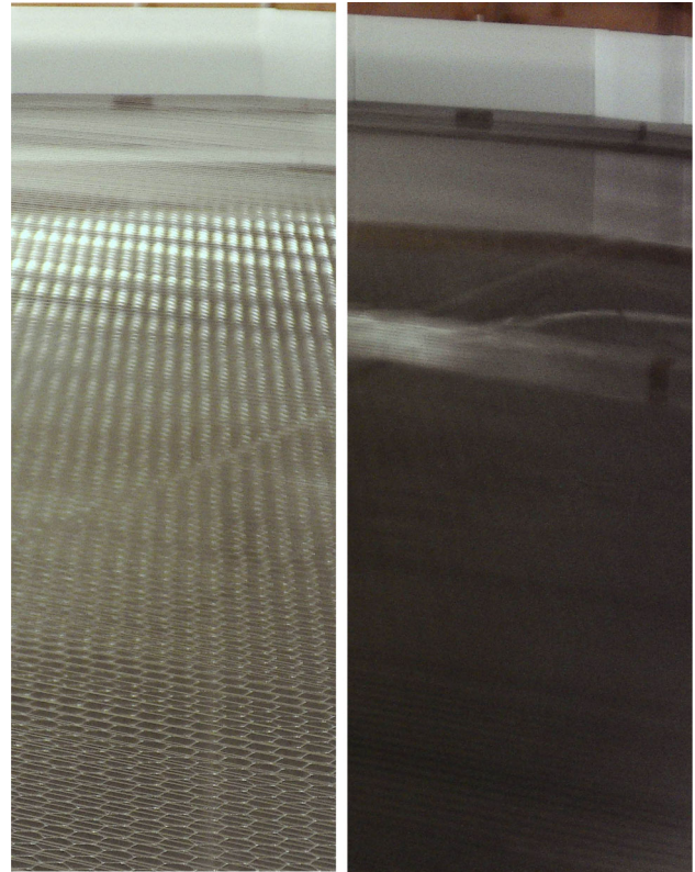
Fig. 6 Two images of the grid camera taken at cryogenic temperatures. The increasing LXe level from the left to the right image obstructs the view onto the hexagonal cathode mesh. Individual electrode wires, as well as the weld seam on the cathode running from the bottom left corner to the top right corner across both images, can be resolved
