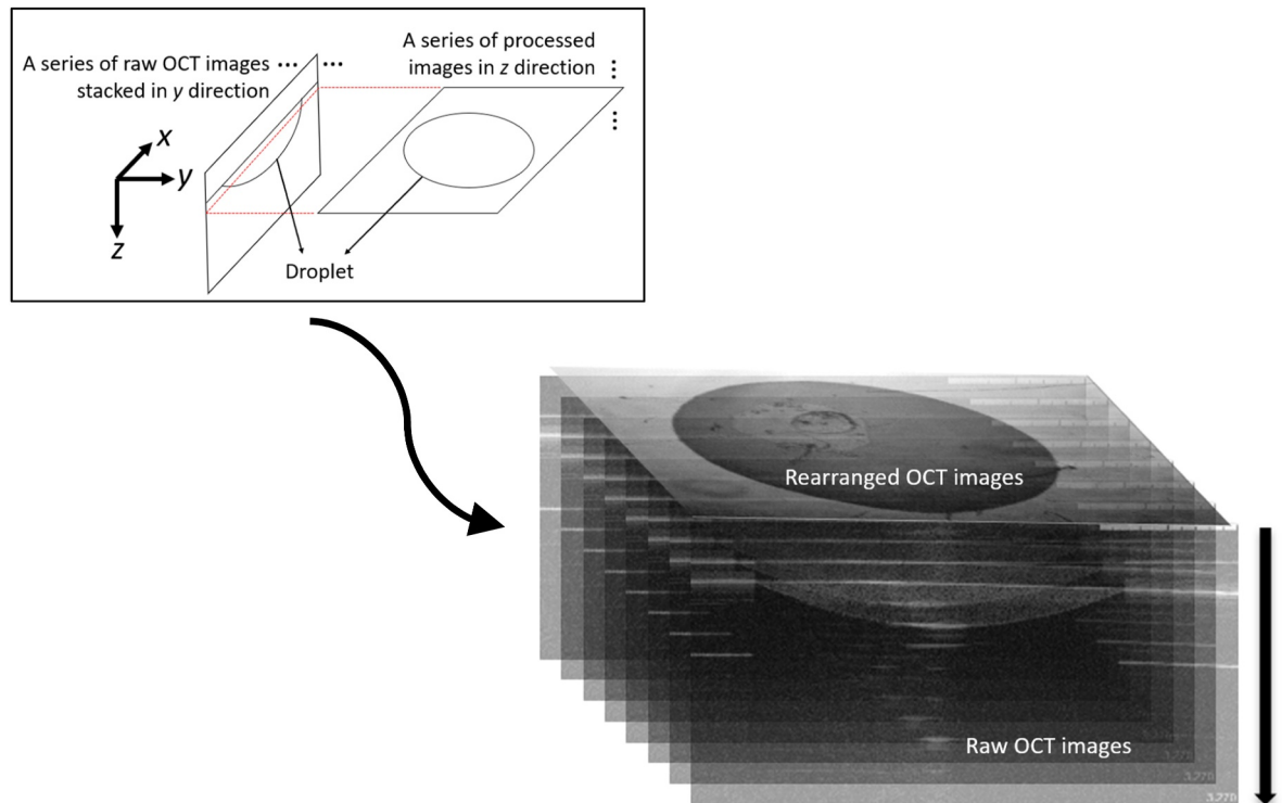
FIGURE 2 | Stacked raw OCT images and rearranged image.
