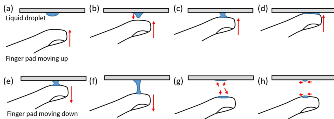
FIGURE 8 | The evolution of the transfer mechanism of the liquid droplet (stages [a–h] illustrate the droplet behavior as the finger approaches, contacts and then retracted from the surface and how the liquid splits between the finger and counterface).
