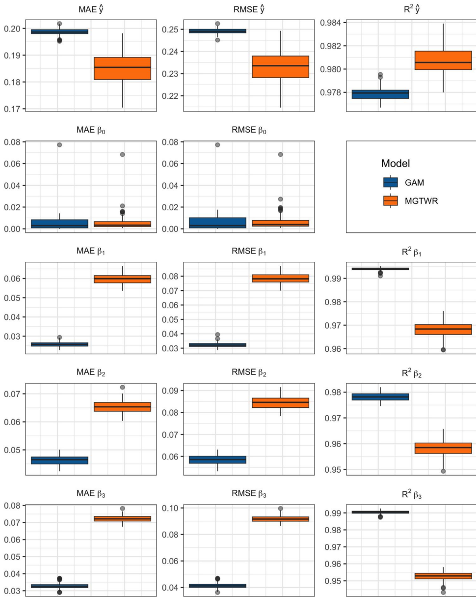
Figure 4. Distributions of model diagnostics (MAE, RMSE and R^2 ) for predicting the true response y and estimating the true coefficients ( \beta_0, \beta_1, \beta_2, \beta_3 ) for the 100 GAMs and 100 MGTWR models.
