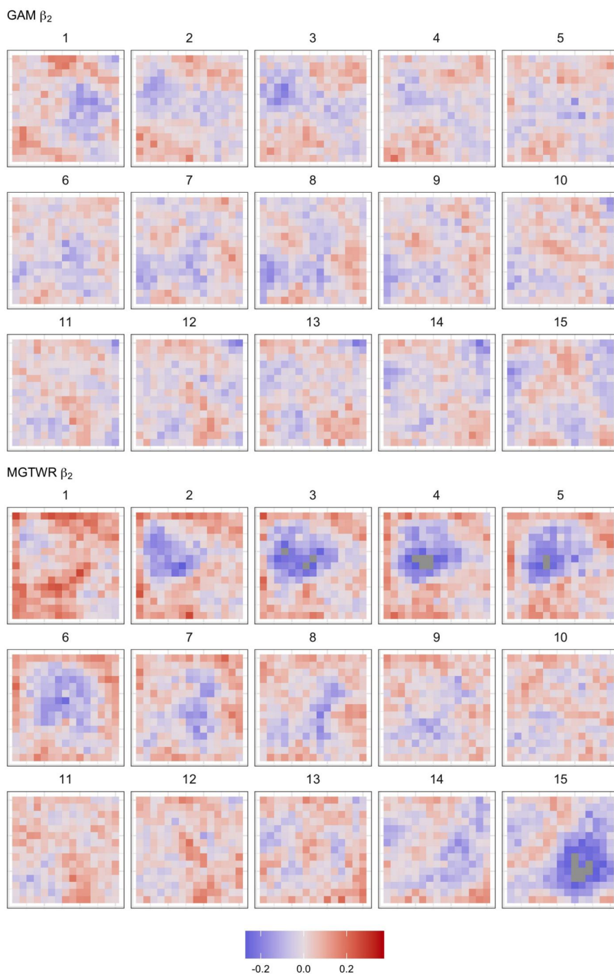
Figure A2. Difference between the GAM (top) and MGTTWR (bottom) estimated coefficients and the true \beta_2 coefficients.
