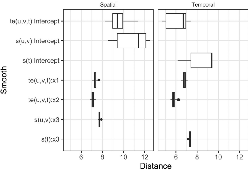
Figure 5. The distributions of the estimated GAM smooth spatial and temporal length ranges across 100 simulated datasets.
