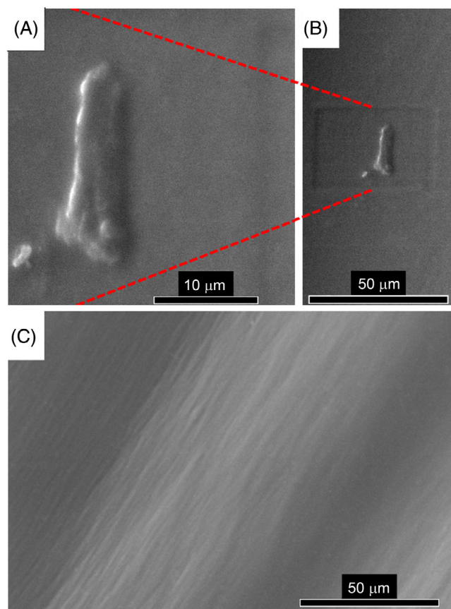
FIGURE 8 ESEM imaging of hydrated collagen hydrogel. (A, B) Surface features were poorly resolved and could not be identified at environmental pressure. (C) As pressure was reduced to 100 Pa striated features appeared on the gel surface. Firm confirmation of these features as the underlying collagen fibre network was not achieved due to the limits of resolving higher magnification images under this mode.
