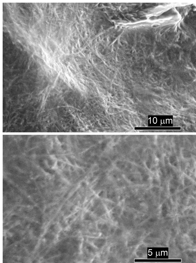
FIGURE 7 ESEM imaging of dehydrated collagen films. Collagen fibres were readily identified; however, identification of constituent fibrils was obscured. Under gaseous secondary ion detection pore spaces between fibres could not be determined.
