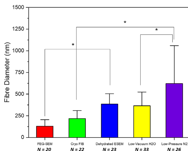
FIGURE 4 Comparison of average fibre diameters under SEM imaging conditions. Imaging of dehydrated films conditions and of cryogenically handled hydrated gels under vacuum conditions produced no significant difference in fibre diameter. Similarly imaging of dehydrated films under environmental pressure and hydrated gels under low-vacuum water vapour atmosphere did not produce significantly different fibre diameters. Fibre diameters under nitrogen low-vacuum atmosphere were significantly larger; however, this was the result of a large aggregation of fibres within a complex 3D network not visible under water vapour imaging.
