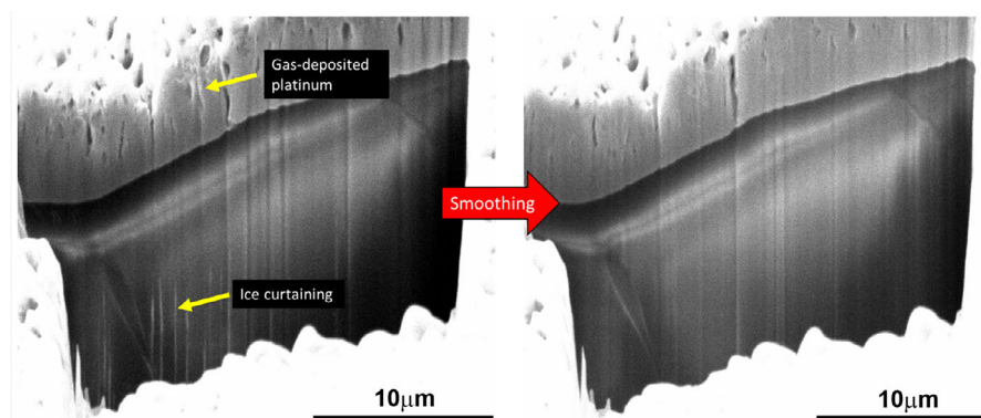
FIGURE 5 Preparation of cryogenic hydrated collagen gels for SEM imaging. Platinum is deposited onto the sample surface by gas injection. A focused ion beam is applied to excavate an exploratory trench. The surface of the revealed ice face is smoothed by further low-intensity milling to reduce ice curtaining generated by differences in the thickness of the deposited platinum layer across the gel surface.
