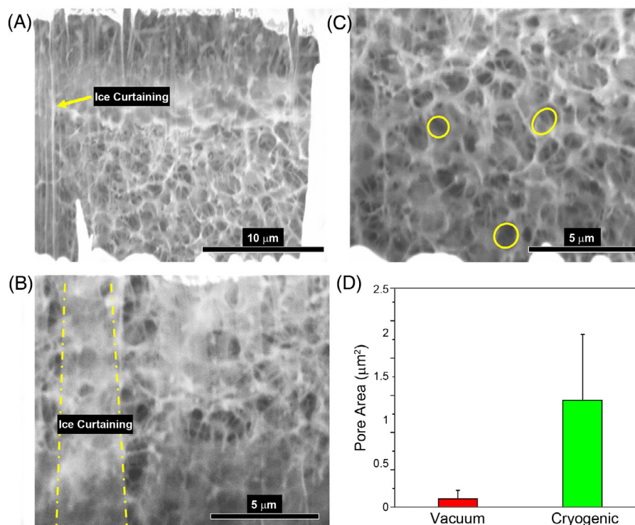
FIGURE 6 Sublimation of cryogenically handled hydrated collagen gels revealed a 3D network of fibres with large area pores. (A, B) Ice curtaining was visible in many milled trenches due to the irregular gas-deposited platinum coating. (C, D) Pores (yellow circles) were found to be of significantly larger dimensions in hydrated gels compared to those ambiently dehydrated and observed under vacuum.
