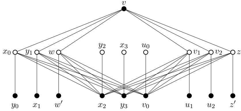
Figure 6: Forbidden Patterns
