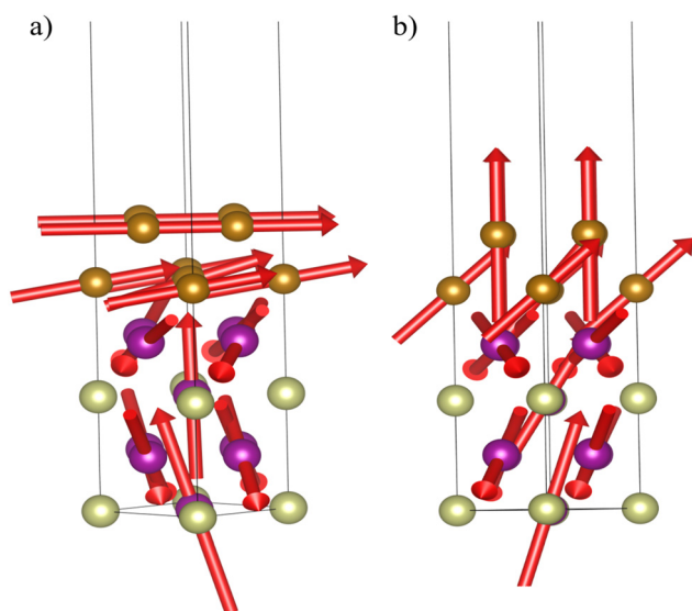
Fig. 5 Magnetic structures for the (a) easy and (b) hard magnetic configurations for Fe on the Mn-rich [100] Ir–Mn surface. Note the easy configuration most closely preserves the magnetic ordering in both the ferromagnetic Fe layer and the antiferromagnetic IrMn layer.
