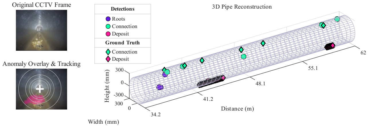
Fig. 4: Full system output: 3D semantic reconstruction of a 28 metre sewer segment.
