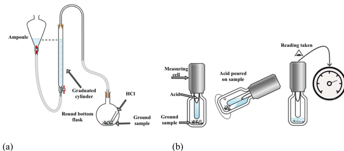
Fig. 6 a Bernard calcimeter, adapted from ([85, 86, 88]; b carbonate bomb (adapted from [87])
