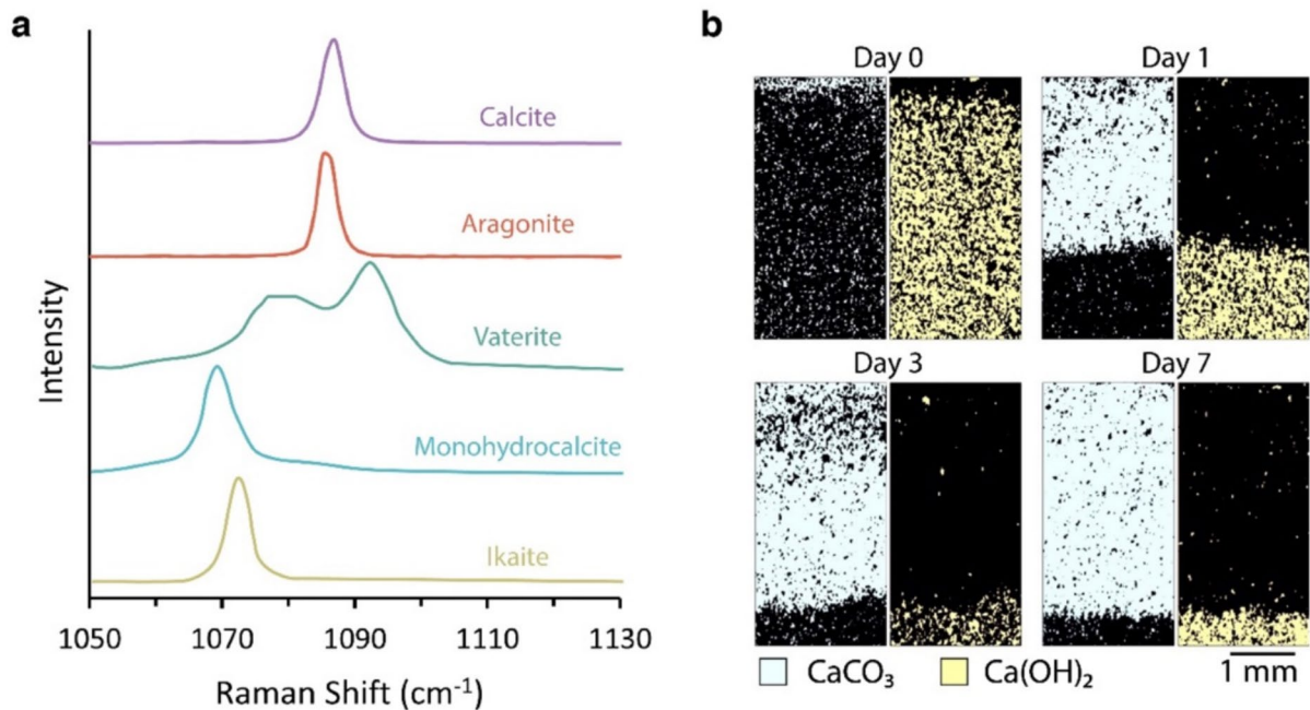
Fig. 4 a Raman spectra of different \text{CaCO}_3 phases, calcite aragonite, vaterite, monohydrocalcite, and ikaite (adapted from [54]); b Raman phase maps ( 1.8 \times 3.6 \text{ mm} ) of calcite and port-
