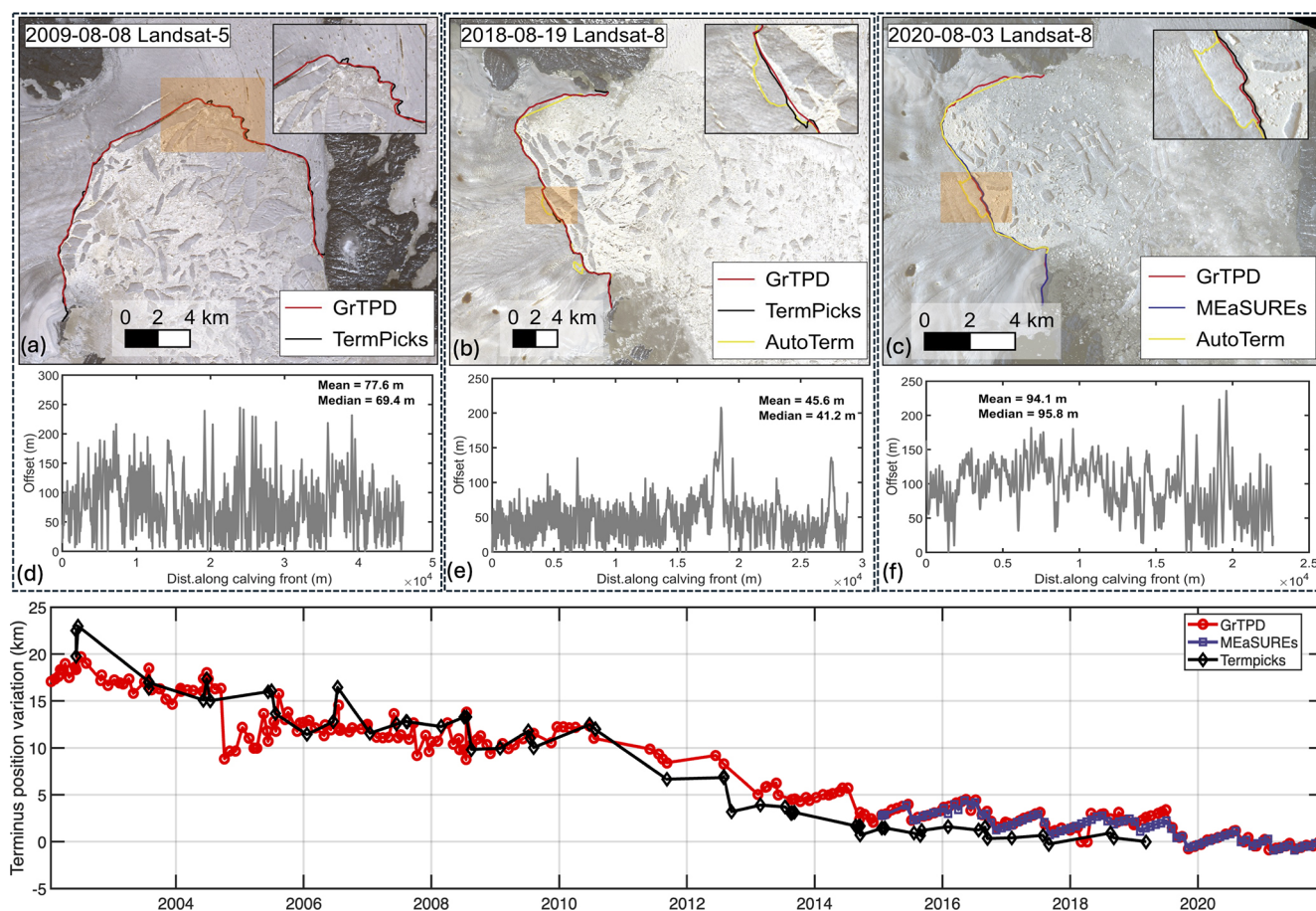
Figure 6. Multi-temporal assessment of Zachariae Isstrøm calving front positions on 8 August 2009, 19 August 2018 and 3 August 2020. (a)–(c) overlay GrTPD (red) with TermPicks (black), AutoTerm (yellow) and MEaSURES (blue) on Landsat images; zoomed insets show areas of high morphological complexity. Panels (d)–(f) illustrate along-front offset profiles for each date. (d) and (e) show comparisons between this dataset and TermPicks, corresponding to (a) and (b), respectively. (f) compares this dataset with MEaSURES, corresponding to (c). Each profile displays both the average and median offsets. (g) presents the time series of manually delineated calving front position variation (km) from 2002 through 2021.
