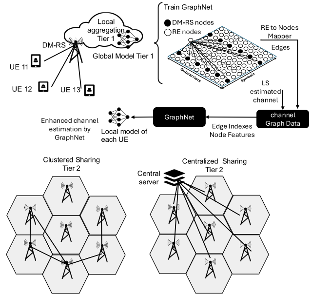
Fig. 6. GraphNet and Two-Tier Federated GraphNet (FGraphNet) for Scalable Channel Estimation in 5G NR. Local channel data are transformed into graph representations and used to train GNN-based channel estimators at each BS (Tier-1). Model updates are then shared across neighboring BSs within a cluster or centrally (Tier-2), enabling collaborative and adaptive channel estimation under heterogeneous network conditions.
