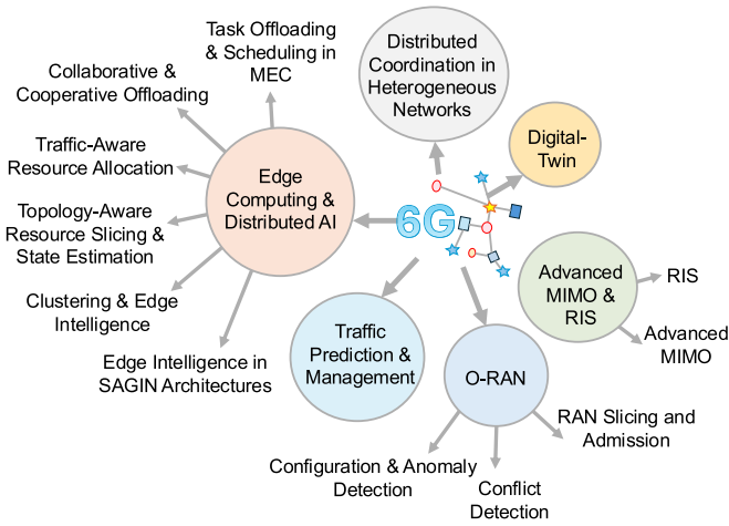
Fig. 5. AI-GNNs Empowering Key 6G Enablers.
