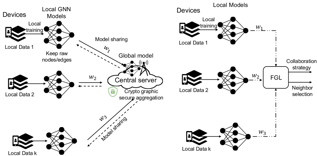
Fig. 4. Synergy between FL and GNNs. GNNs operate either as local, structure-aware models within federated learning or as coordination layers that adapt communication topology and collaboration strategies to optimize latency, energy efficiency, and task performance.
