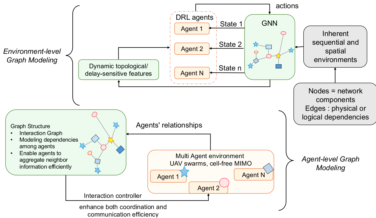
Fig. 3. DRL-GNN synergy: agent-level and environment-level graph modelling perspectives.
