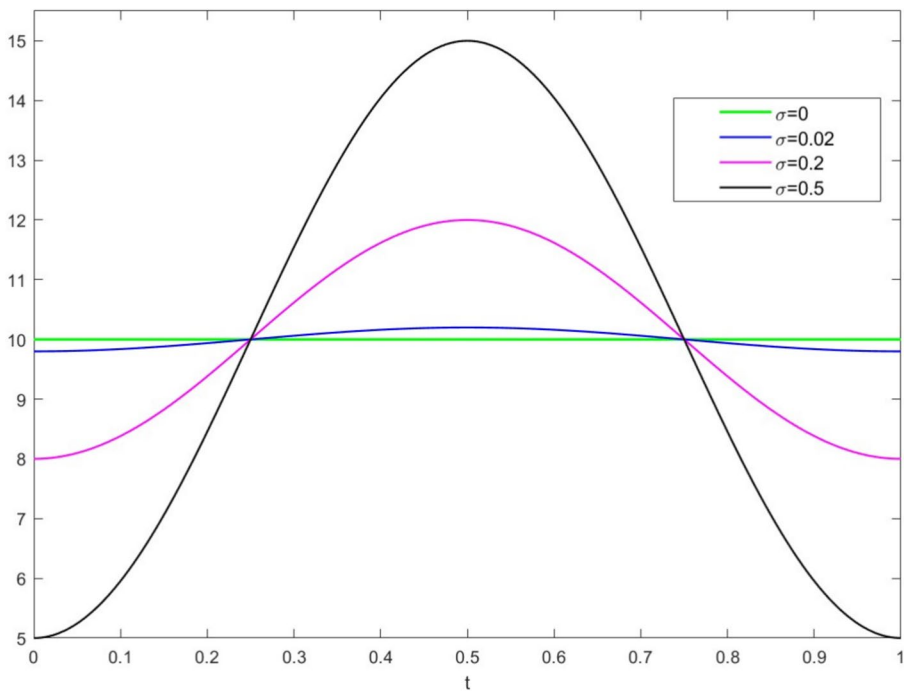
Fig. 6 The time-varying reproduction number R_0(t) as a function of t in the standard SIR model and SIR models with time-varying contact rates, for a scenario with N = 100
