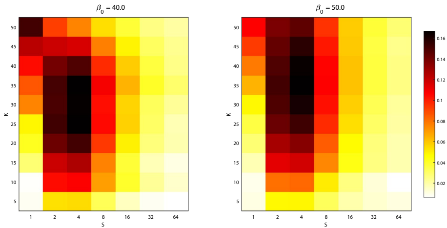
Fig. 1 The Hellinger distance H(\mathcal{P}(K), \mathcal{P}_S(K)) as a function of S , in scenarios with \beta_0 = 40.0 (left) and 50.0 (right) and \alpha = 2.0 , for congestion levels K ranging between 5 and 50
