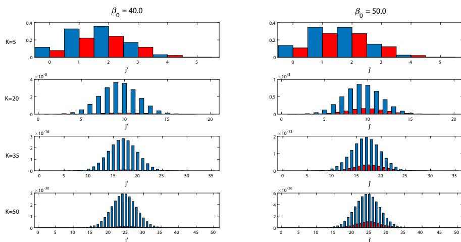
Fig. 5 Erlangian approximations \{F_S(24|1, 0; K, j') : j' \in \{0, \dots, K\}\} (histogram in blue) and \{G_S(24|1, 0; K, j') : j' \in \{0, \dots, K\}\} (histogram in red) in a scenario with \beta_0 = 40.0 and \alpha = 24.0 , for K \in \{5, 20, 35, 50\}
