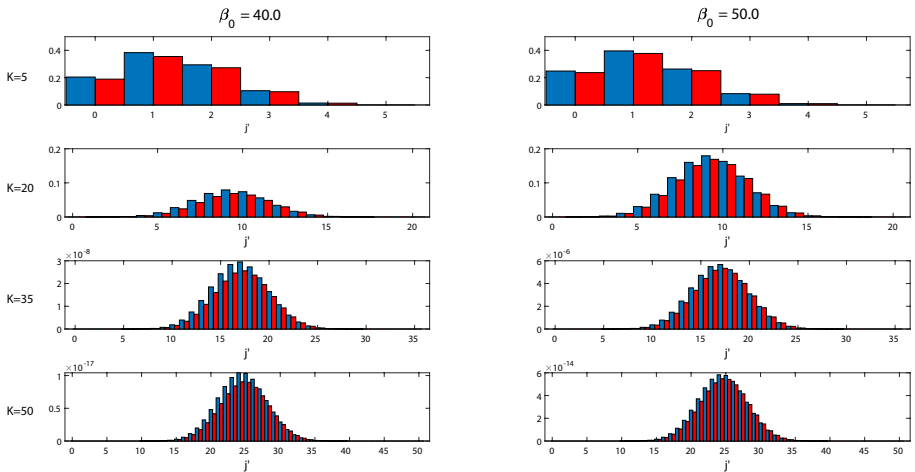
Fig. 4 Erlangian approximations \{F_S(24|1, 0; K, j') : j' \in \{0, \dots, K\}\} (histogram in blue) and \{G_S(24|1, 0; K, j') : j' \in \{0, \dots, K\}\} (histogram in red) in a scenario with \beta_0 = 40.0 and \alpha = 12.0 , for K \in \{5, 20, 35, 50\}
