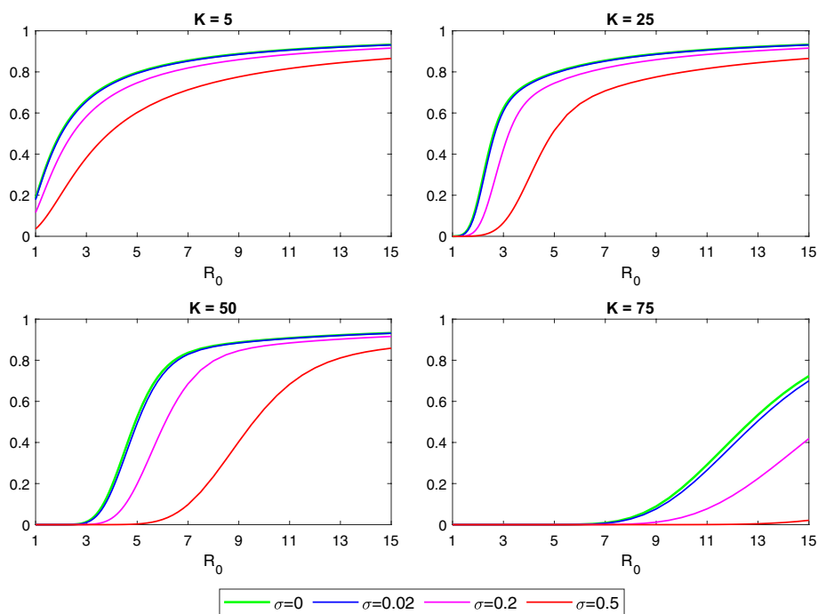
Fig. 7 The Erlangian approximation of probability P(\eta_K \leq T \mid (I(0), J(0)) = (1, 99)) as a function of R_0 in the standard SIR model and SIR models with time-varying contact rates, for T = 1 , K \in \{5, 25, 50, 75\} and a scenario with N = 100
