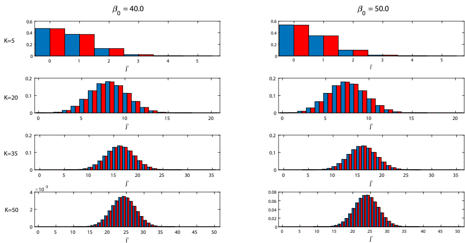
Fig. 3 Erlangian approximations \{F_S(24|1, 0; K, j') : j' \in \{0, \dots, K\}\} (histogram in blue) and \{G_S(24|1, 0; K, j') : j' \in \{0, \dots, K\}\} (histogram in red) in a scenario with \beta_0 = 40.0 and \alpha = 4.0 , for K \in \{5, 20, 35, 50\}
