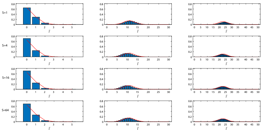
Fig. 2 The solution \mathcal{P}(K) (solid line in red) versus its Erlangian approximation \mathcal{P}_S(K) (histogram in blue) in a scenario with \beta_0 = 40.0 and \alpha = 2.0 , for congestion levels K = 5, 30 and 50 (from left to right)
