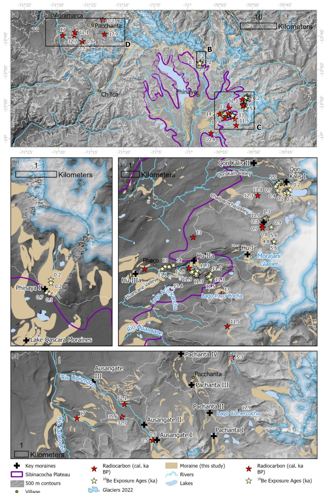
FIGURE 3 Published chronology from the Cordillera Vilcanota area. Radiocarbon ages (Goodman et al., 2001; Mark et al., 2002; Mercer & Palacios, 1977) are recalibrated using the Calib version 8.20 14 C calibration programme (Stuiver & Reimer, 1993), and are presented as calibrated ages (cal. ka BP), using the IntCal20 dataset (Reimer et al., 2020). Published cosmogenic nuclide ages (Kelly et al., 2015; Sagredo et al., 2016; Stroup et al., 2014, 2015) are recalculated using the LSDn scaling scheme (Borchers et al., 2016; Lifton et al., 2014) and the global production rate (Borchers et al., 2016).
