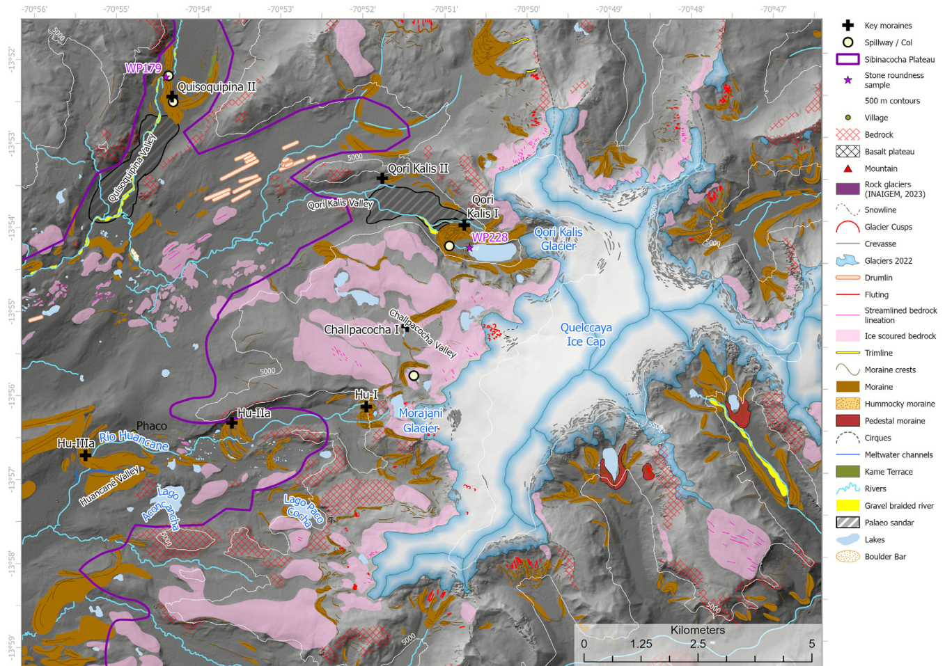
FIGURE 9 Quelccaya Ice Cap glaciology and geomorphology.
