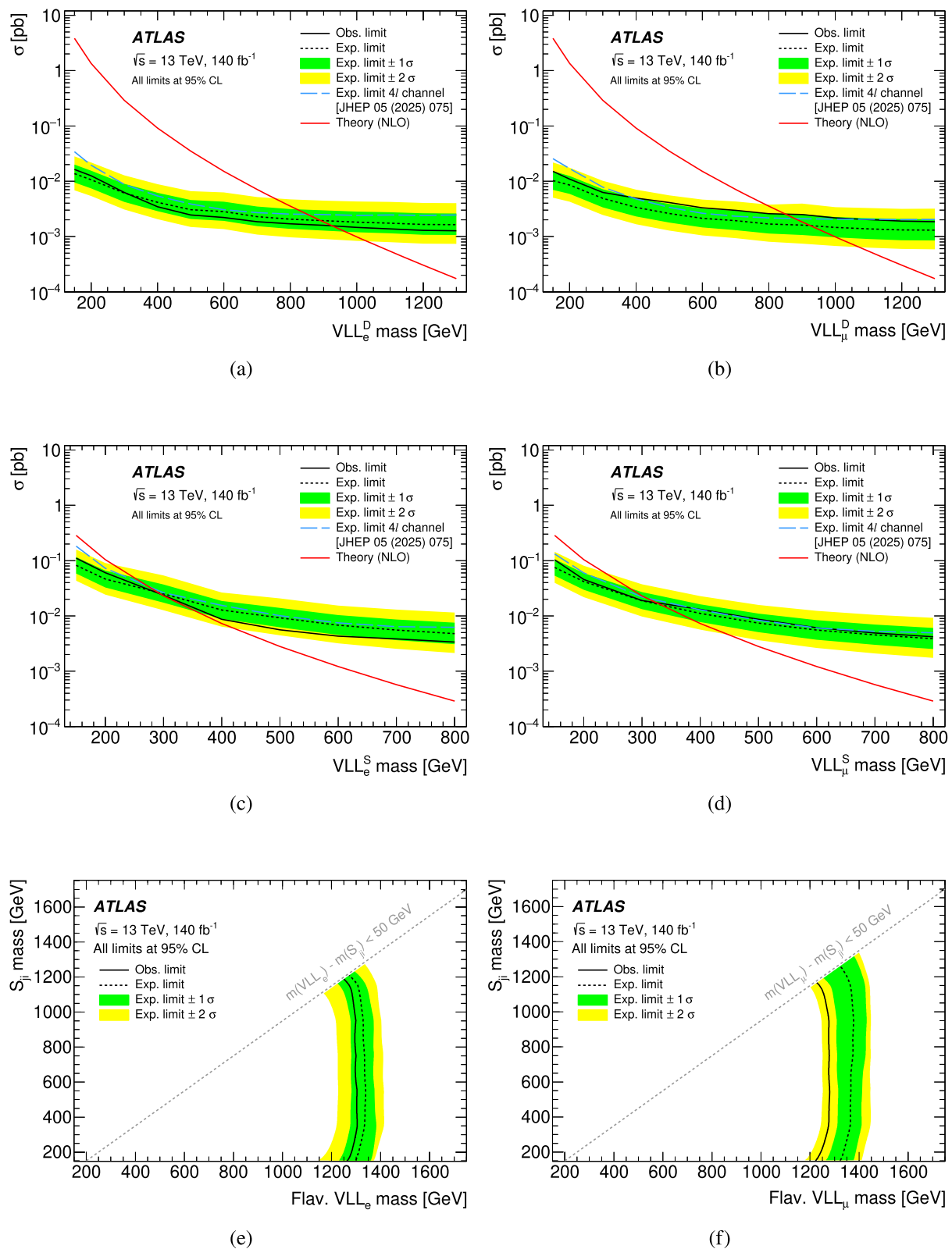
Fig. 10 Combined observed and expected limits at 95% CL on the cross-section ( \sigma ) as a function of the VLL mass for the a \text{VLL}_e^D , b \text{VLL}_\mu^D , c \text{VLL}_e^S , d \text{VLL}_\mu^S models, and on the plane of the S_{ji} mass versus the VLL mass for the e flavourful \text{VLL}_e , and f flavourful \text{VLL}_\mu
