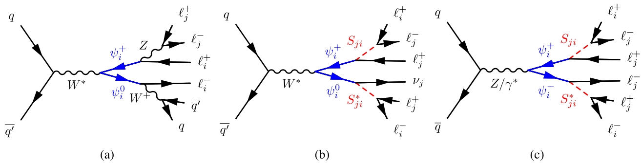
Fig. 1 Example Feynman diagram for the pair production of VLL, denoted by \psi_i , in the flavourful model, with the VLLs produced via a , b W^* boson and c a Z boson, with the decay of the VLLs into SM leptons and a two SM vector bosons, and b , c two scalars S_{ji} .
