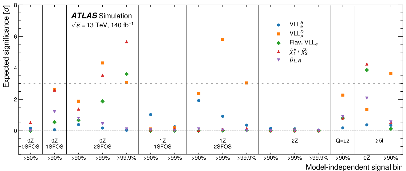
Fig. 8 Expected significance in the model-independent regions to the benchmark signal models: VLL_e^S with a mass of 200 GeV, VLL_\mu^D with a mass of 600 GeV, flavourful VLL_e with a mass of 1200 GeV and a scalar S mass of 550 GeV, wino-like chargino with a mass of 1300 GeV and a neutralino mass of 800 GeV, and smuon with a mass of 350 GeV
