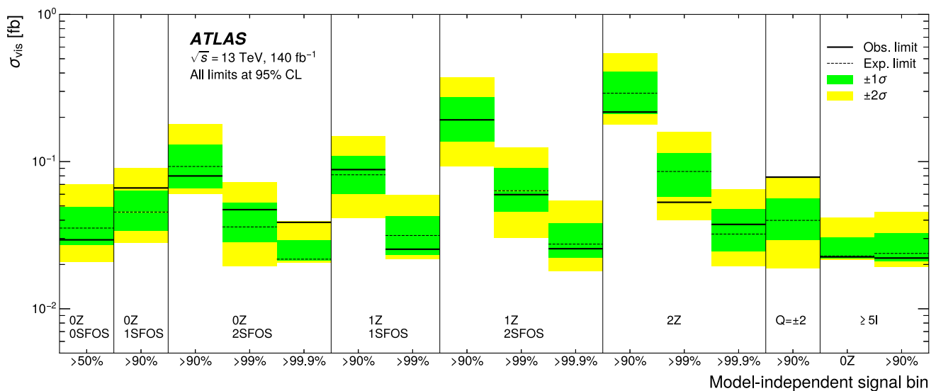
Fig. 7 Observed and expected excluded visible cross section limits, \sigma_{\text{vis}} for the model-independent regions. The various requirements on the anomaly score corresponding to the specified background rejection cuts (99.9/99/90/50%) are shown for all regions, except for the \geq 5l 0Z SR, where no AD is applied
