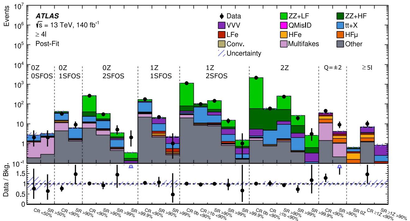
Fig. 6 Comparison between data and the background prediction for the discovery regions included in the model-independent fit, after a background-only fit to data in the five cut-based control regions and ten low-anomaly score discovery regions ('post-fit'). All signal bins are shown ('SR') together with the low-anomaly score discovery regions ('CR'). The various requirements on the anomaly score corresponding to the specified background rejection cuts (99.9/99/90/50%) are shown for all SRs and CRs, except for the \geq 5l 0Z SR, where no AD is
