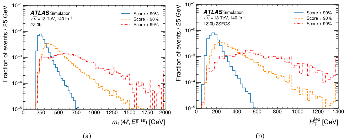
Fig. 2 Comparison of background shapes for a m_T(4\ell, E_T^{\text{miss}}) in the 2Z 0b region and b H_T^{\text{lep}} in the 1Z 0b 2SFOS region, considering various requirements on the anomaly score corresponding to the specified background rejection cuts. The last bin contains the overflow
