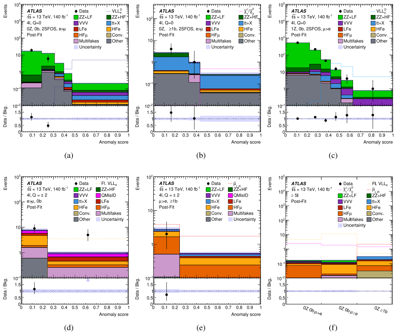
Fig. 9 Comparison between data and the background estimate for the anomaly score distribution used in different benchmark regions, after a background-only fit to data ('post-fit'): a 4\ell Q = 0 0Z 0b 2SFOS e > \mu , b 4\ell Q = 0 0Z \geq 1b 2SFOS e > \mu , c 4\ell Q = 0 1Z 0b 2SFOS \mu > e , d 4\ell Q = \pm 2 0b e > \mu , e 4\ell Q = \pm 2 \geq 1b \mu > e , and f the three \geq 5\ell regions: 0Z 0b \mu > e , 0Z 0b e \geq \mu , and 0Z \geq 1b , defined without AD. Distributions for a VLL_e and VLL_\mu signal point of mass 500 GeV, one flavourful VLL_e signal point for a VLL mass of 1 TeV and scalar of 550 GeV, a wino-like chargino and neutralino signal
