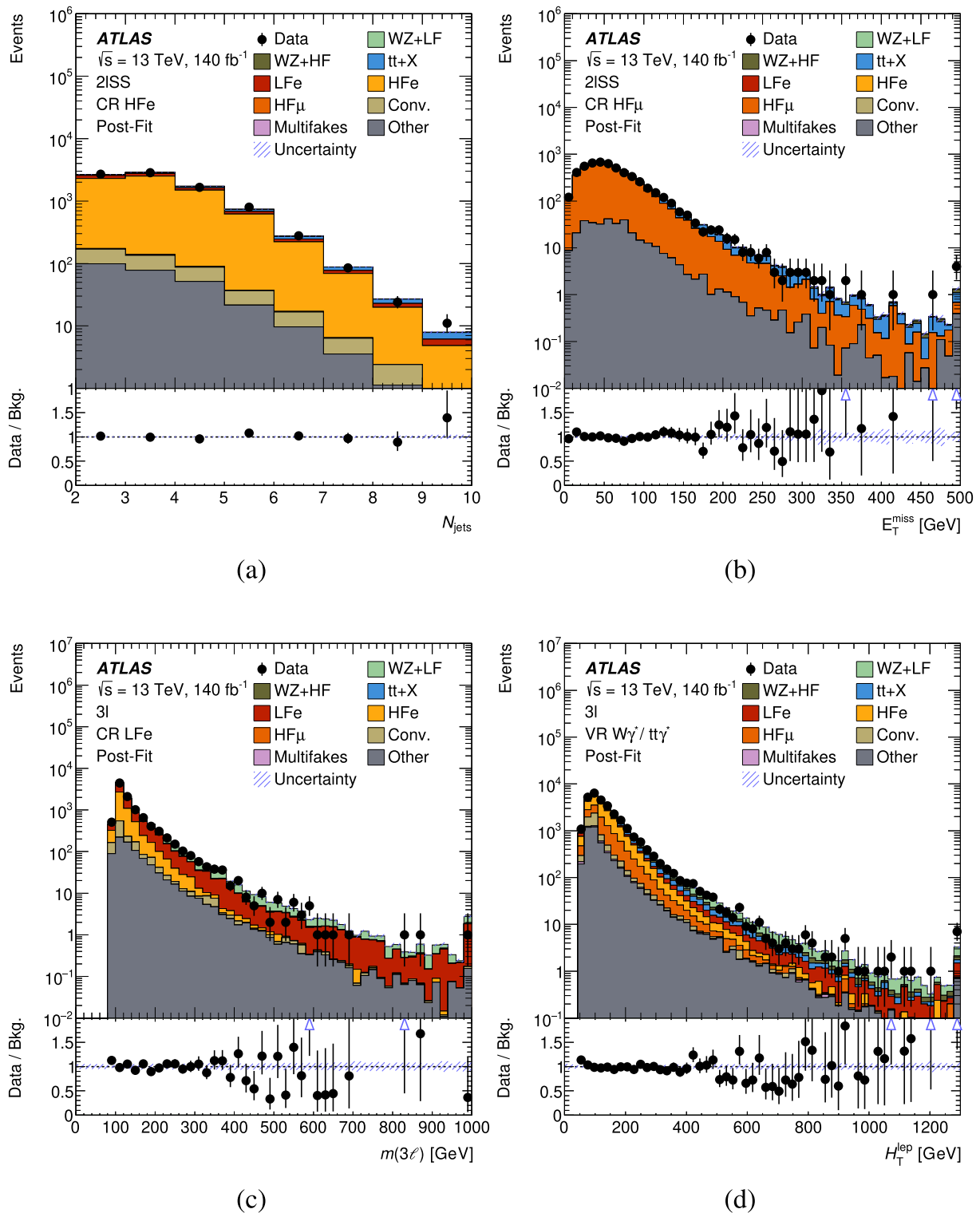
Fig. 5 Comparison between data and the background prediction for the a N_{\text{jets}} , b E_T^{\text{miss}} , c m(3\ell) , and d H_T^{\text{lep}} distribution in the a HFe CR, b HFμ CR, c LFe CR, and d the W\gamma^*/t\bar{t}\gamma^* validation region. The background contributions after the likelihood fit to data ('post-fit') for the background-only hypothesis are shown as filled histograms. The ratio of the data to the background prediction ('Bkg.') is shown in the lower panel. The 'tt+X' background component includes the t\bar{t}H , t\bar{t}Z , and
