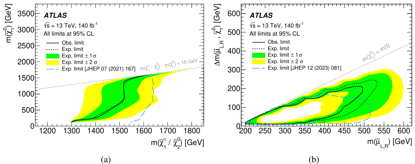
Fig. 11 Combined observed and expected limits at 95% CL for the a wino-like chargino and neutralino, and b smuon models, as a function of the masses of \tilde{\chi}_1^\pm/\tilde{\chi}_2^0 and \tilde{\chi}_1^0 , and \tilde{\mu}_{L,R} and \Delta m(\tilde{\mu}_{L,R}, \tilde{\chi}_1^0) , respectively. The expected limits from the dedicated ATLAS searches [21,22]
