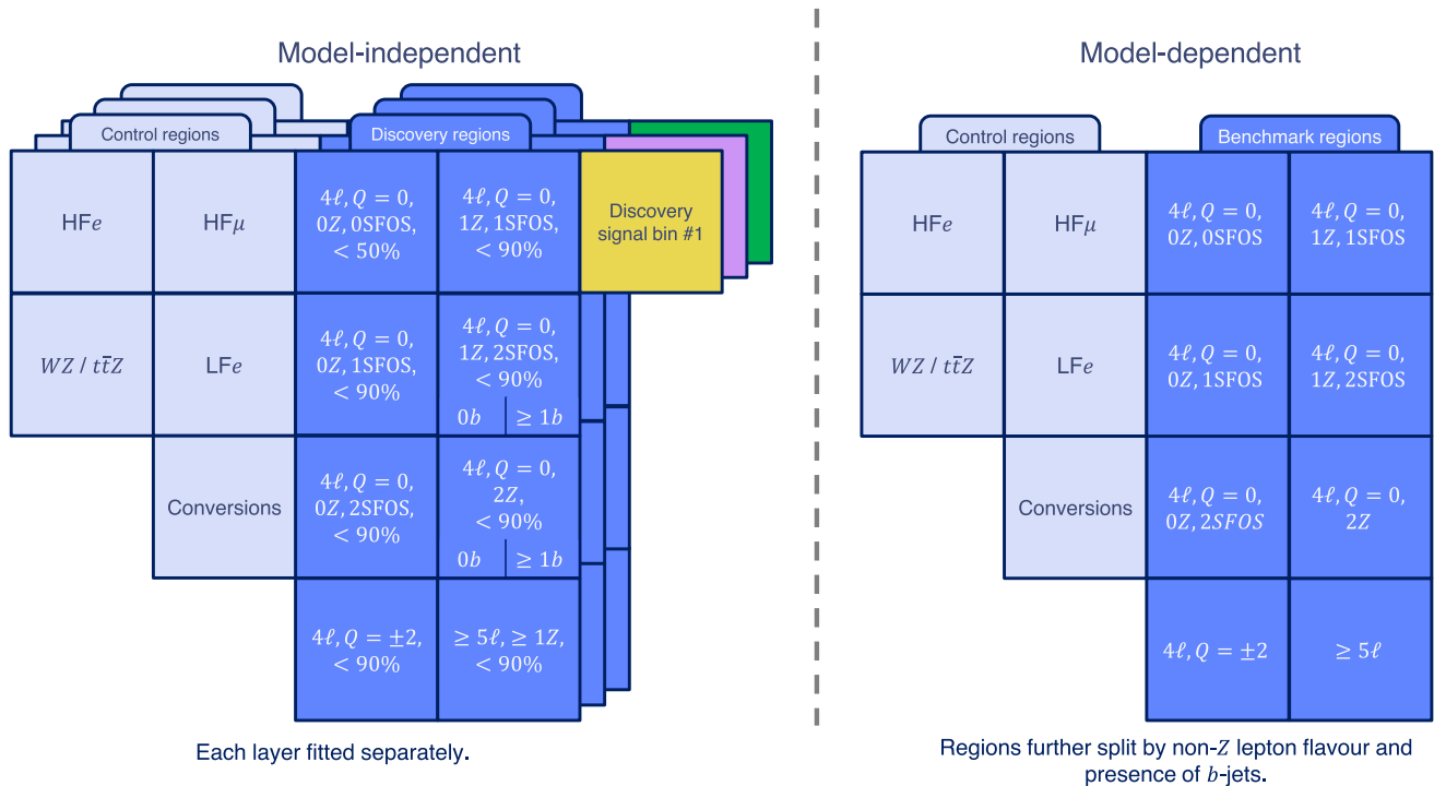
Fig. 3 Illustrative sketch of the control regions and (left) discovery or (right) benchmark regions in the (left) model-independent or (right) model-dependent search. For the model-independent scenario, the discovery regions correspond to low-anomaly score regions fitted together with a high-anomaly score discovery signal bin at a time. Each layer corresponds to the different fits with the same control regions and low-
