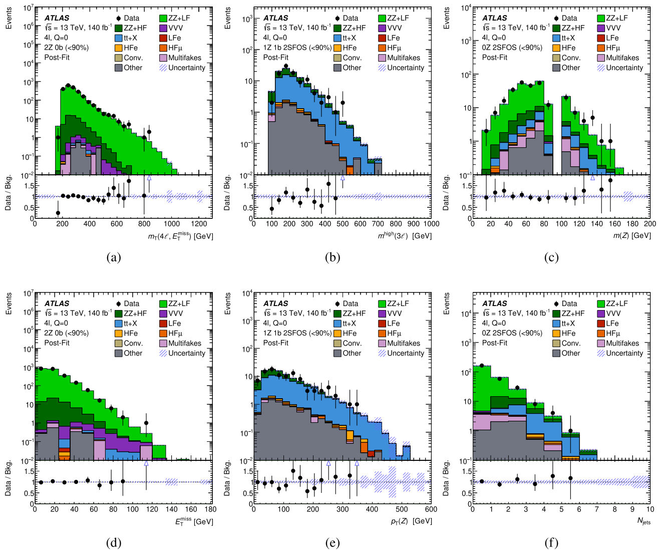
Fig. 4 Comparison between data and the background prediction for the a m_T(4\ell, E_T^{\text{miss}}) , b m^{\text{high}}(3\ell) , c m(Z) , d E_T^{\text{miss}} , e p_T(Z) , and f N_{\text{jets}} distribution in the a , d ZZ 0b, b , e 1Z 1b 2SFOS, and c , f 0Z 2SFOS region, after requiring the anomaly score to be below the 90% background rejection point. The background contributions after the likelihood fit to data ('post-fit') for the background-only hypothesis are shown as filled histograms. The 'tt+X' background component includes the t\bar{t}Z , and t\bar{t}H processes. The 'HF \ell ' ('LF \ell ') background component refers to processes containing one non-prompt light lepton from heavy-flavour
