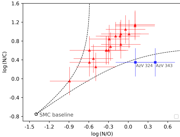
Fig. 7. \log N/C vs \log N/O . The red triangles show the distribution of our sample. The stars for which the oxygen abundance was obtained from fitting the O I \lambda\lambda 7772\text{--}7774\text{--}7775 multiplet are shown in blue squares. The dashed black lines represent the upper and lower boundaries adopted from Maeder et al. (2014).
