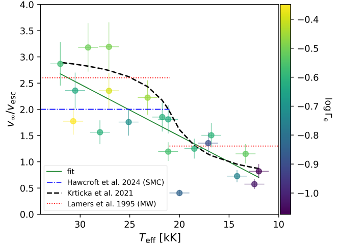
Fig. 13. Ratio ( v_{\infty}/v_{\text{esc}} ) as a function of temperature. The solid green line represents the linear fit to our sample. The dashed black line is the relation presented in Krticka et al. (2021). The dotted red lines represent the ratios from Lamers et al. (1995). The colour gradient correlates with the value of \Gamma_e .
