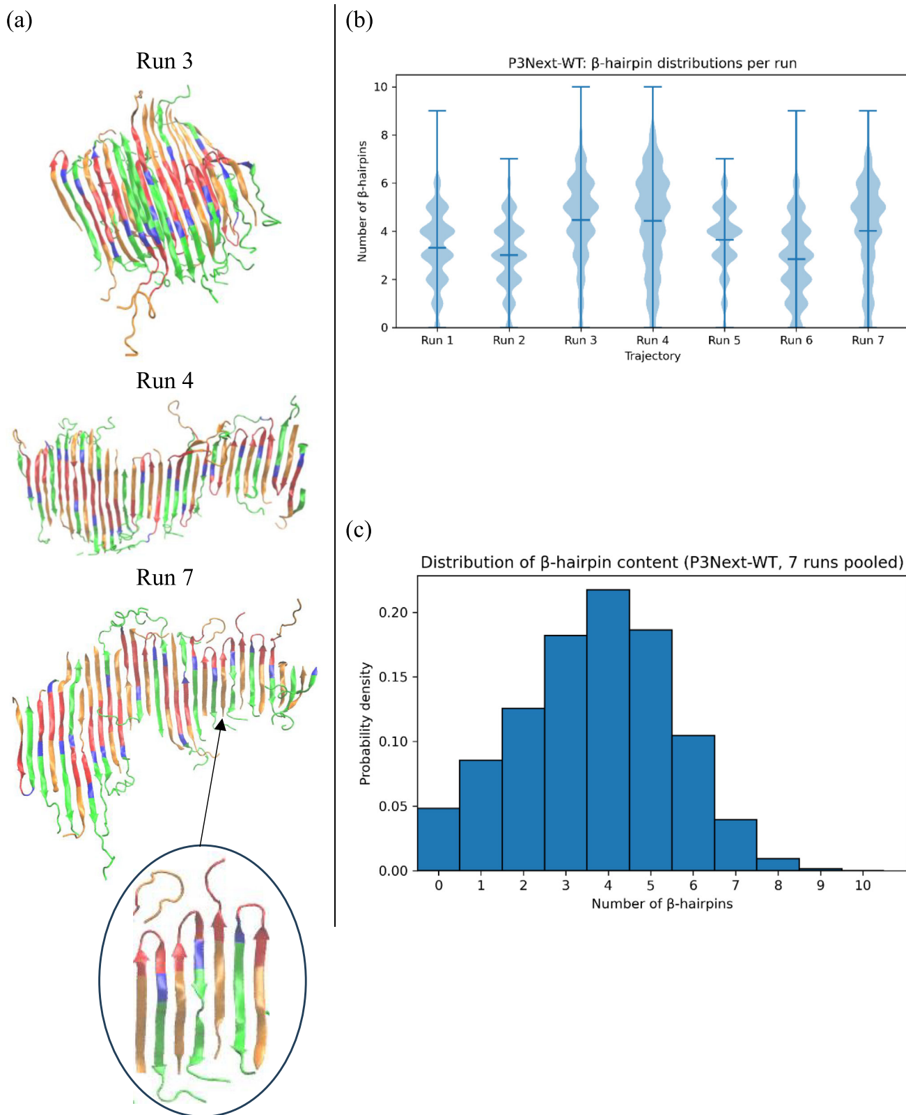
FIGURE 4 Conformational variability and \beta -hairpin statistics of P3Next-WT across seven independent simulations. (a) Snapshots at the ends of the simulations of P3Next-WT fragments reveal that the number of \beta -hairpins varies in the P3Next-WT fibrils. A color code is used to display the position of P1 (red), P2 (green), the in-between residues \alpha Syn [43, 44] (blue), and the additional residues in P3Next compared to P3 (orange). Enlarged section from the snapshot of Run 7 shows \beta -hairpins in the fibril. (b) Distribution of \beta -hairpin content for each of the seven independent P3Next-WT trajectories, shown as violin plots. Each violin displays the full probability density of \beta -hairpin counts during a run, with horizontal bars marking the mean and vertical lines indicating extrema. (c) Pooled histogram of \beta -hairpin content across all frames from all seven WT trajectories shows that distribution is centered around 3–5 \beta -hairpins.
