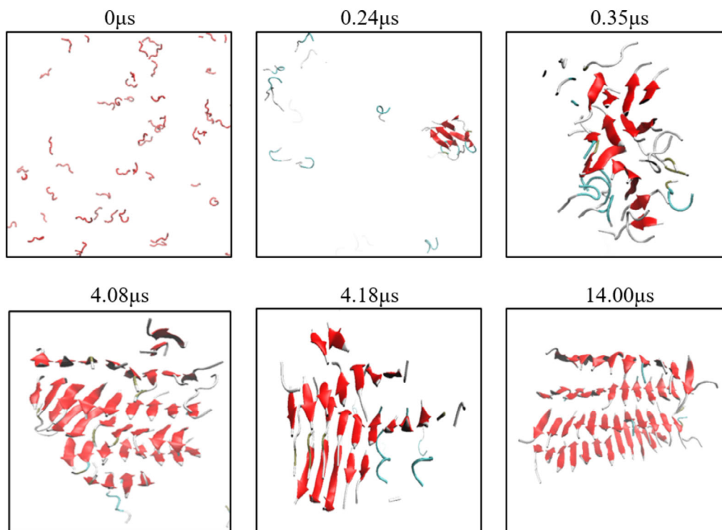
FIGURE 2 Snapshots at different times during the early stage of fibril formation of P1-WT fragments from one simulation. See also Supplementary Movie 1.
