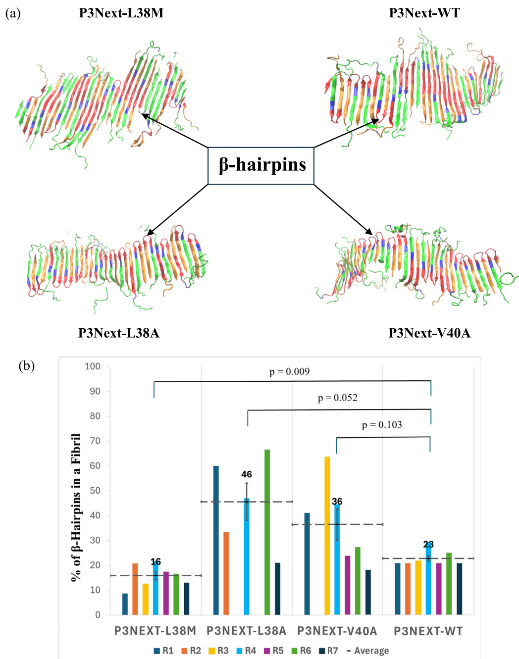
FIGURE 6 (a) Snapshot of \beta -hairpin formation in all P3Next variant fibrils. (b) The percentage of \beta -hairpins formed in each fibril. The average percentage of \beta -hairpins in P3Next-L38M fibril is less than in the fibrils of the other variants. P3Next-WT and L38M aggregated in all seven runs, L38A and V40A did not aggregate in all simulations. The dashed lines and the numbers above them indicate the average percentage of \beta -hairpins formed by each variant. The figure also displays probability values indicating statistical significance at the top.
