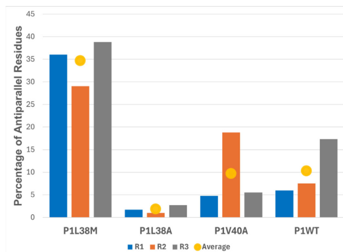
FIGURE 5 (a) Snapshots of final configurations of P1 peptide simulations with the sequence substitutions L38M, L38A, or V40A, as well as the wild-type P1 (P1-WT). Although all four sequences formed multi-layer fibrils, the number of parallel and antiparallel \beta -strands are different. Each fibril is shown from two different angles through separate snapshots. (b) Average percentage of antiparallel residues within a fibril.
