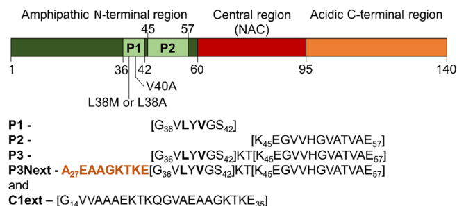
FIGURE 1 \alpha Syn regions and the peptide fragments that were simulated herein. The amphipathic N-terminal (green) contains residues \alpha Syn[1–60]. The central non-amyloid component (NAC) region (red) contains residues \alpha Syn[61–95]. The acidic C-terminal region (orange) covers the last 45 residues. P1 and P2 are short motifs in the N-terminal region (light green). The sequences of P1, P2, P3, P3Next, and C1ext are listed. Note the charges on the termini are blocked in the simulation (see Methods).
