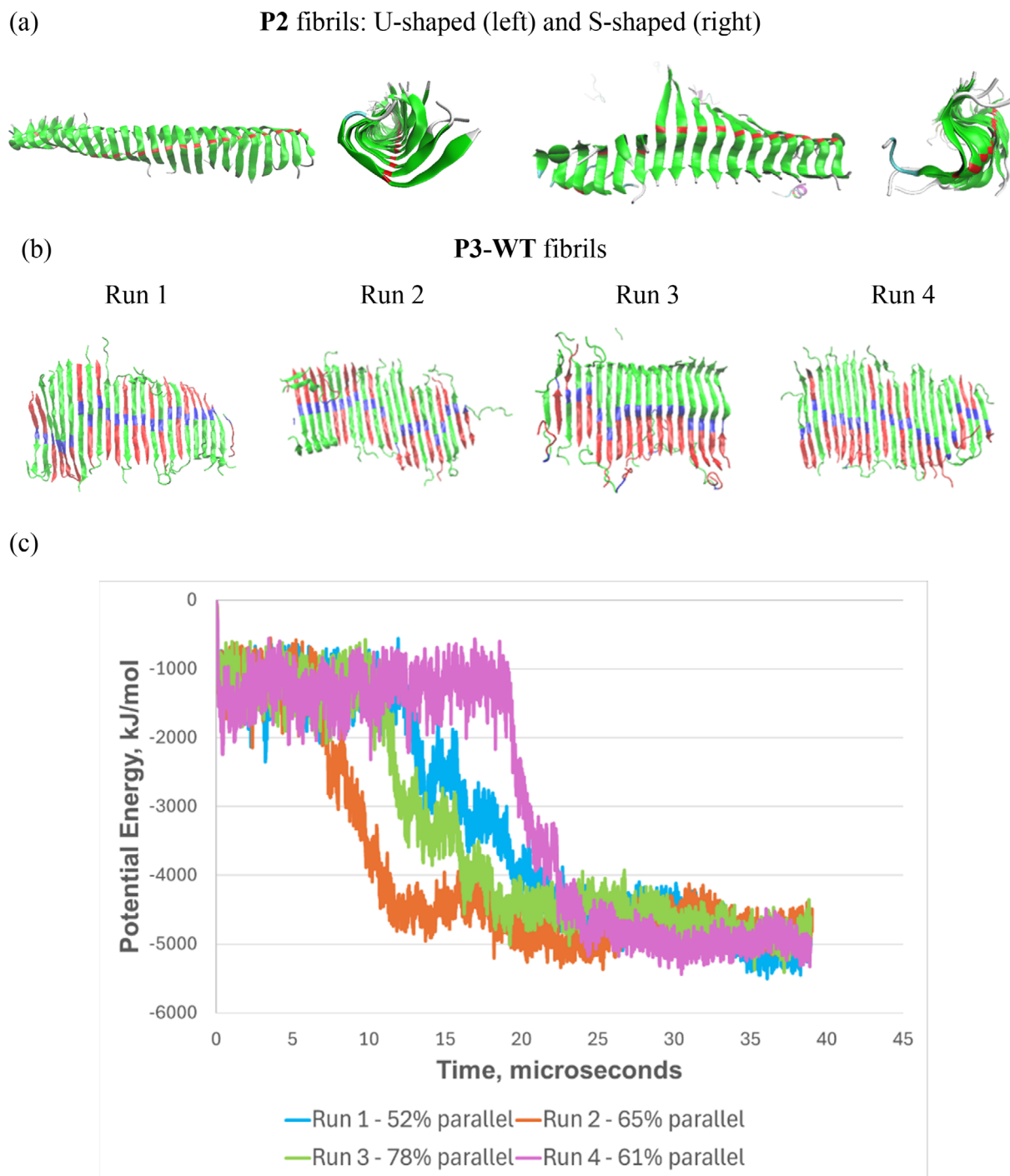
FIGURE 3 (a) Simulation snapshot of final conformation and schematic representation of U-shaped and S-shaped conformation of P2 fibrils. Red indicates G51 and green shows all other residues. (b) Simulation snapshots of P3 fragments at the end of each run show mixed fibrils with different percentage of parallel residues within the fibrils. As P3 contains both P1 and P2, the color code is used to display the position of P1 (red), P2 (green), and the in-between residues \alpha Syn [43, 44] (blue). (c) Total interaction energy vs. time for the four runs of P3-WT.
