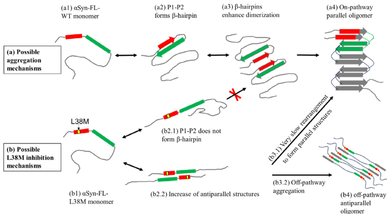
FIGURE 7 (a) A possible mechanism for \alpha Syn-FL-WT aggregation (Yu et al., 2015). (b) A possible mechanism for L38M inhibition of \alpha Syn-FL. L38M affects \alpha Syn-FL by reducing \beta -hairpin formation in P1/P2 region and by inducing antiparallel structures. The colored blocks indicate the regions that are simulated: P1 (red), P2 (green). The rest of the \alpha Syn-FL protein is gray.
