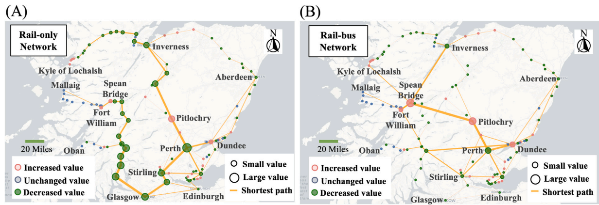
Fig. 6. Visualisation of betweenness centrality distribution in the (A) rail-only and (B) rail-bus network.
