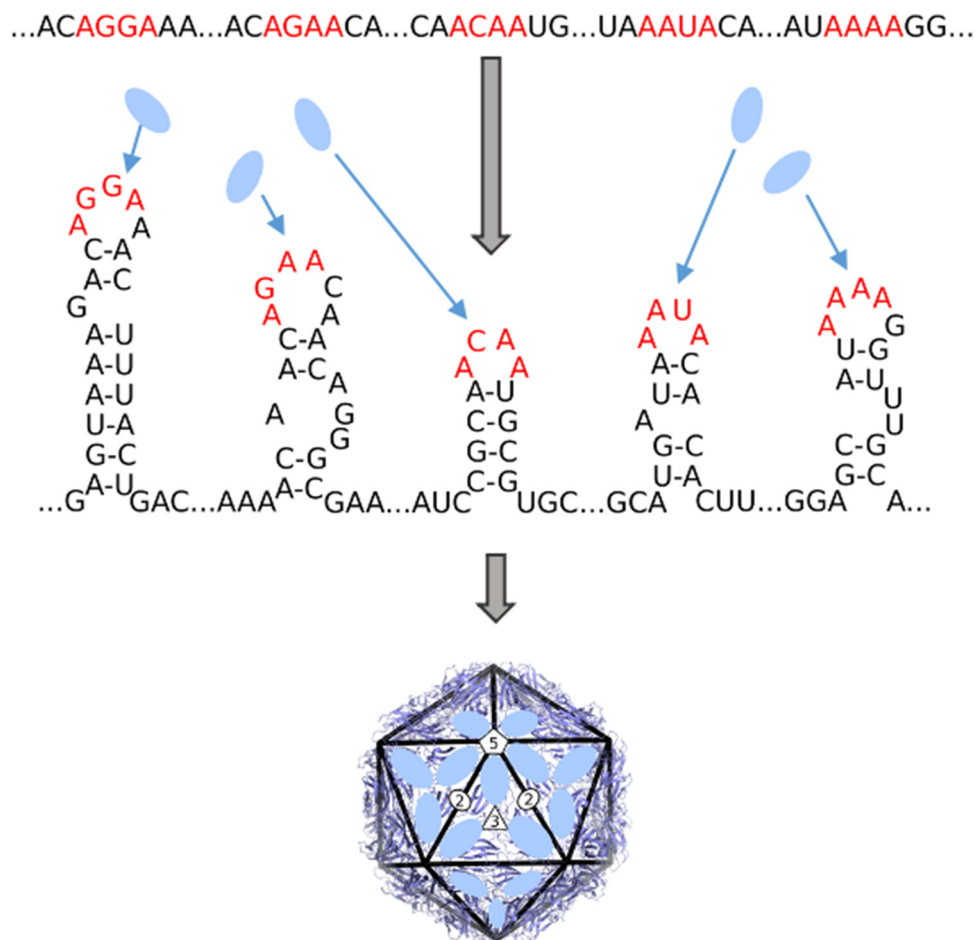
Figure 1. The packaging-signal-mediated assembly mechanism. Packaging-signal-mediated virus assembly [1] relies on multiple secondary structure elements ( packaging signals, PSs ) with a shared sequence motif (here AxxA, red) that is recognized by viral coat protein (CP, blue ovals). Individual stem-loops will drive sequence-specific assembly in vitro , whilst multiple sites, such as those at the 5' end of the Satellite Tobacco Necrosis Virus-1 gRNA shown, act cooperatively to promote assembly [3]. The cooperativity is sensitive to the folding propensity of the stem-loop, as well as the relative nucleotide separation of the stems.
