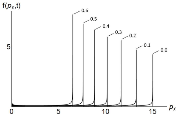
Fig. 6. Electron beam distribution function given by Eq. (56) versus time for p_{m,0} = 15 at s_2 t = 0.0, 0.1, 0.2, 0.3, 0.4, 0.5, 0.6 . The electron momentum is normalized on \Pi_2 .
