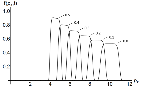
Fig. 4. Electron beam distribution function given by Eq. (49) versus time for m = 8 , p_{b,0} = 10 and \Delta p_0 = 1 at s_2 t = 0.0, 0.1, 0.2, 0.3, 0.4, 0.5 . The electron momentum is normalized on \Pi_2 .
