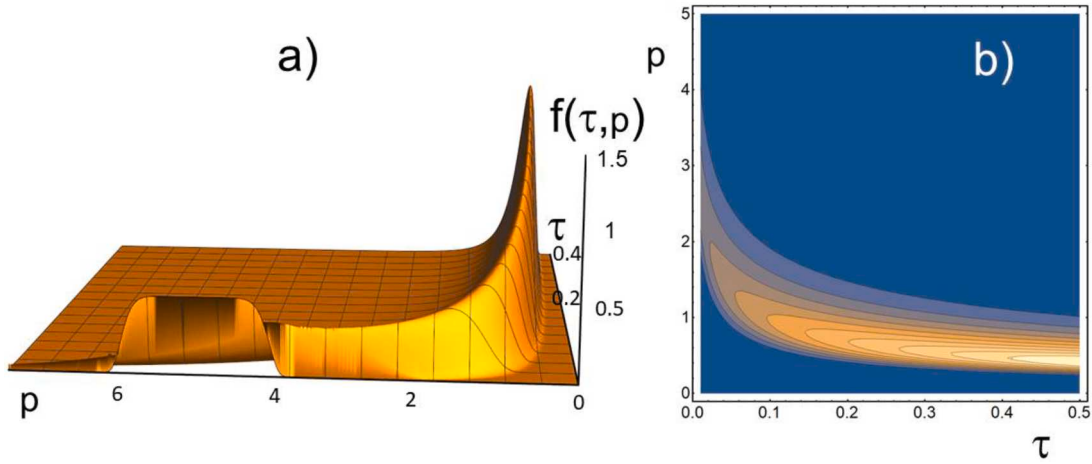
Fig. 7. Electron beam evolution for initial distribution function given by Eq. (44) with m = 8 , p_0 = 5 , \Delta p_0 = 1 ; a) function f(\tau, p) ; b) equal value contours of f(\tau, p) on the plane (\tau, p) . The electron momentum is normalized on \Pi given by Eq. (61).
