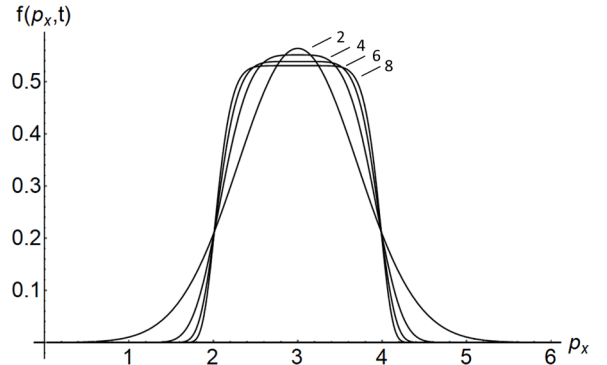
Fig. 1. Electron beam distribution functions (44) for m = 2, 4, 6, 8 and p_{b,0} = 3 , and \Delta p_0 = 1 . Here we use the momentum normalization to \Pi_1 given by Eq. (45).
