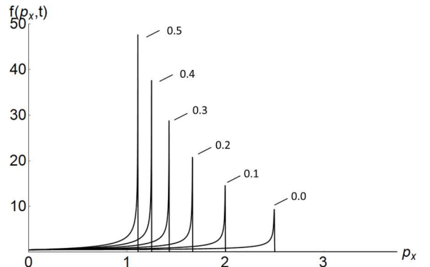
Fig. 5. Electron beam distribution function given by Eq. (54) versus time for p_{m,0} = 2.5 at s_1 t = 0.0, 0.1, 0.2, 0.3, 0.4, 0.5 . The electron momentum is normalized on \Pi_1 .
