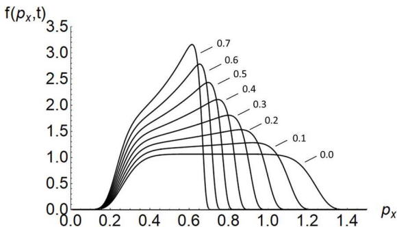
Fig. 3. Electron beam distribution functions (46) versus time for m = 8 , p_{b,0} = 0.75 and \Delta p_0 = 0.5 at s_1 t = 0.0, 0.1, 0.2, 0.3, 0.4, 0.5, 0.6, 0.7 . The electron momentum is normalized to \Pi_1 .
