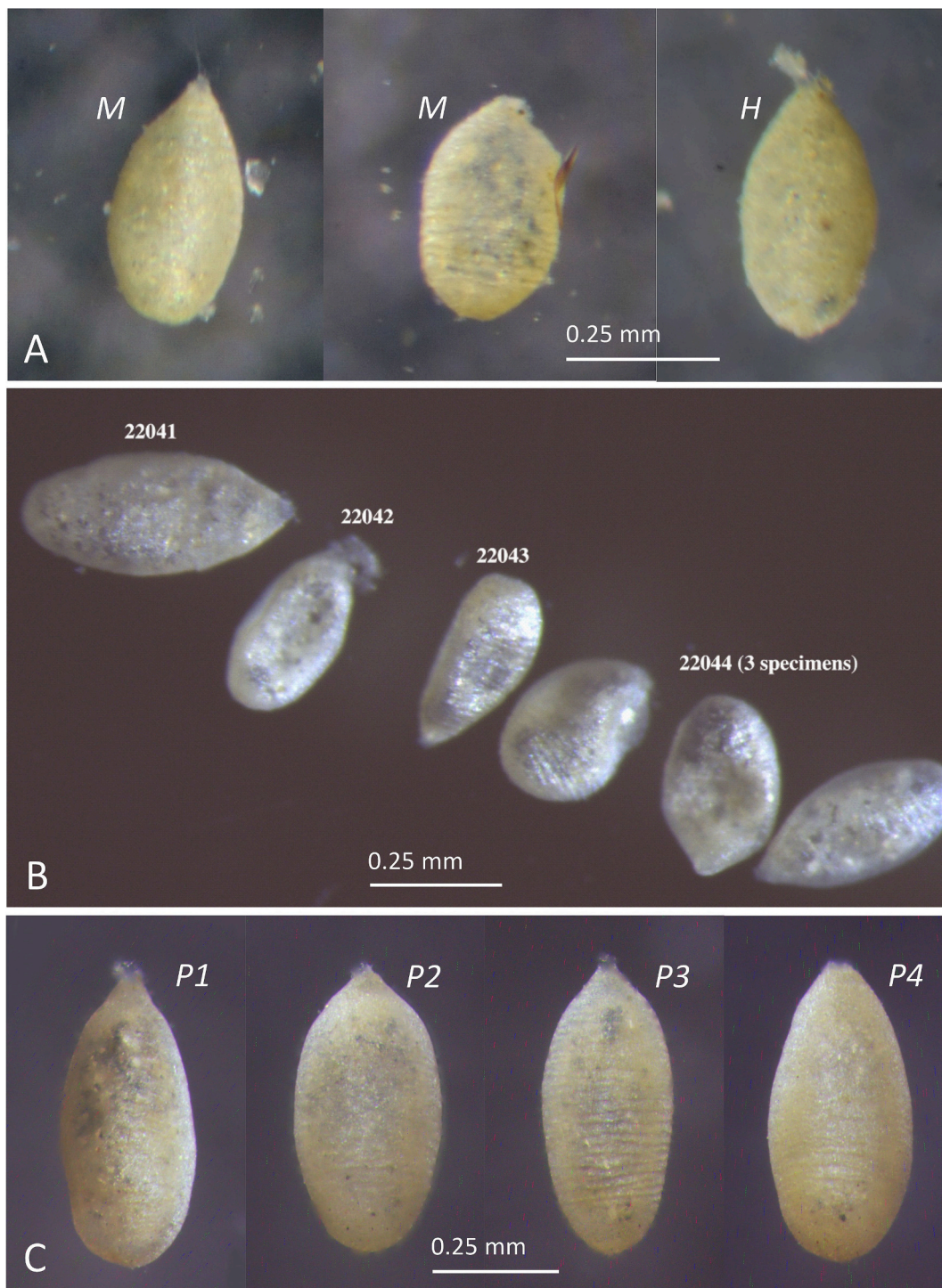
Fig. 6. Psammophaga owensi sp. nov. (A) Fresh specimens (M = destined for molecular determination; H = holotype). (B) Specimens for destined molecular determination in RNAlater™; their numbers correspond to subsequently extracted isolates. (C) Paratypes P1–P4 (fresh material).
