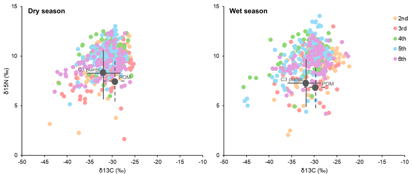
FIGURE 3 | Biplot of \delta^{13}\text{C} and \delta^{15}\text{N} values for consumer assemblages (fishes and aquatic macroinvertebrates) and two basal resource categories (C3 riparian and aquatic vegetation and POM) from each site along the continuum of the Tintinda River for dry ( n=471 consumer tissue samples) and wet seasons ( n=452 consumer tissue samples). Different colours represent Strahler order of the sites along the river continuum. There was one site representing each Strahler order. Values for consumers were adjusted for trophic fractionation.
