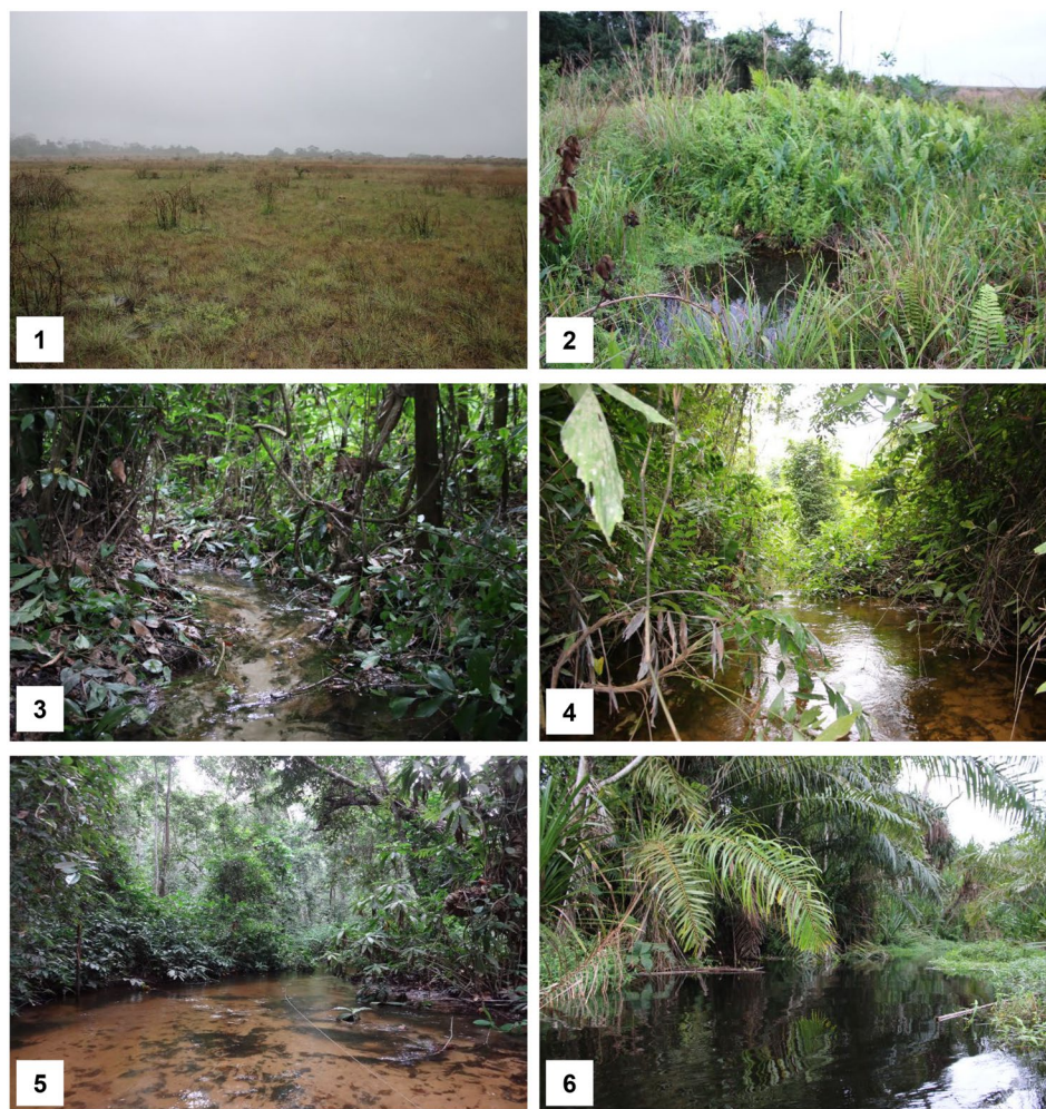
FIGURE 2 | Photographs of sites on the Tintinda River from second (2) to sixth (6) Strahler order along the fluvial gradient. First-order sites (1) situated in the grassland-savannah vegetation zones of the Tintinda River were dry in both seasons.
