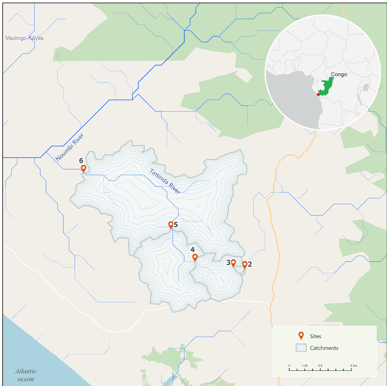
FIGURE 1 | Study area showing study sites (numbers reflect Strahler order, from second to sixth) along the continuum of the Tintinda River in the Republic of the Congo.
